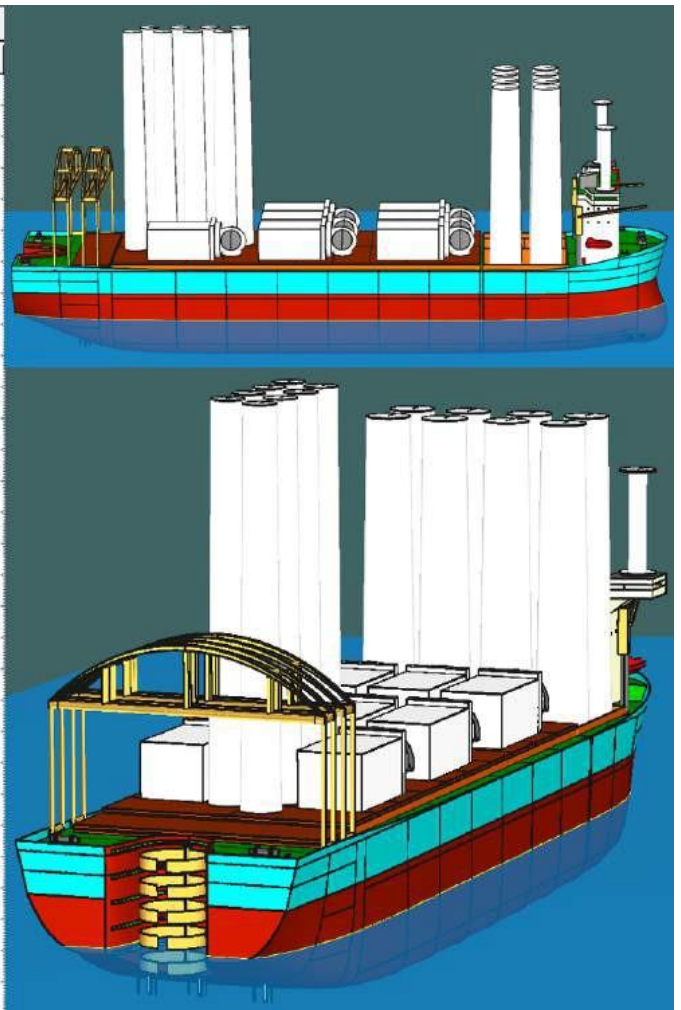
Figure 7-22 Equilibrium Status at Departure Condition While Loading 8x12MW WT
