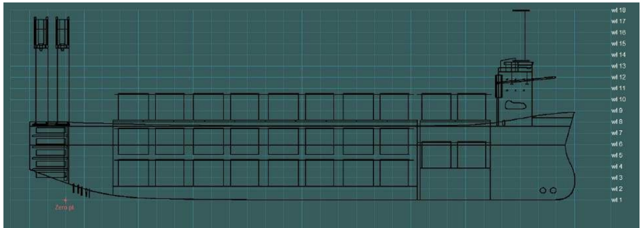
Figure 6-108 TPs loading arrangement (Side View)
