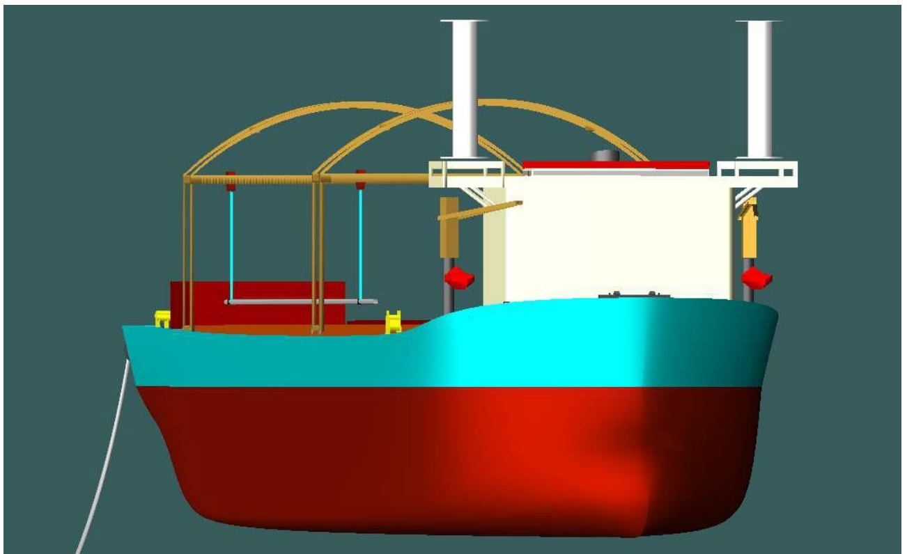
Figure 6-234 The cable is cut and lifted to be loaded on top of the hatch cover
