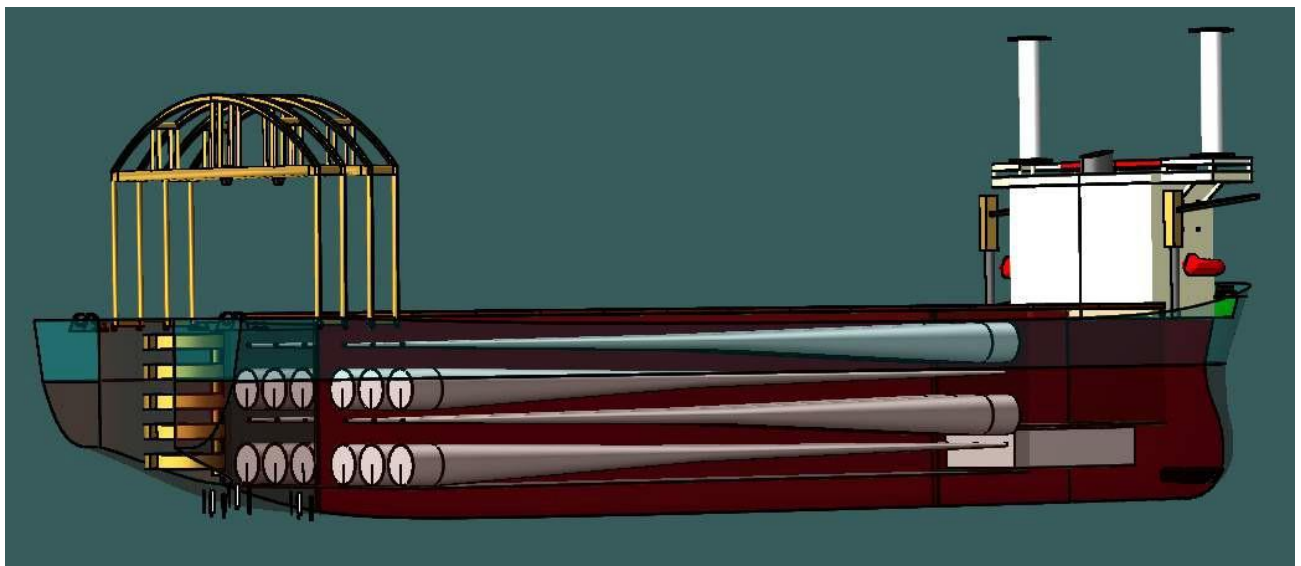
Figure 6-21 Perspective View of Load out of 12 MW Blades inside the holds
