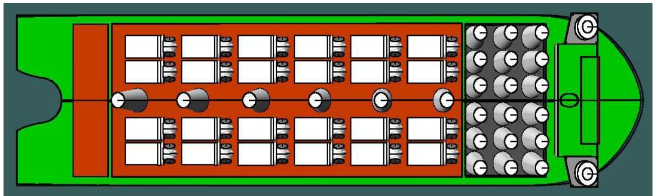
Figure 6-38 Top View of Load out of 5MW Wind Turbine
