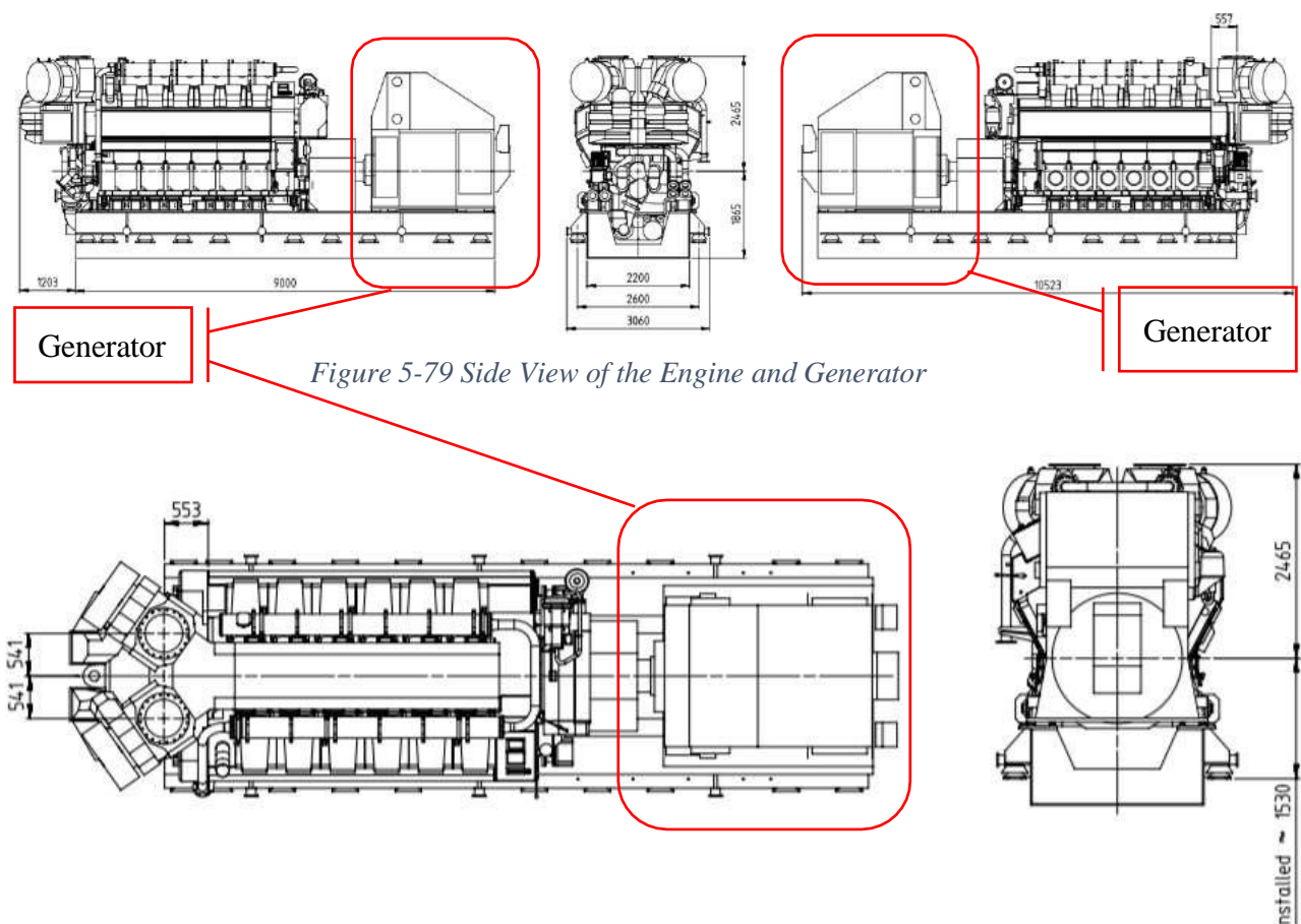
Figure 5-80 Plan of The Engine and Generator
