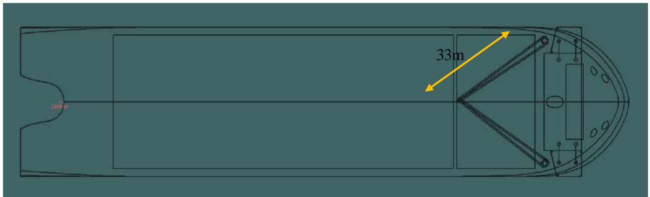
Figure 5-47 Boom Length of Provision Cranes
