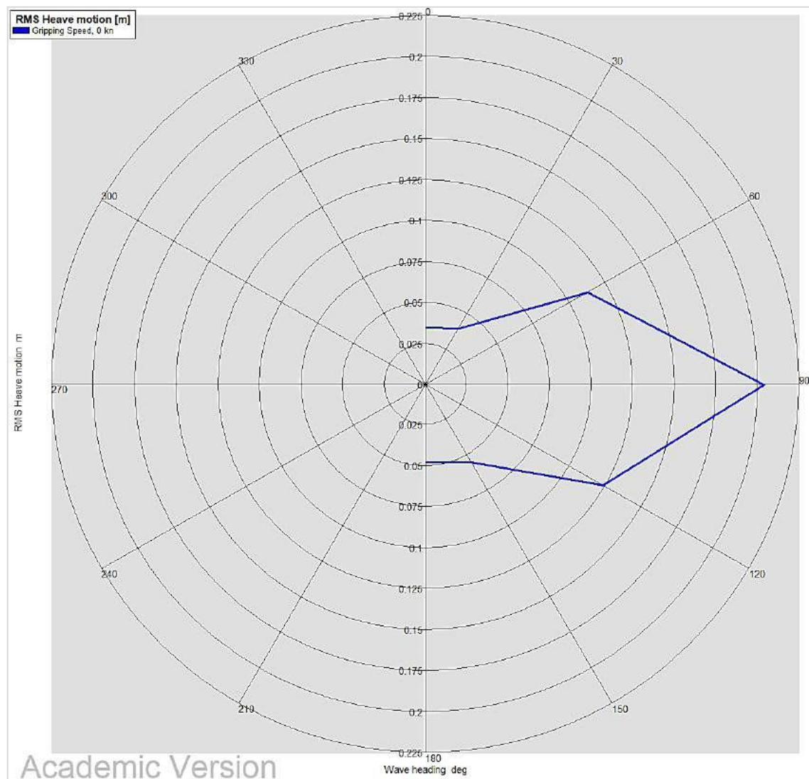
Figure 8-5 Heave Motion at COG – Slight Sea state
