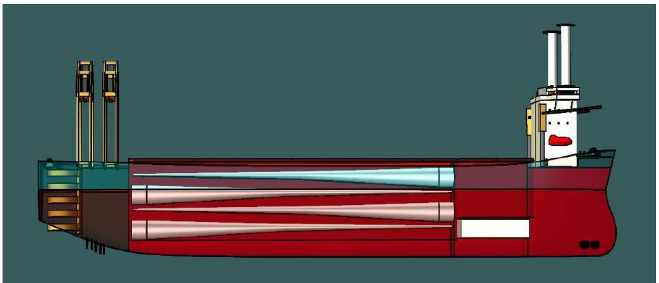
Figure 6-24 Side view of Load out of 12 MW Blades inside the holds
