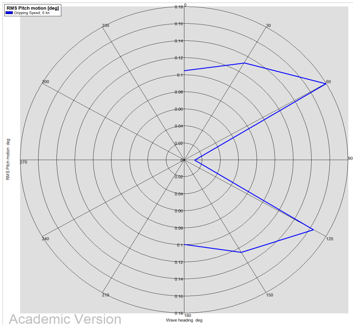
Figure 8-7 Pitch Motion at COG – Slight Sea state
