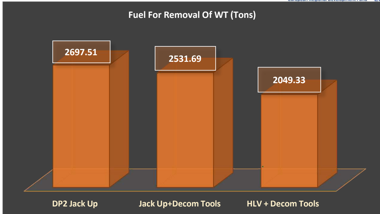
Figure 3-45 Fuel Consumption of Various Logistic configuration for Decommissioning of Hornsea1 OWP
