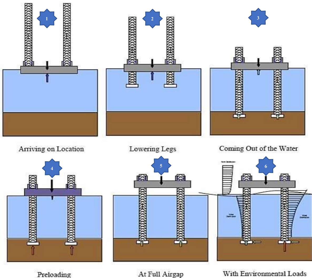
Figure 3-5 Transition Modes of a Jack up Vessel
