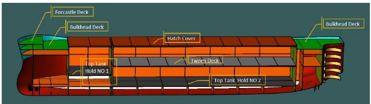
Figure 5-10 Decom Tools Vessels Decks
