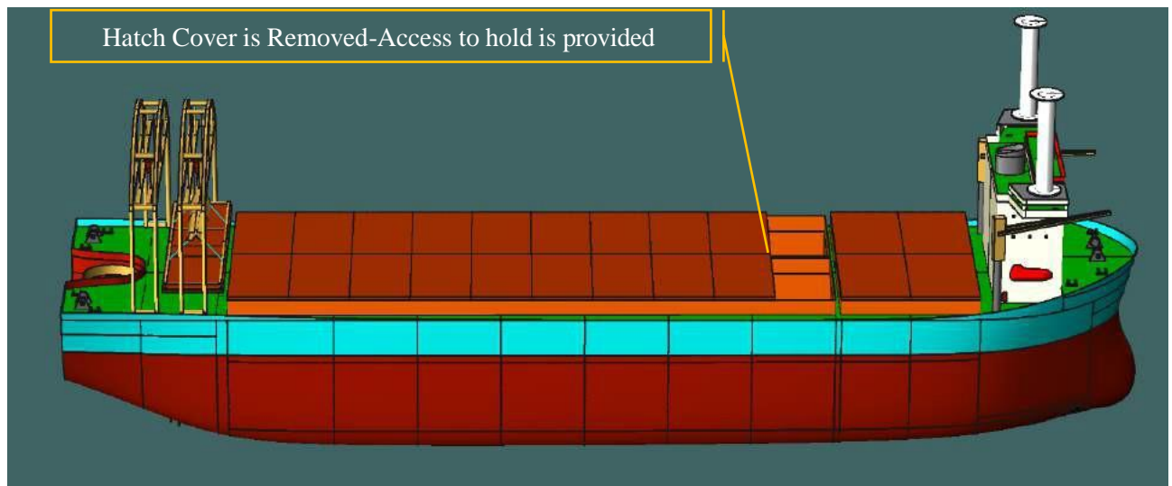
Figure 5-96 Procedure to open the Hatch Cover-Step 4 Access Provided to the Hold
