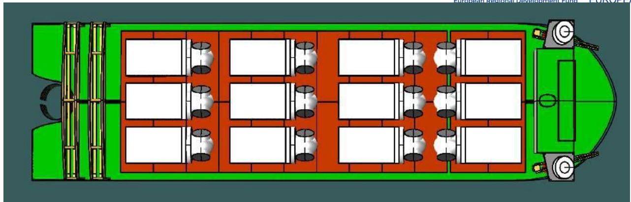
Figure 6-52 Top View of Load of 12MW Nacelle with Decom Tools Vessel
