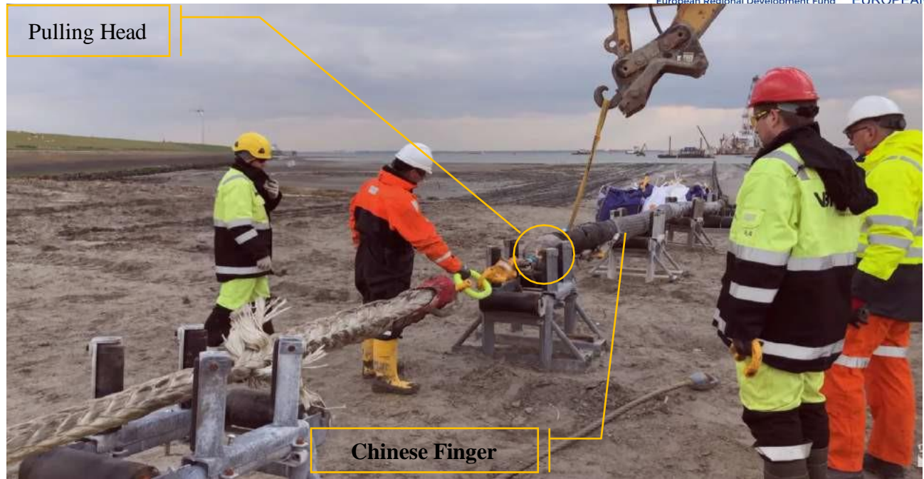
Figure 6-200 Pulling the Cable with onshore winch via both Pulling head and Chinese finger (Boskalis 2019)
