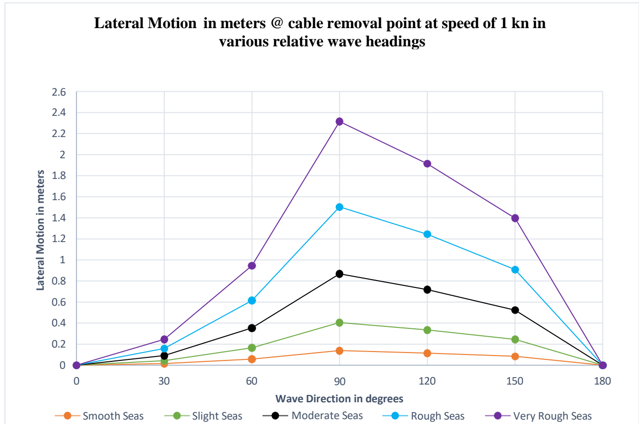
Figure 8-18 Comparison of lateral movement during cable removal operation in various sea state
