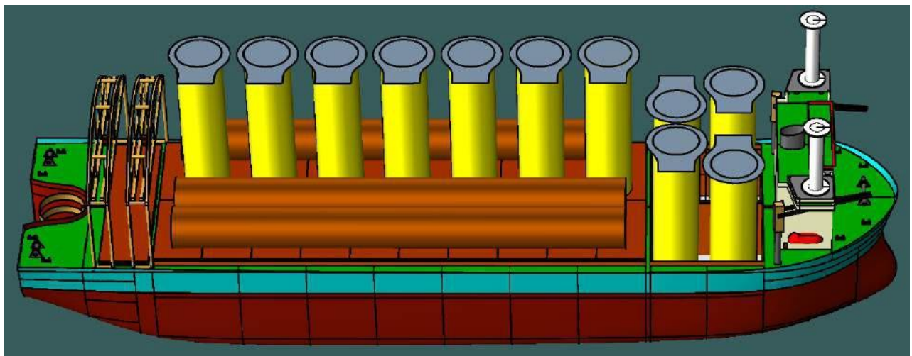
Figure 6-31 Top view of Load out of 12MW TP & Monopile (First Arrangement)
