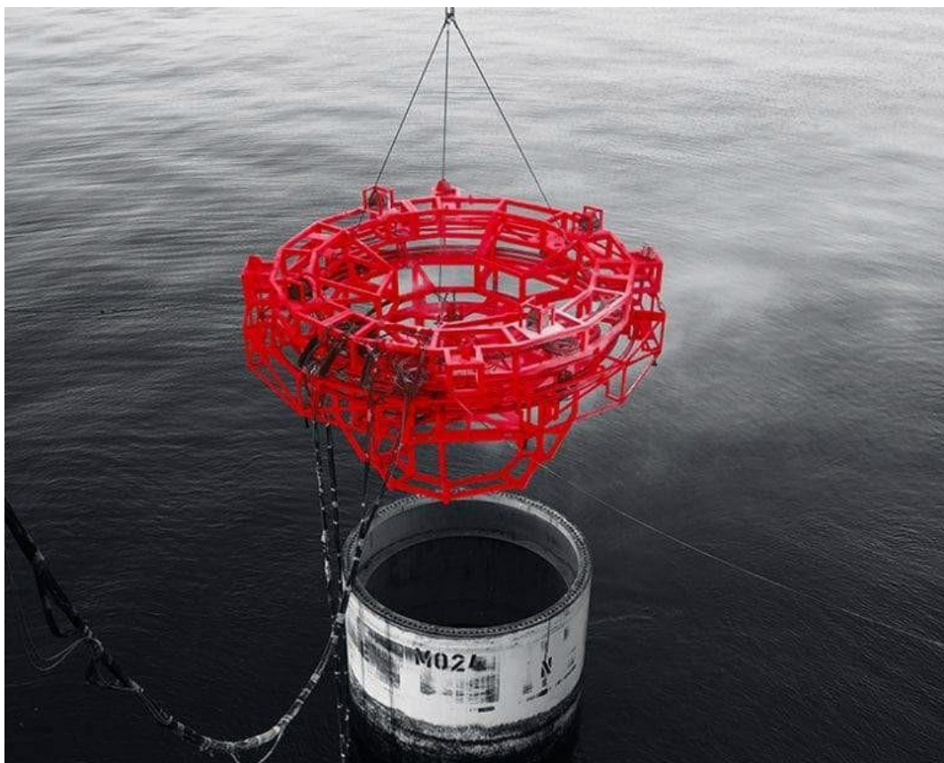
Figure 6-156 Marine Growth Removal Tool (CLAXTON n.d.)
