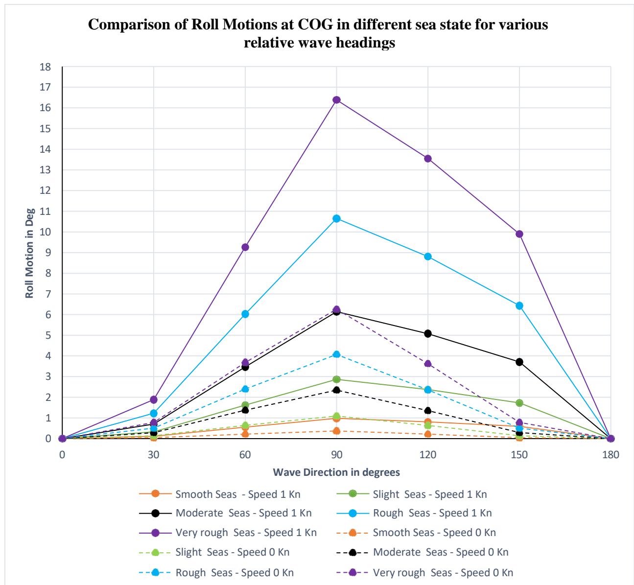
Figure 8-10 Comparison of Roll Motions at COG in different sea state
