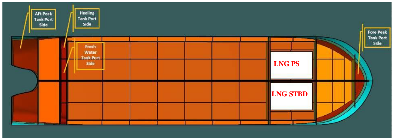
Figure 5-23 Top View of Decom Tools Vessel's Tanks
