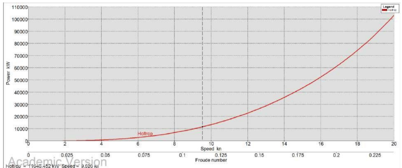
Figure 5-65 Correlation Between Speed and Power at Draft of 19.79 meters
