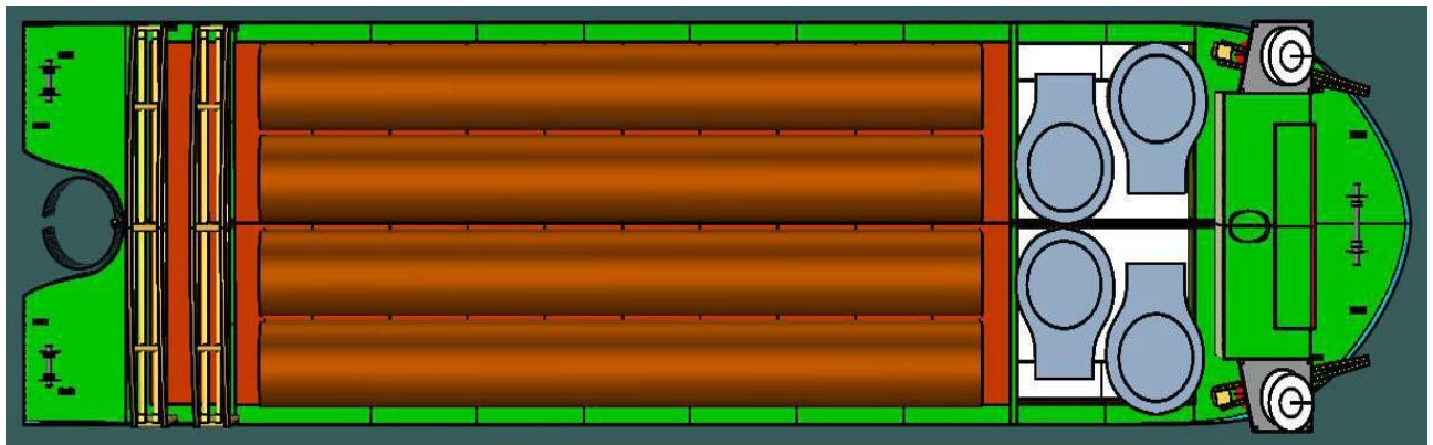
Figure 6-34 Top View of Load out of TP and Monopile (Second Arrangement)
