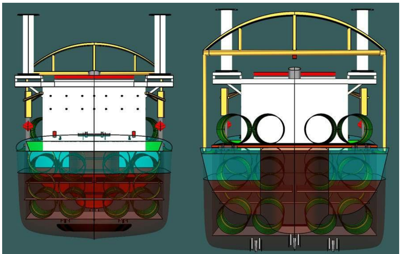
Figure 6-165 Load out of 24 Numbers of MP plus TP (Bow View)
