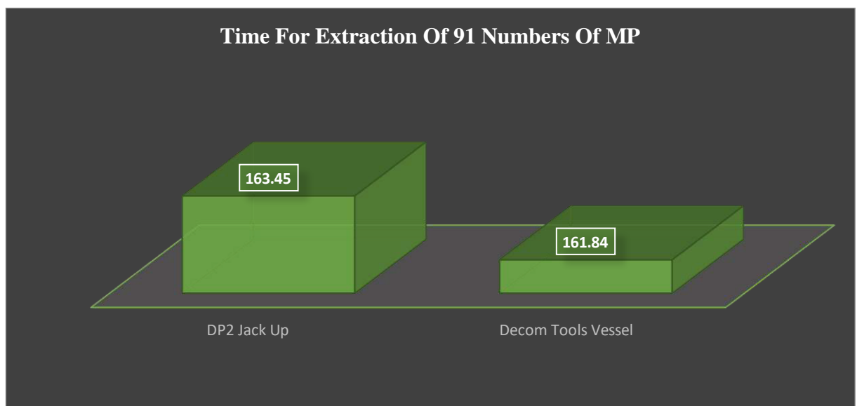
Figure 6-172 Comparison of Duration for MP Extraction
