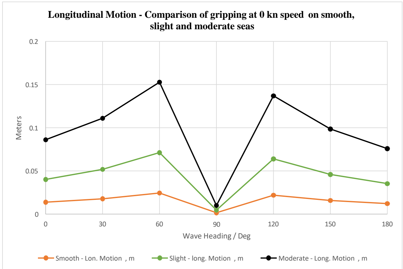
Figure 8-12 Longitudinal Motion at Gripper point on three different Sea States
