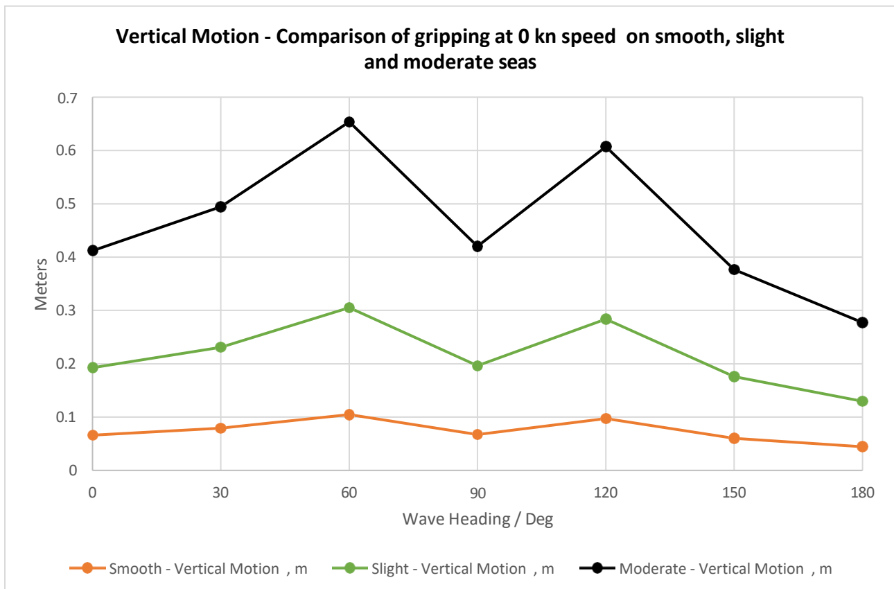
Figure 8-11 Absolute Vertical Motion at Gripper point on three different Sea States
