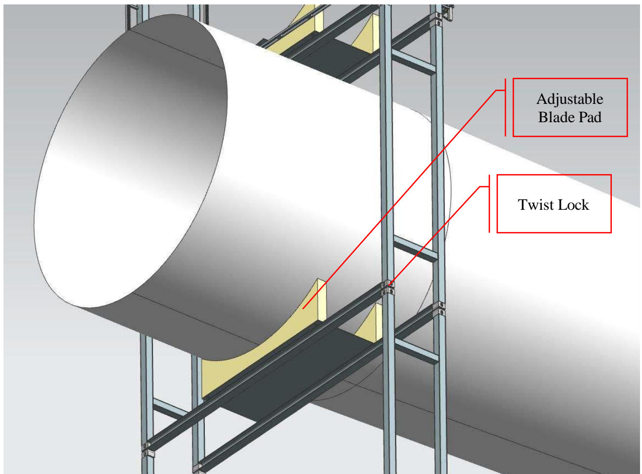
Figure 6-64 Blade Pad and Twist Lock
