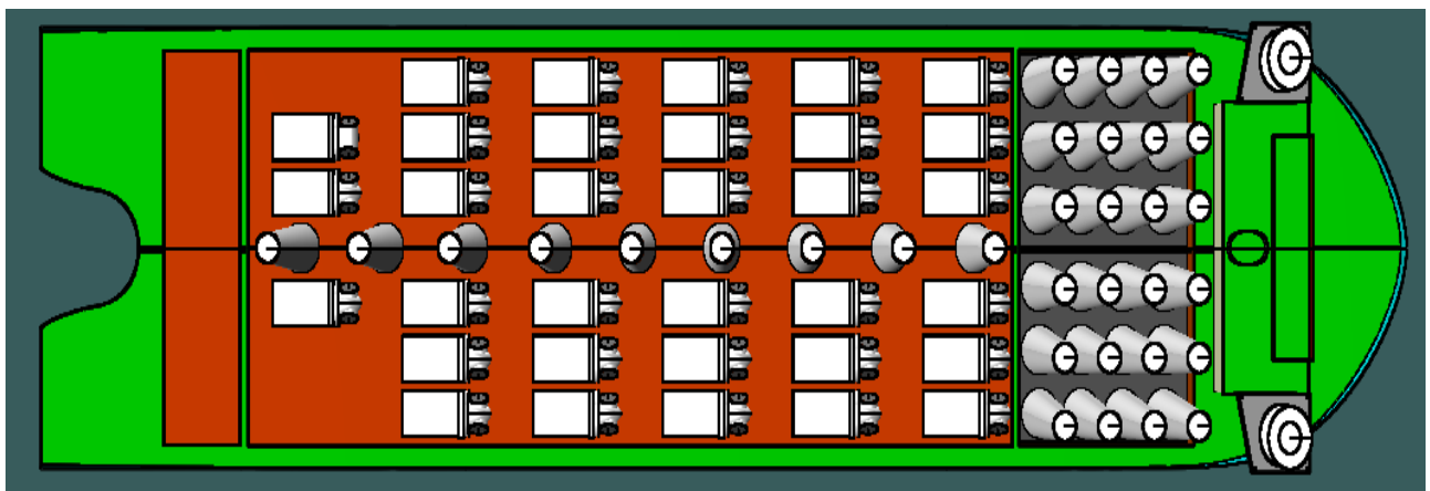
Figure 6-41 Top View of Load out of 3.6 MW Wind Turbine
