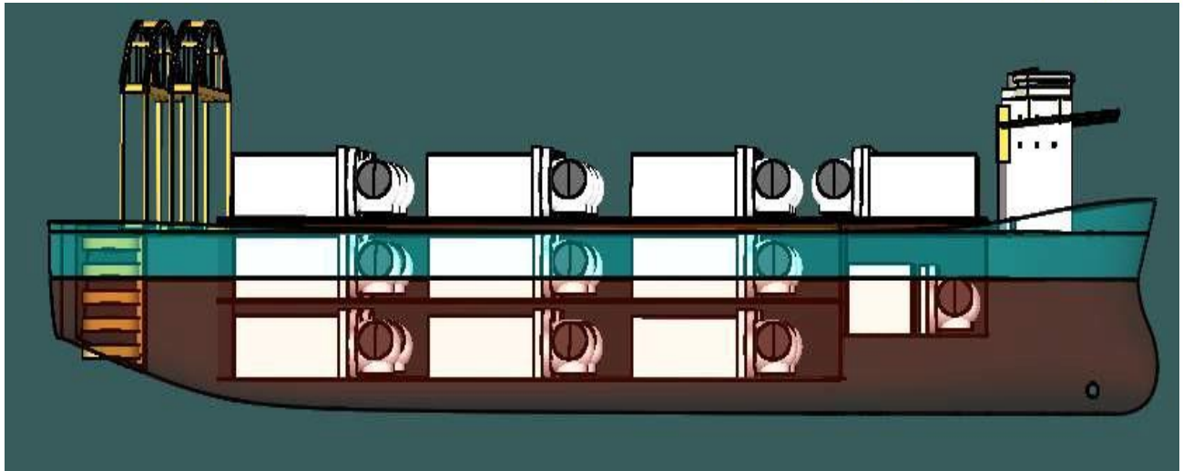
Figure 7-31 Lod out of 26 Number of 12 MW Nacelle
