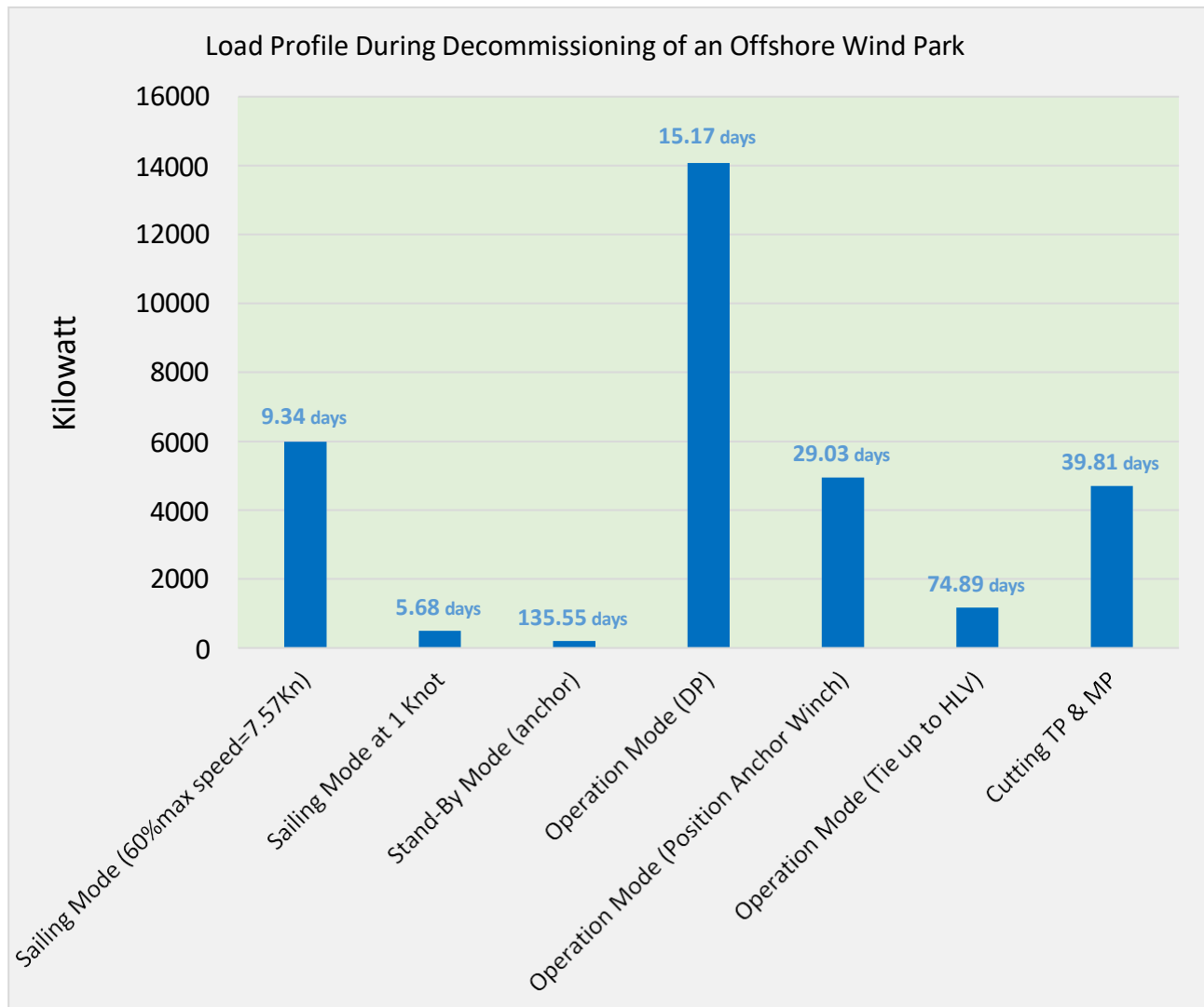
Figure 5-78 Load Profile During Decommissioning of an Offshore Wind Park
