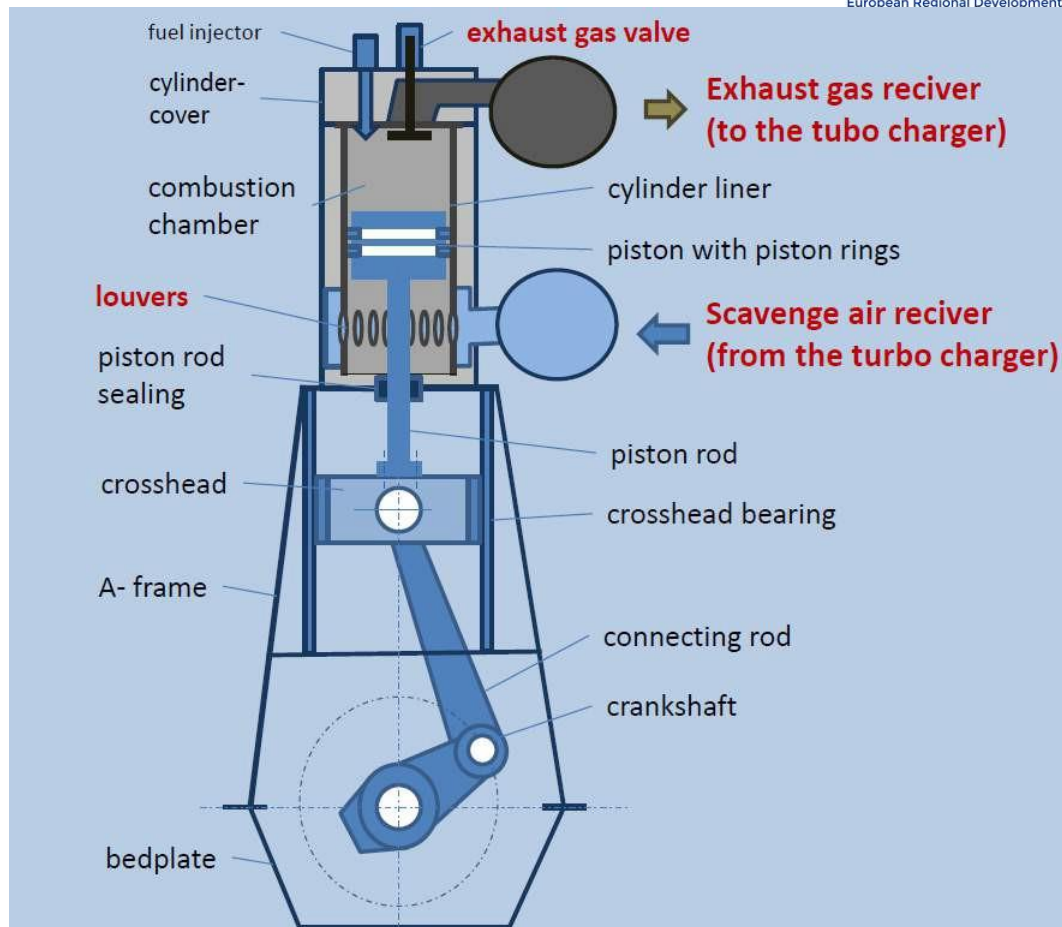
Figure 4-5 Cross Section of 2-Stroke Crosshead Engine
