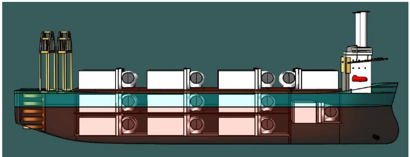
Figure 6-53 Side View of Load of 12MW Nacelle with Decom Tools Vessel
