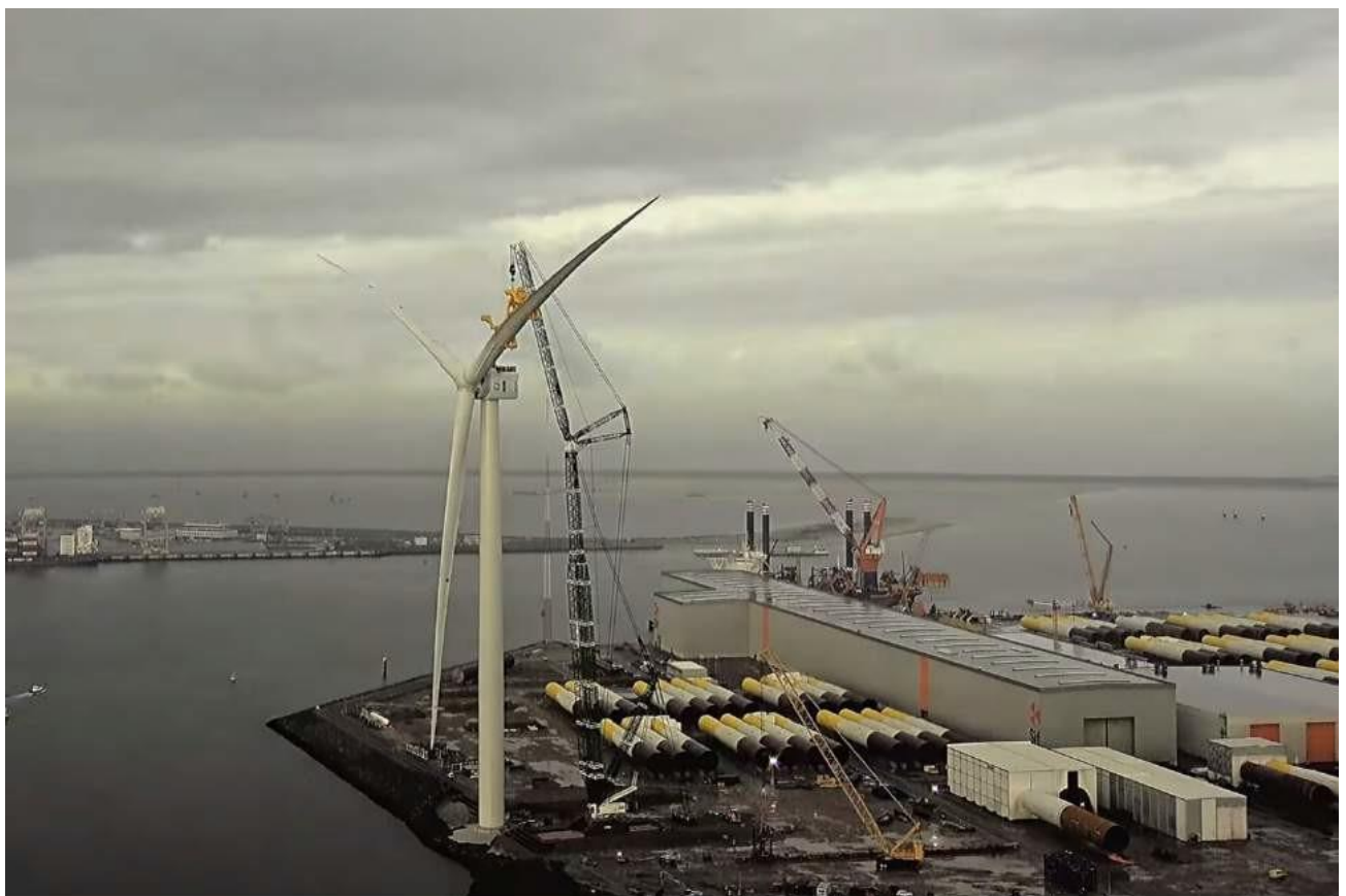
Figure 6-19 Installation of Third Blade of 12 MW GE X-Heliade Nacelle in the Rotterdam Port (GE Renewable Energy 2019)
