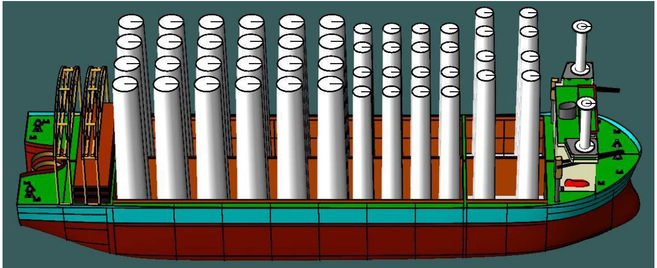
Figure 6-49 Top View of Load of 12MW Tower with Decom Tools Vessel
