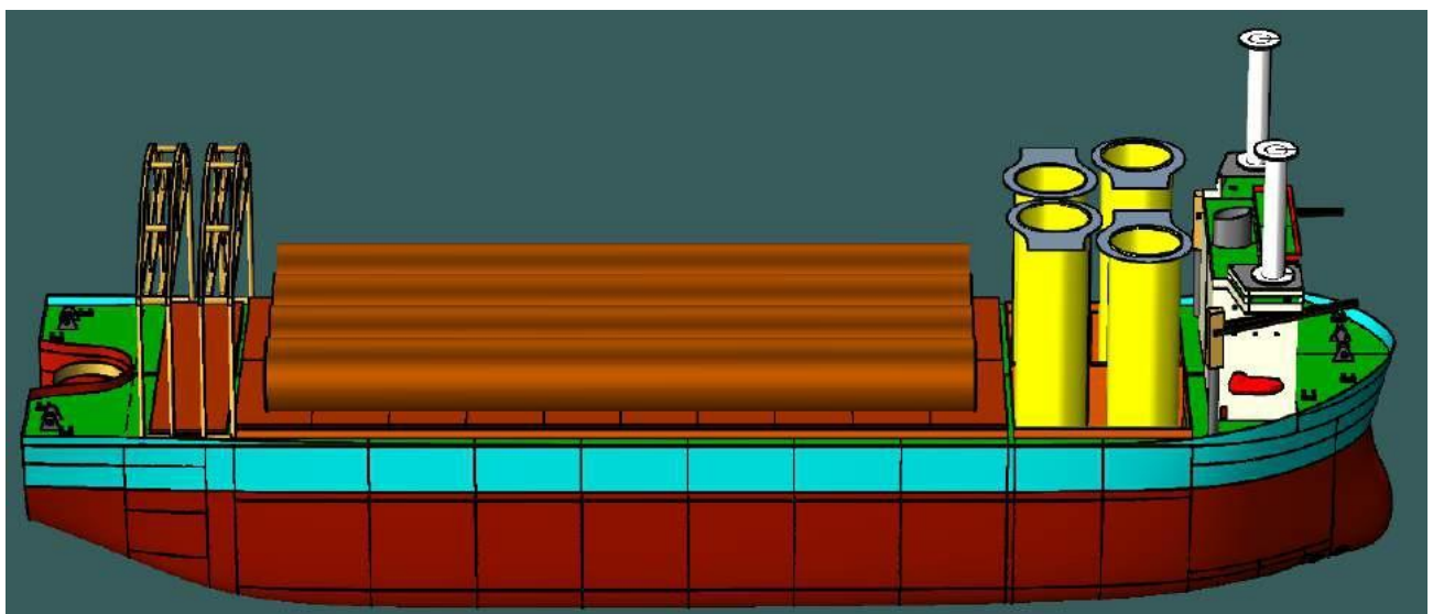
Figure 6-35 Side View of Load out of TP and Monopile (Second Arrangement)
