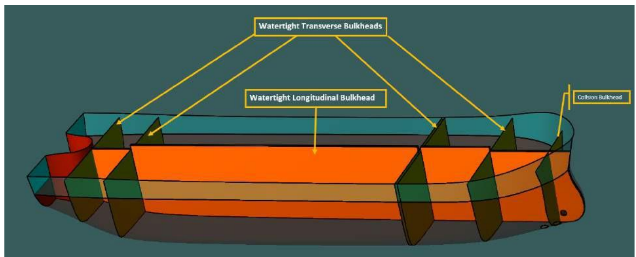
Figure 7-7 Watertight Hull and Subdivision of Decom Tools Vessel
