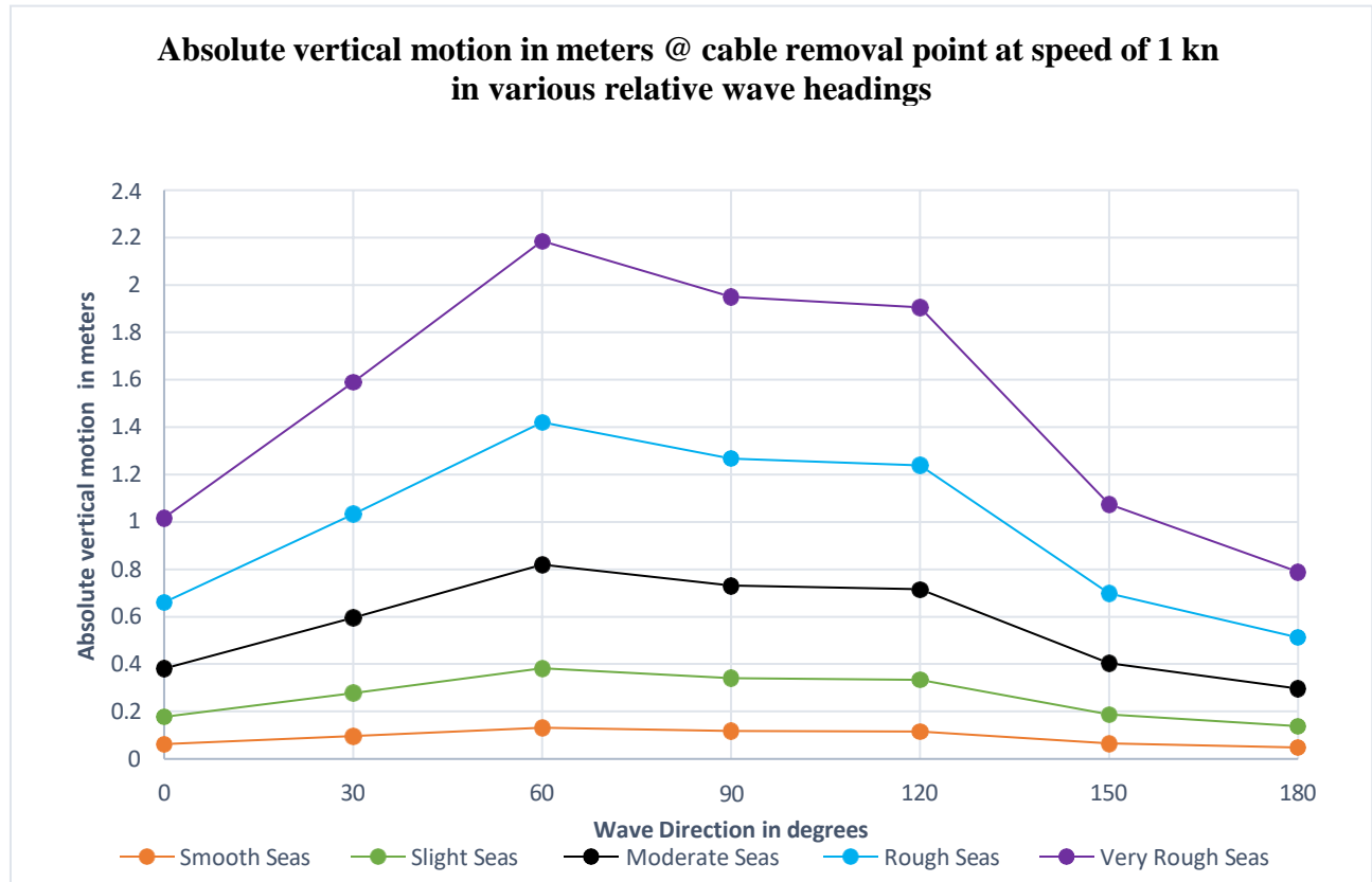
Figure 8-16 Comparison of absolute vertical motion during cable removal operation in various sea state
