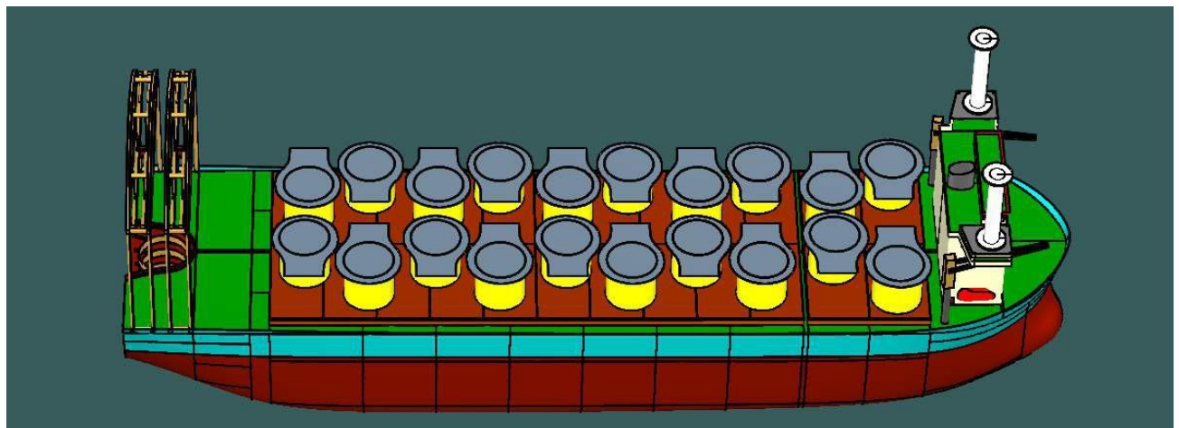
Figure 6-109 TPs loading arrangement (Bird's Eye View)
