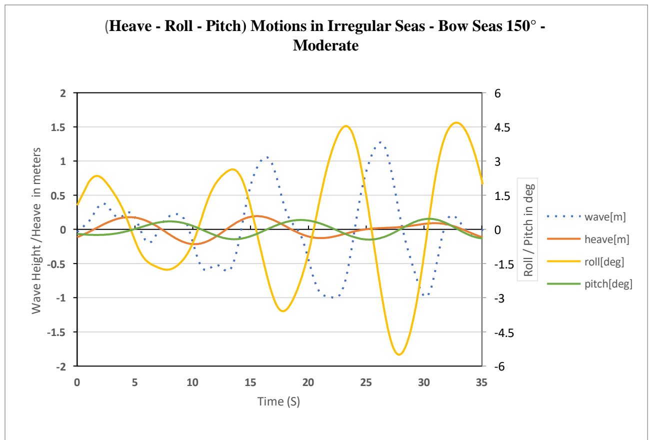
Figure 8-20 Motion in irregular bow seas 150° – Moderate
