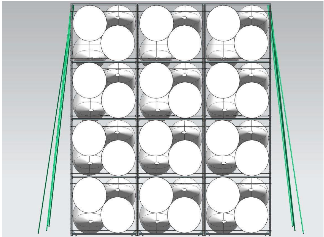
Figure 6-83 3.6 MW blades inside the racks (front View)
