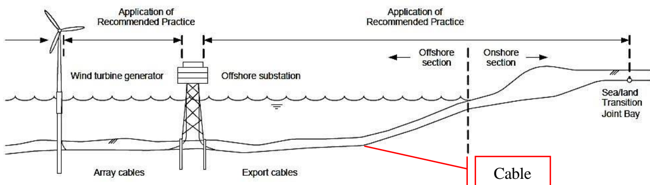
Figure 6-177 Transmission of Generated Power by OWT to Shore (DNV.GL 2016)
