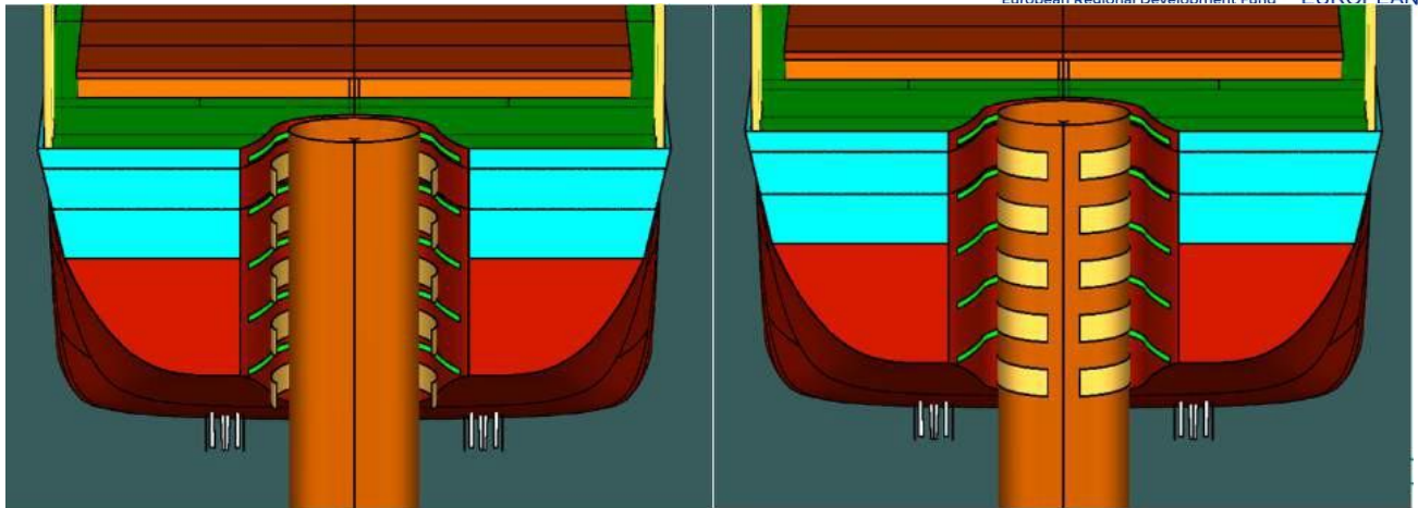
Figure 6-134 Status of Pile Grippes
