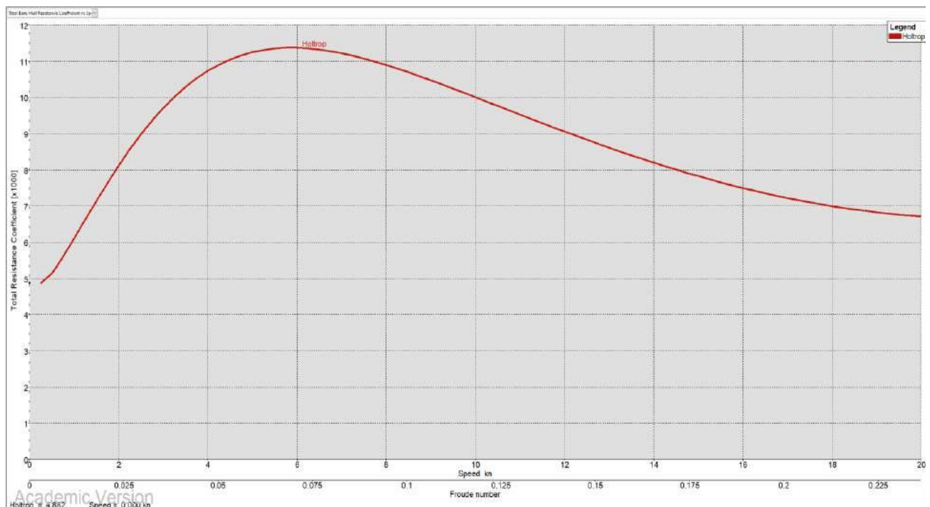
Figure 4-9 Decom Tools Resistance Coefficient
