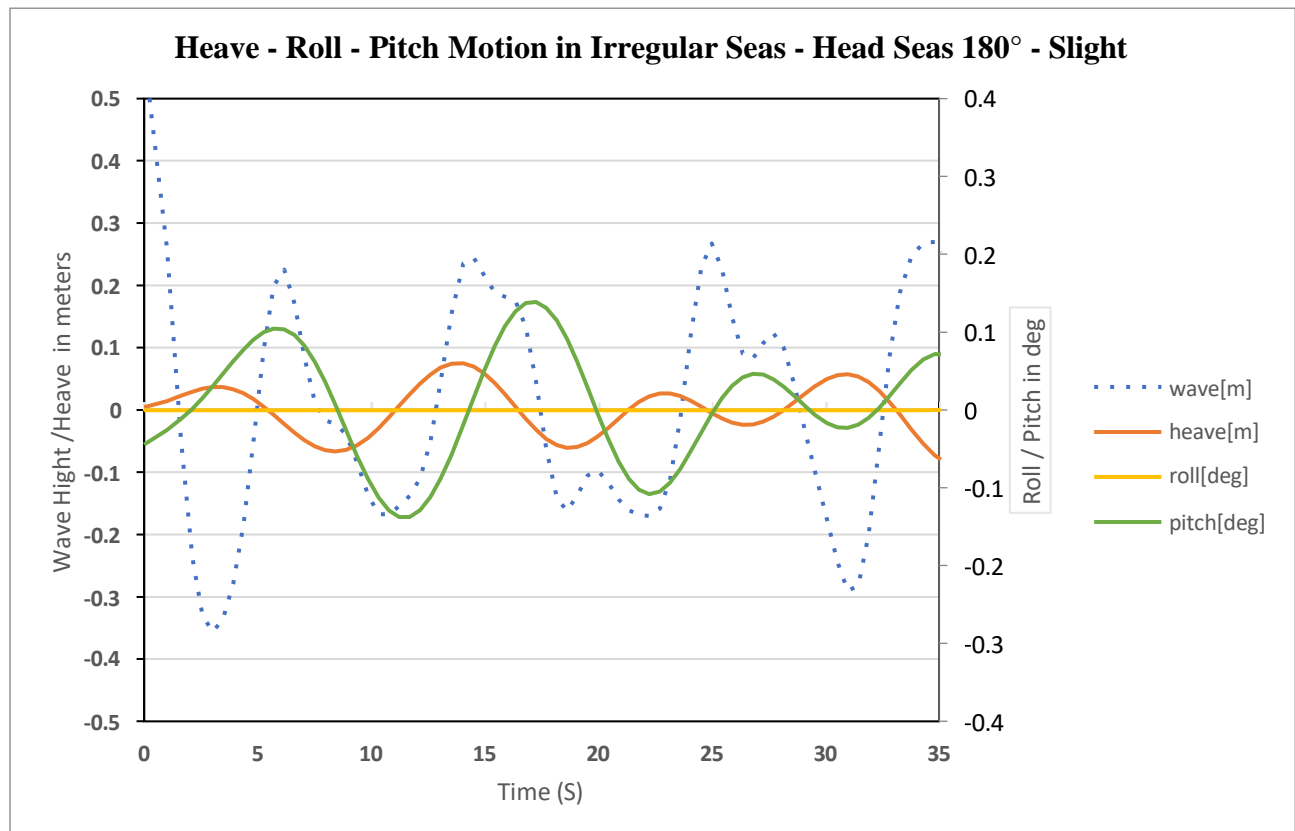
Figure 8-14 Motion in irregular head seas – Slight Seas
