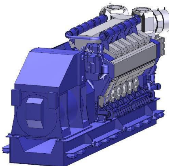
Figure 5-82 Perspective View of Wärtsilä 12L34DF
