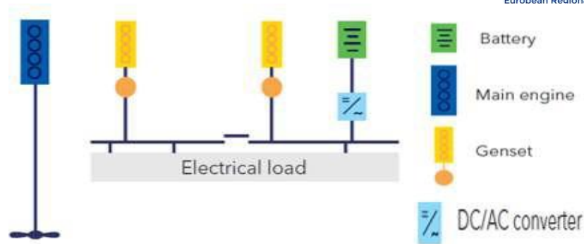
Figure 4-31 Mechanical Propulsion with Battery Hybrid Electrical Power Plant
