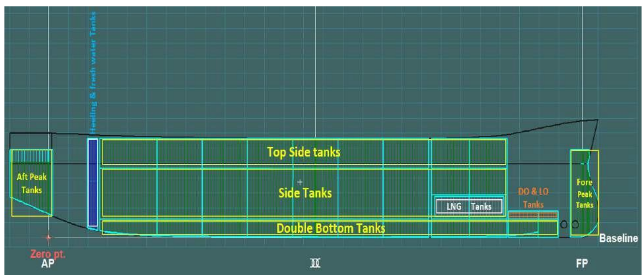
Figure 7-9 Plan of Tanks of Decom Tools Vessel
