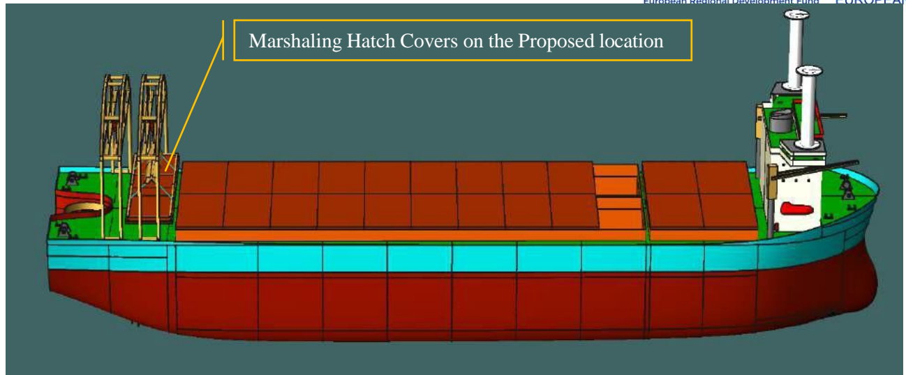
Figure 5-95 Procedure to open the Hatch Cover-Step 3 Placing Hatch Cover on the Proposed Location
