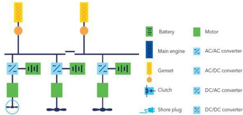
Figure 4-33 Hybrid Battery Propulsion, with Distributed Batteries
