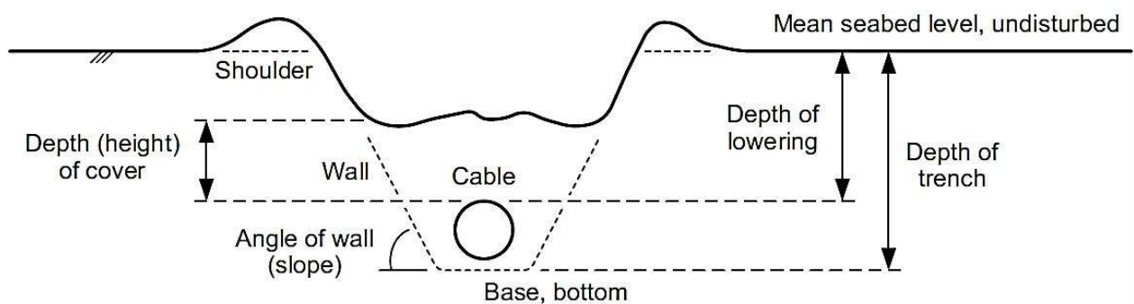
Figure 6-178 Burial of Submarine Cables (DNV.GL 2016)
