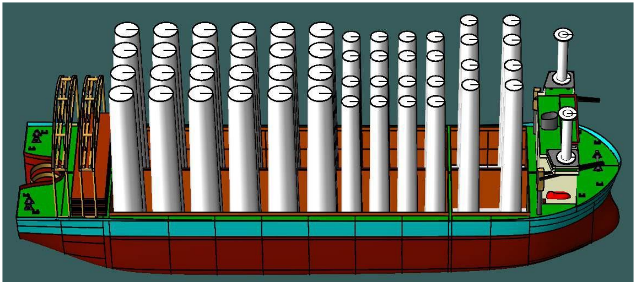
Figure 7-29 Load out of 24 Numbers of 12 MW WT Tower
