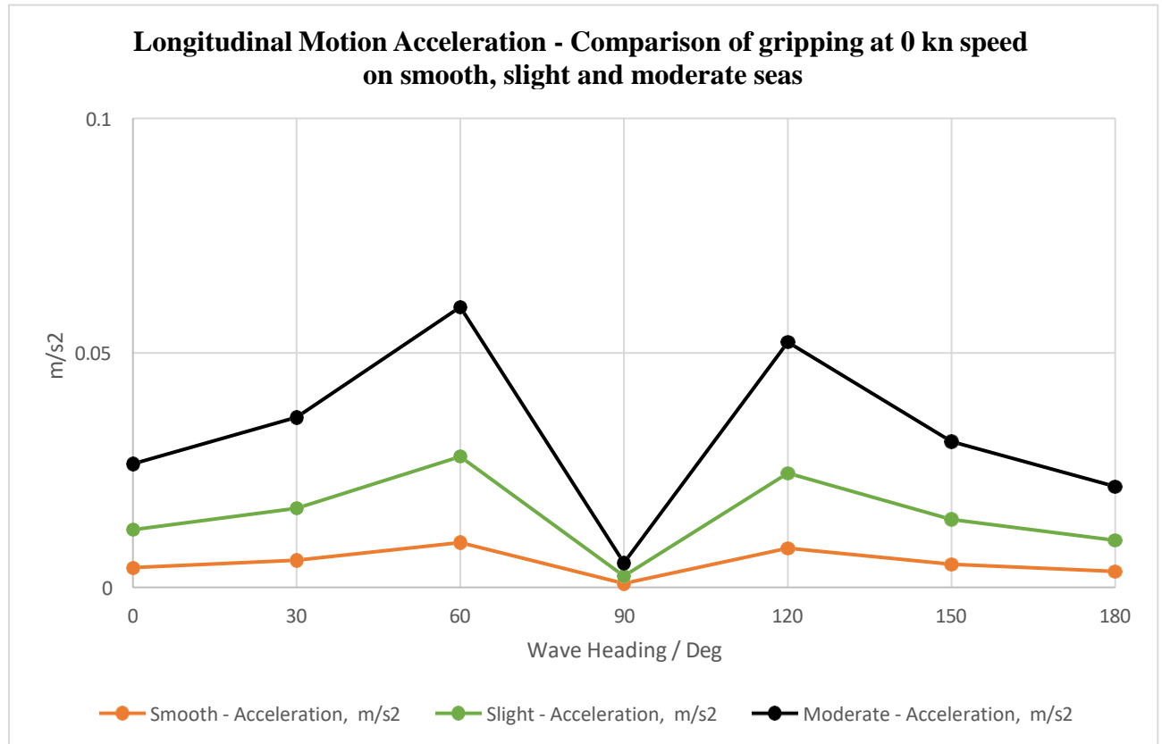
Figure 8-27 Longitudinal Motion Acceleration at Gripper point on three different Sea States
