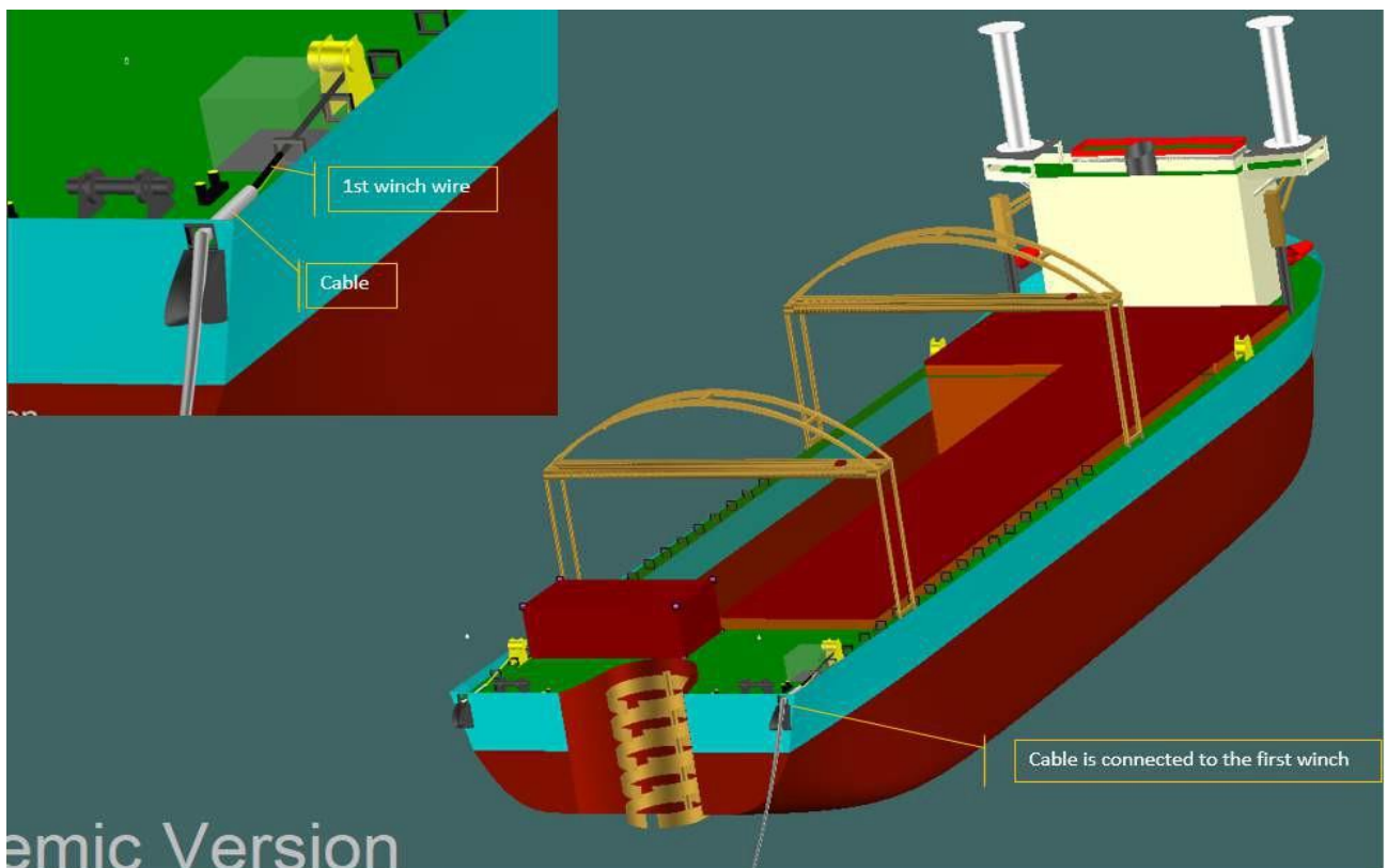
Figure 6-227 Cabled is pulled by first winch onto the deck
