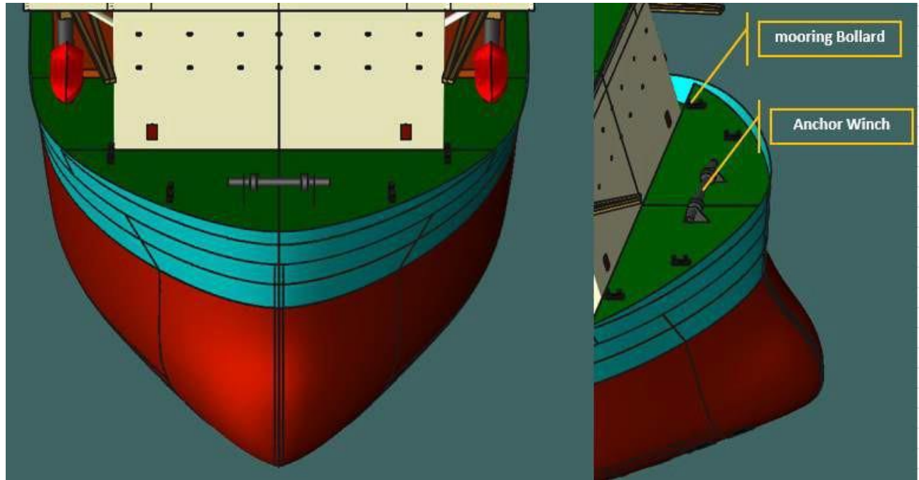
Figure 5-88 Details of Bow of the Decom Tools Vessel
