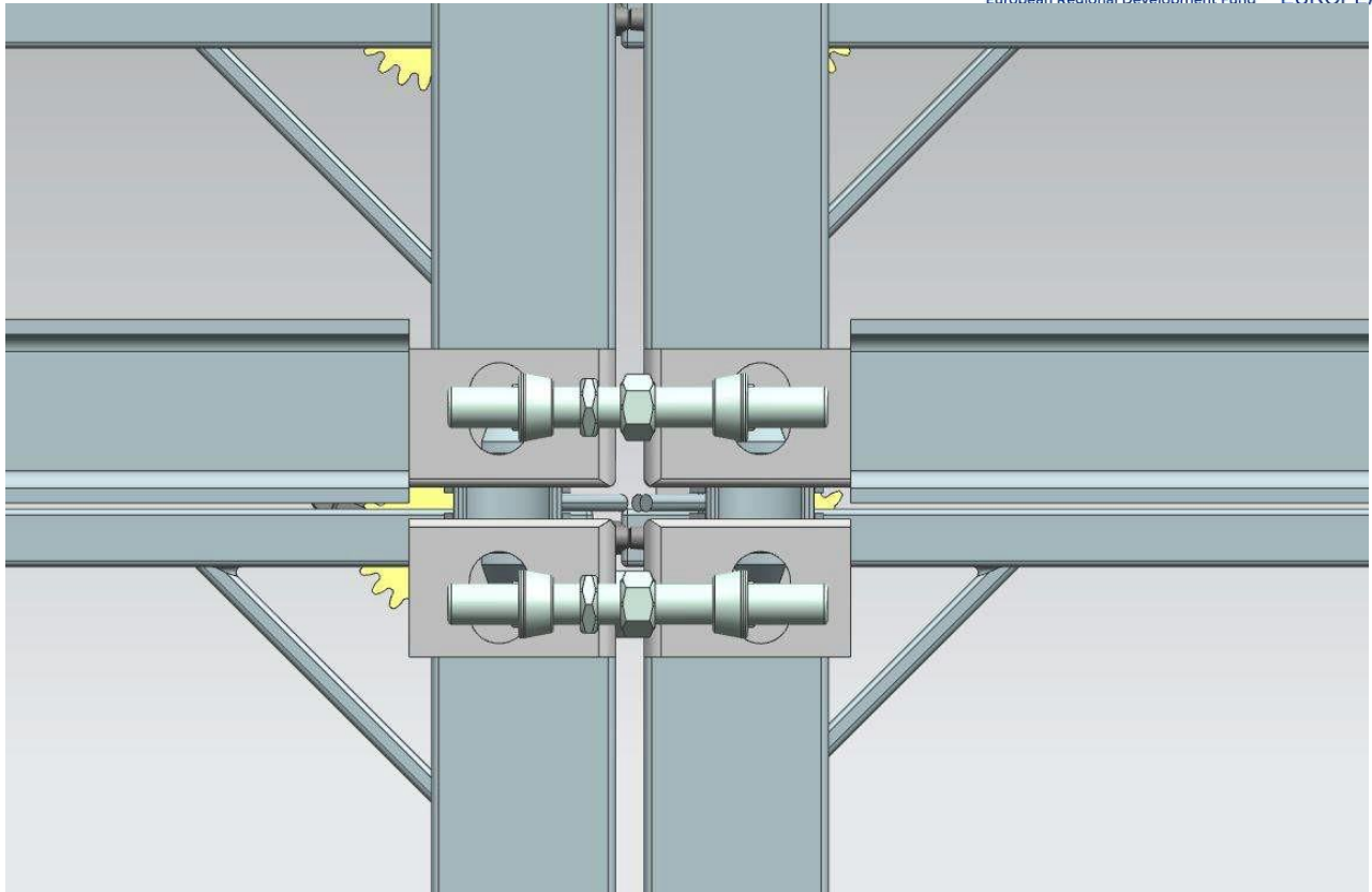
Figure 6-66 Connection of Blades Rack
