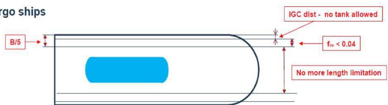
Figure 5-30 Location of LNG tank based on IGF code (Kokarakis 2015)
