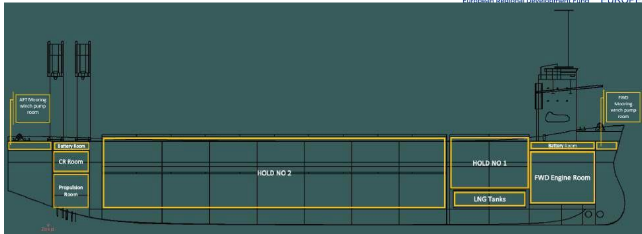
Figure 5-83 Engine room, Propulsion Room and Battery Room
