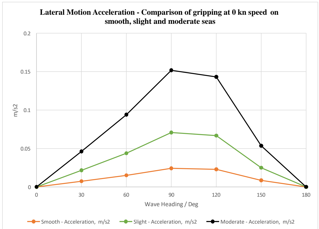
Figure 8-28 Lateral Motion Acceleration at Gripper point on three different Sea States
