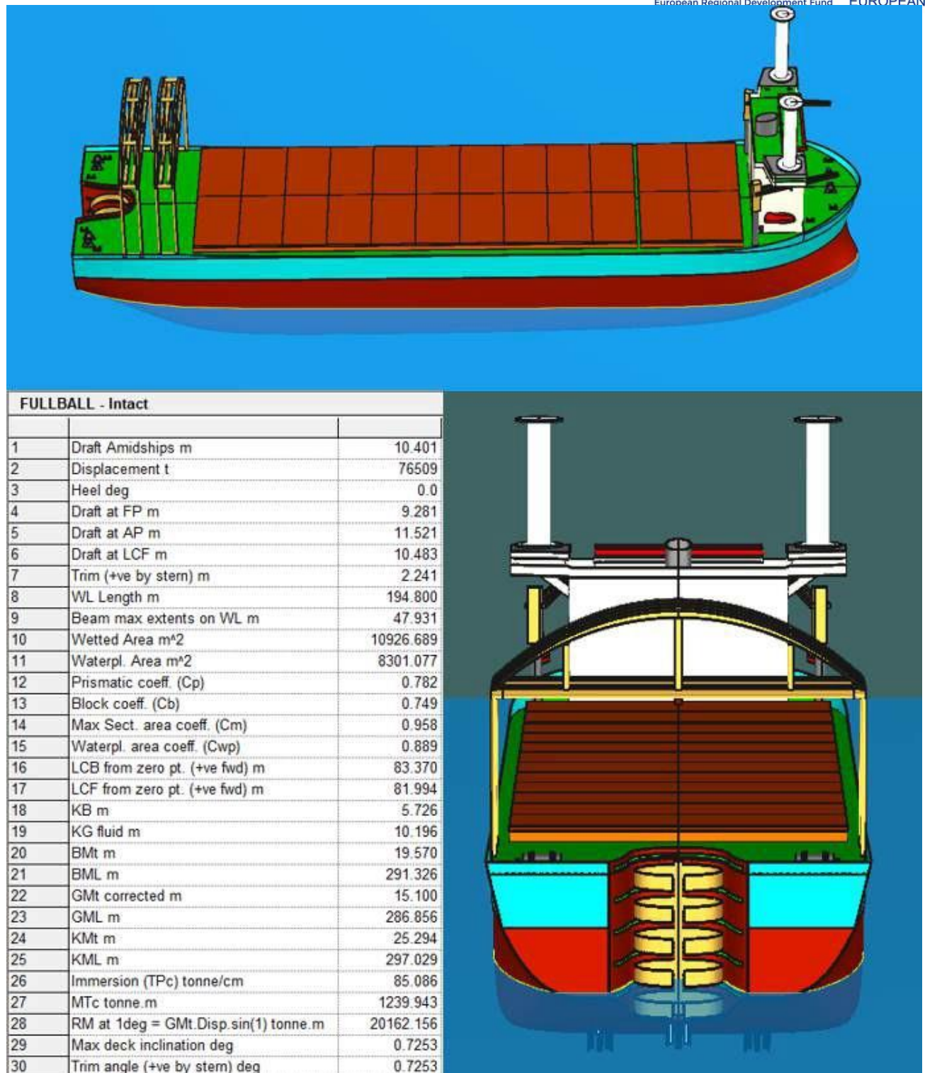
Figure 7-12 Decom Tools Vessel at full Ballast Equilibrium
