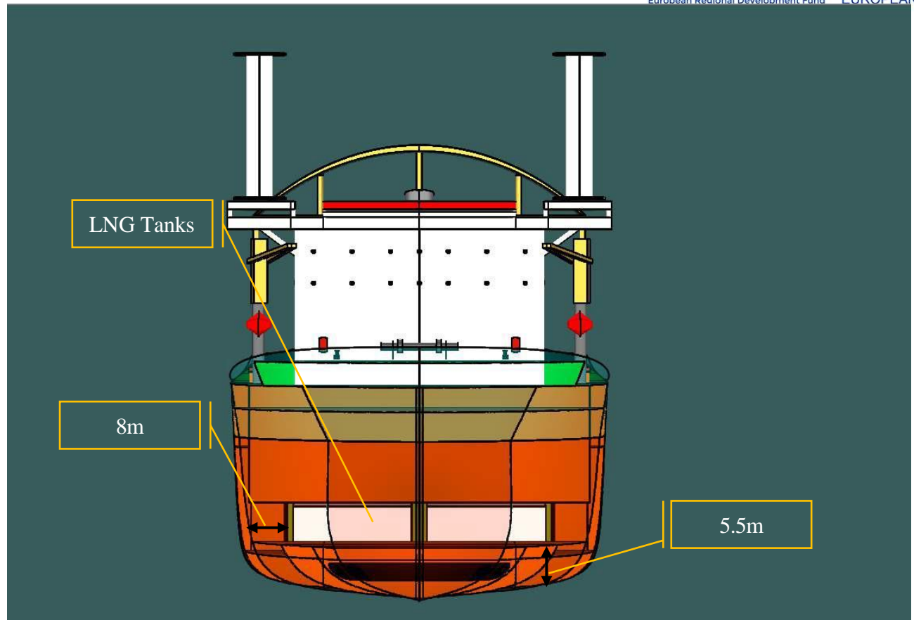
Figure 5-34 Location of LNG tanks of Decom Tools Vessel
