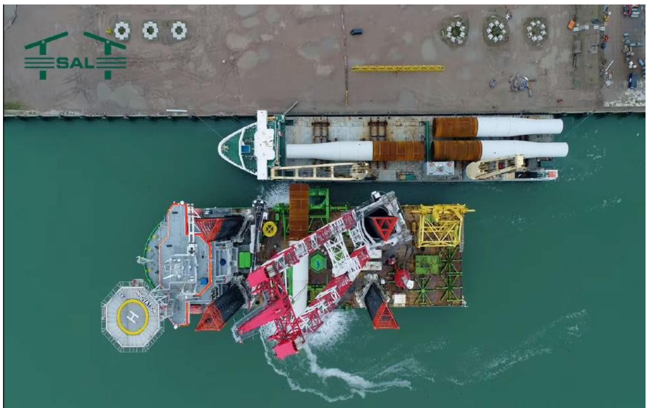
Figure 5-68 Loading of Monopile from Cargo Vessel to the Installation vessel (SAL 2019)
