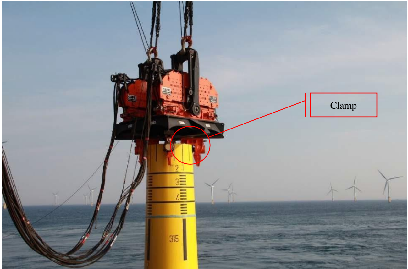
Figure 6-129 The connection of Clamps of Vibratory Hammer to the Monopile
