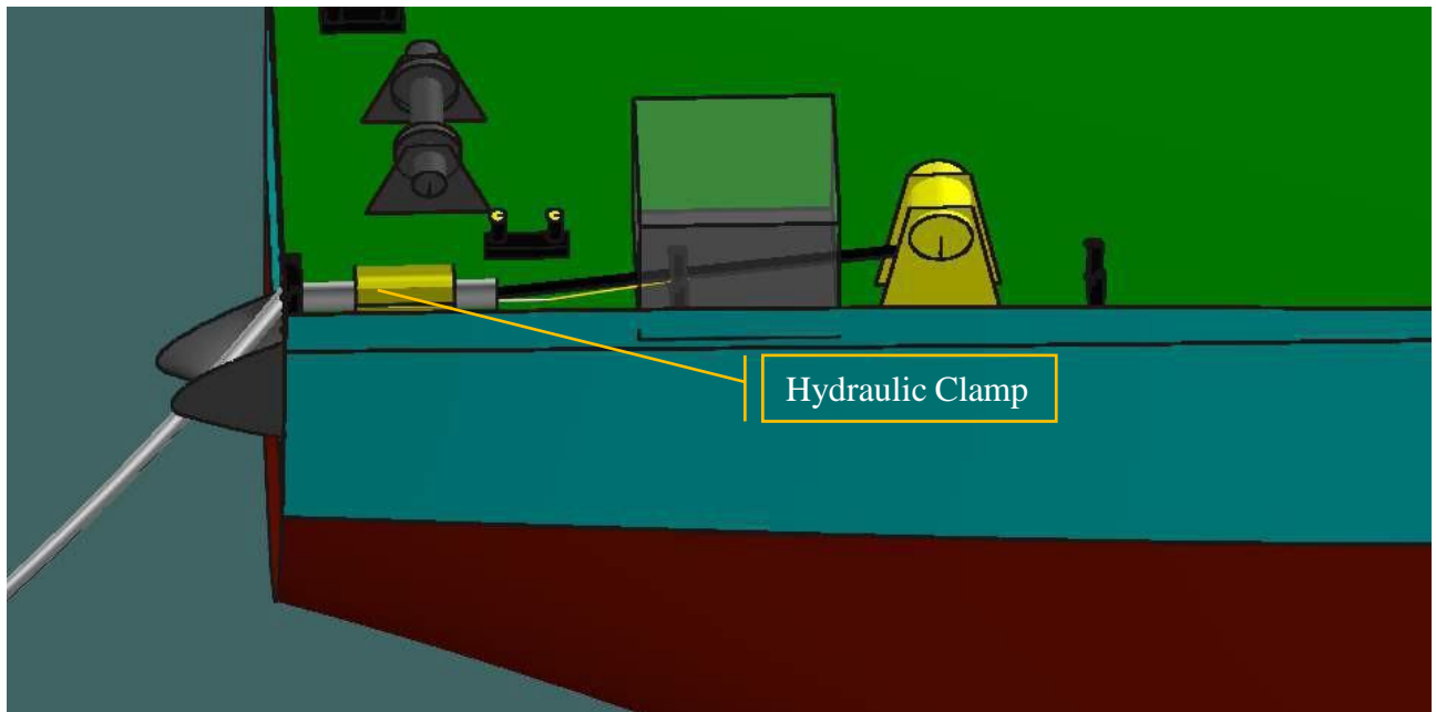
Figure 6-228 Hydraulic Clamp Tightened the Cable Firmly
