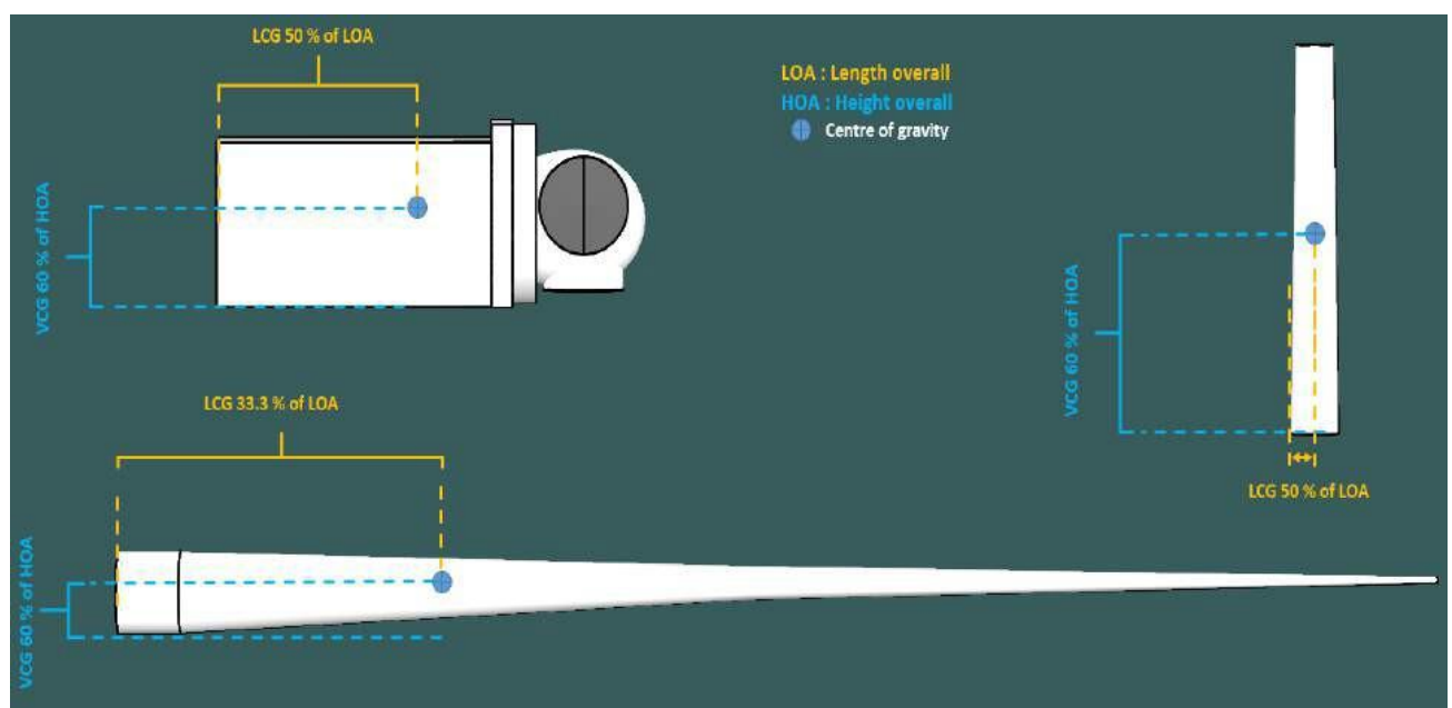
Figure 7-20 VCG, TCG & LCG of 12MW Wind Turbine
