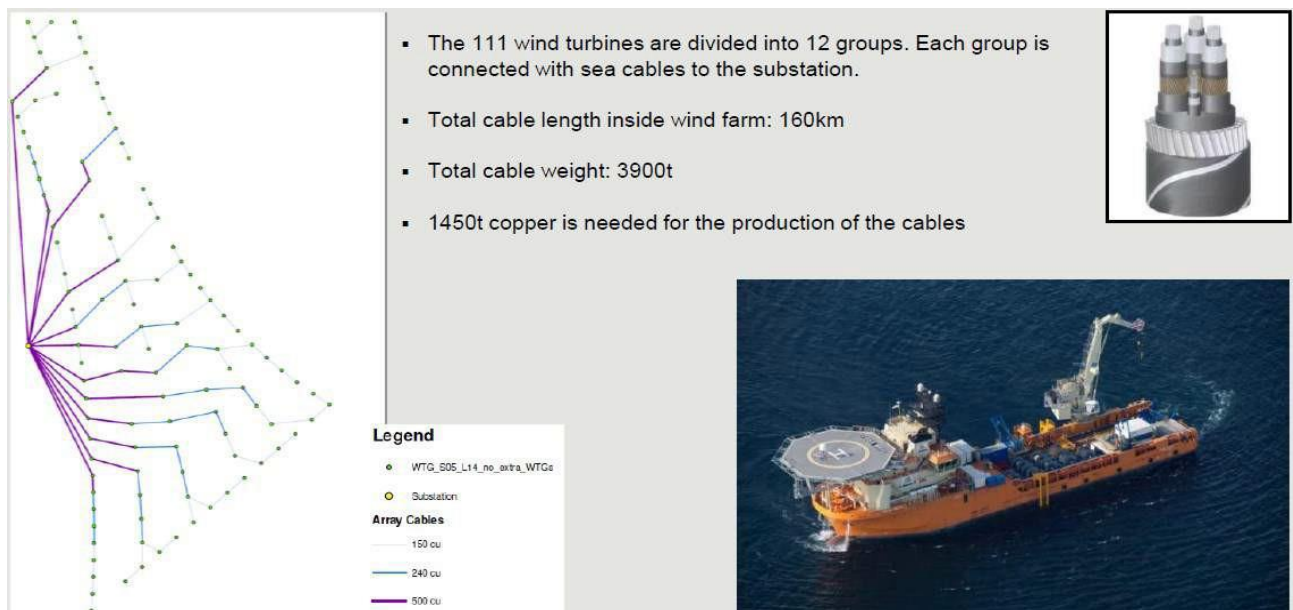
Figure 6-201 Information about Infield Cable of Anholt OWP (Orsted 2019)
