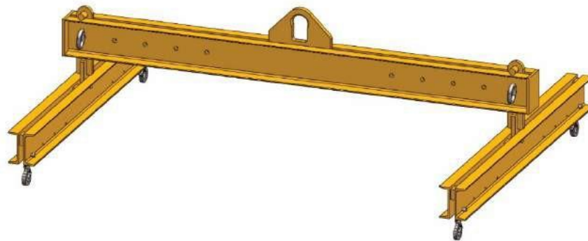
Figure 5-93 Hatch Cover Lifting Tool (TRI-STATE RIGGING EQUIPMENT n.d.)
