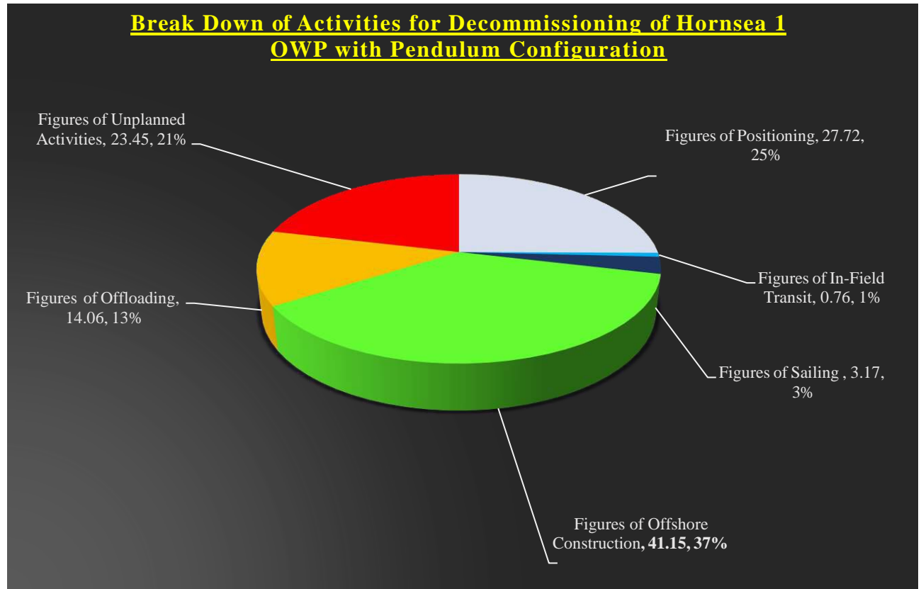
Figure 3-33 Break Down of Noblewind offshore Wind Farm Decommissioning with a Jack up
