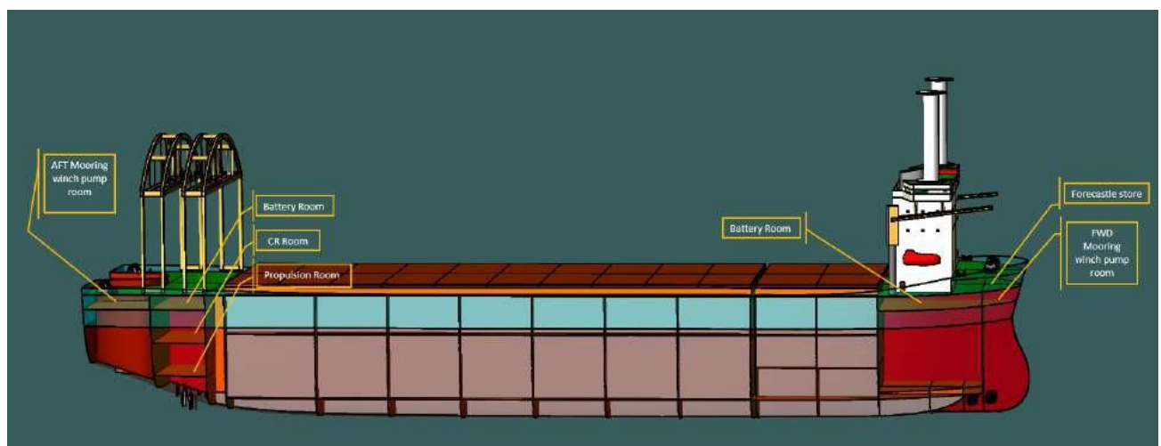
Figure 5-84 Engine room, Propulsion Room and Battery Room
