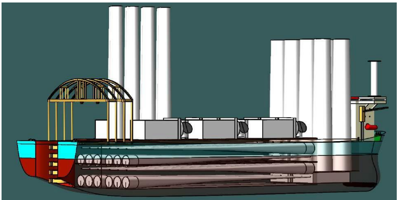
Figure 6-29 Perspective of Load out of 12MW Blades, Nacelle and Tower
