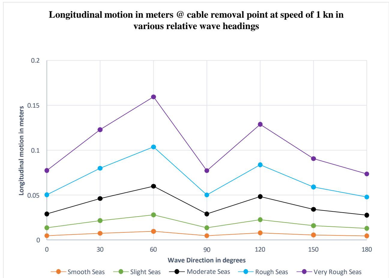
Figure 8-17 Comparison of longitudinal movement during cable removal operation in various sea state
