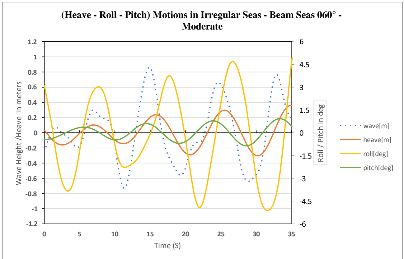
Figure 8-23 Motion in irregular beam seas 060^\circ – Moderate
