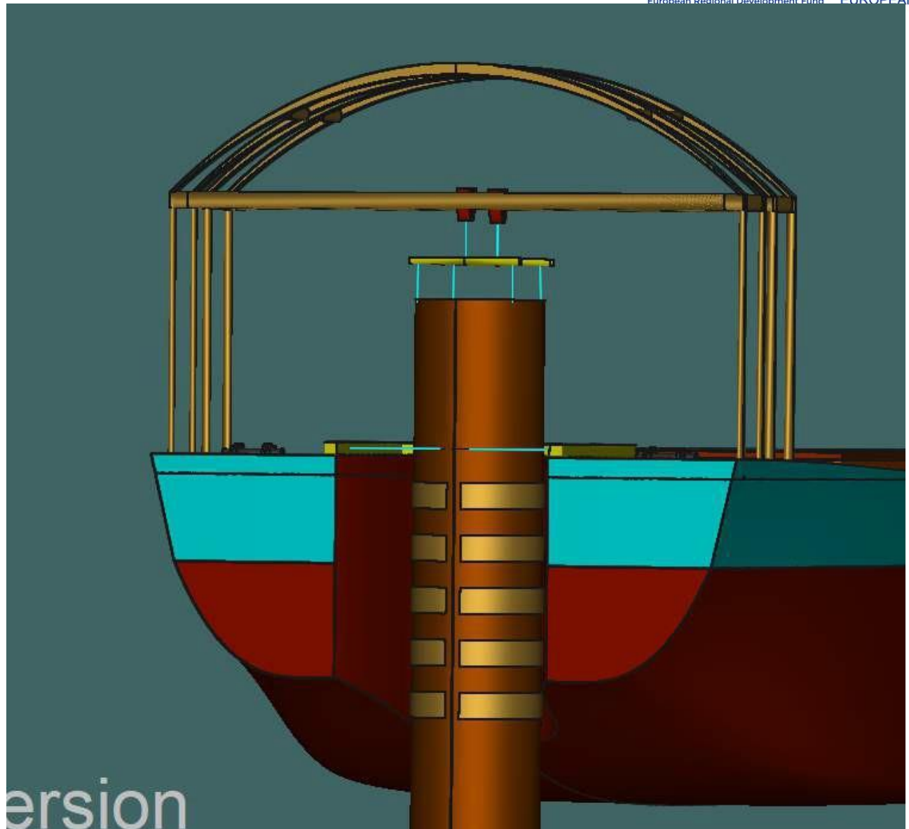
Figure 6-146 Commencement of Cutting with Diamond Wire Cutter
