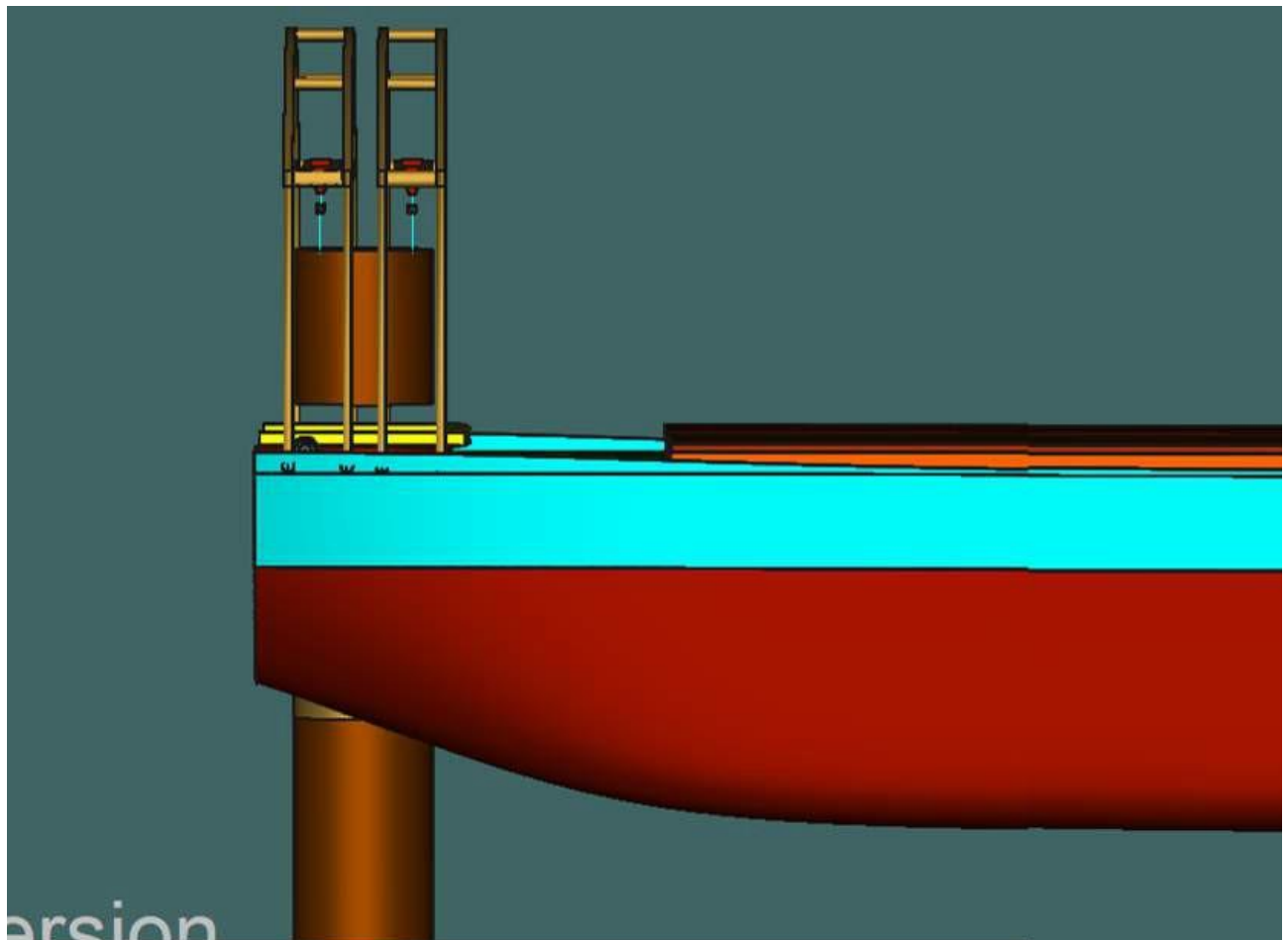
Figure 6-152 Lifting the Cut section of Monopile (Side view)
