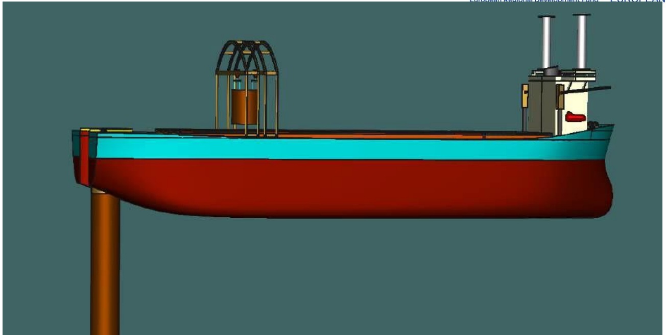
Figure 6-153 Transferring the Cut Section of Monopile
