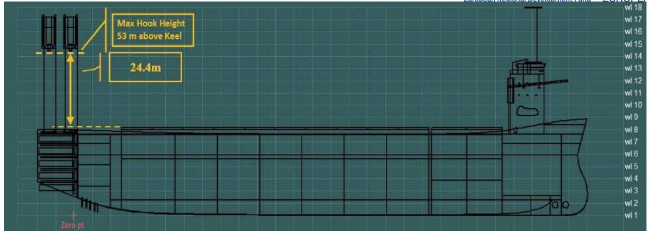
Figure 5-42 Height of Gantry Crane
