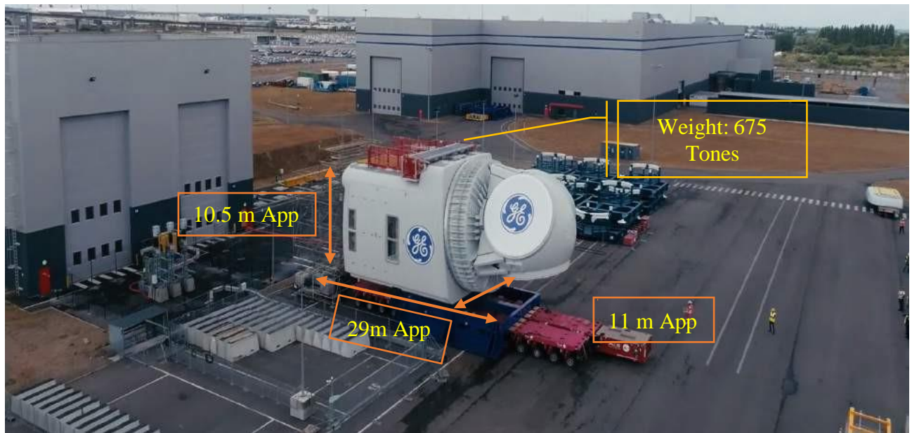
Figure 6-6 Transportation of 12MW GE X-Heliade Nacelle (Energyfacts.eu 2019)
