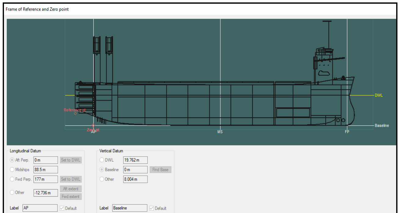
Figure 7-1 Decom Tools Vessel Coordinates
