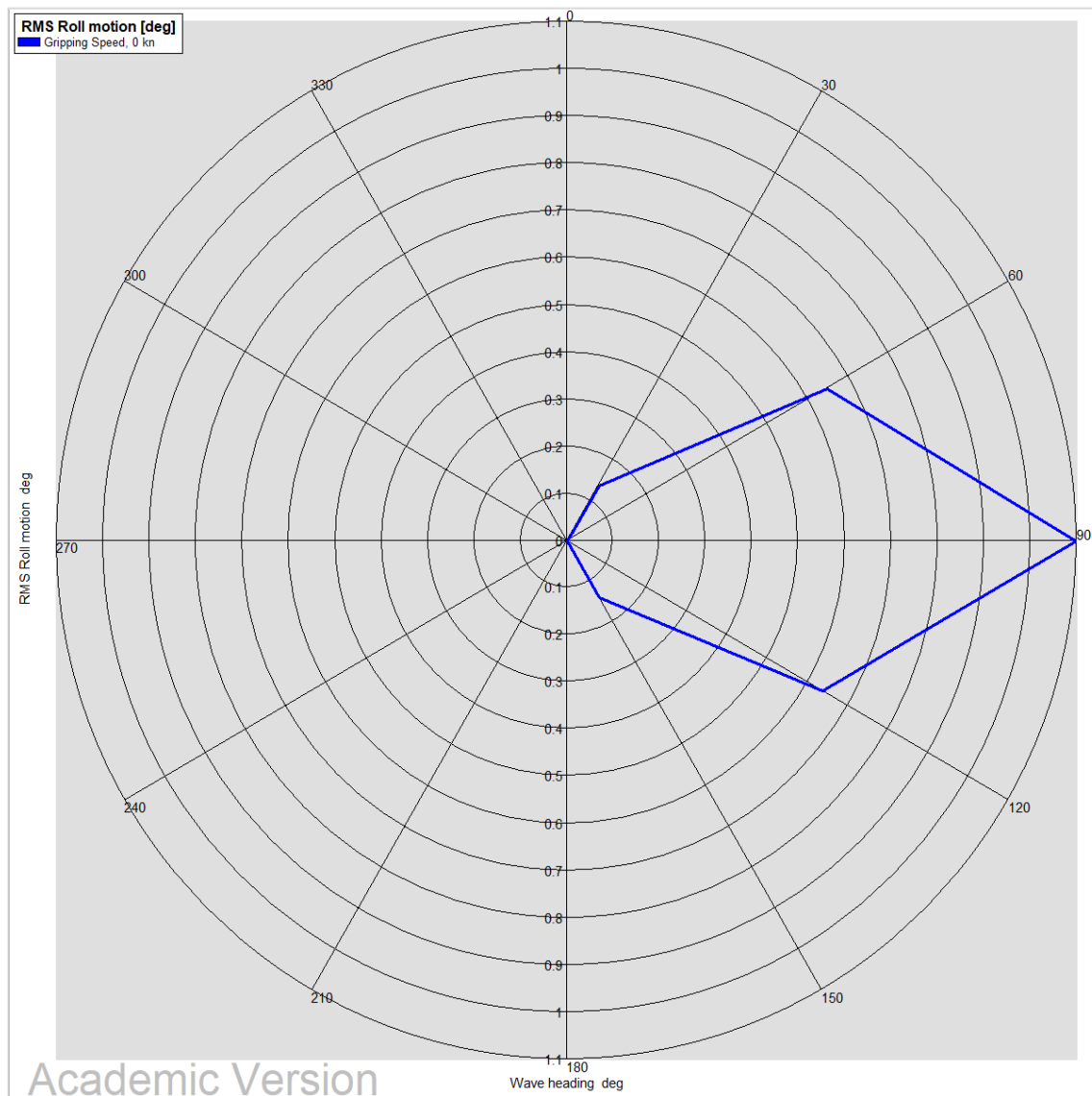
Figure 8-9 Roll Motion at COG – Slight Sea state
