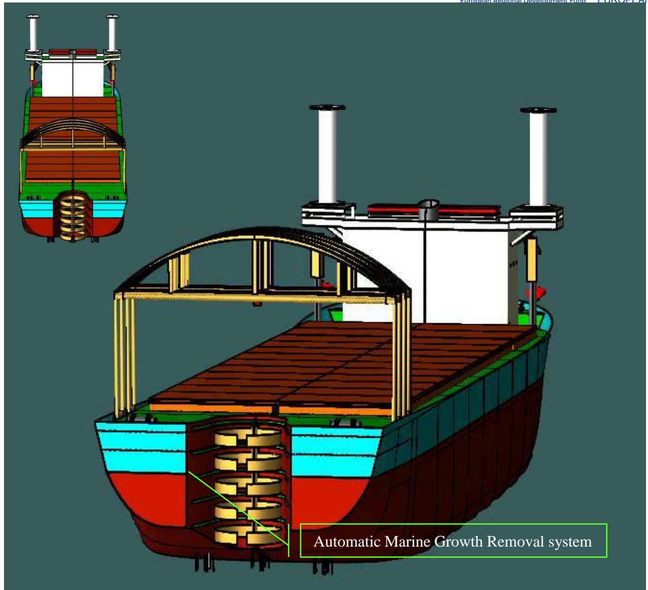
Figure 5-86 Perspective and Back View of Decom Tools Vessel
