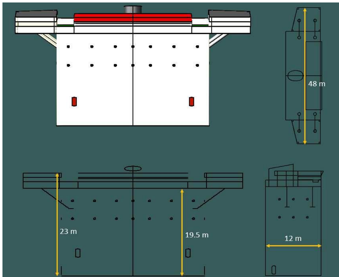
Figure 5-37 Dimension of Accommodation
