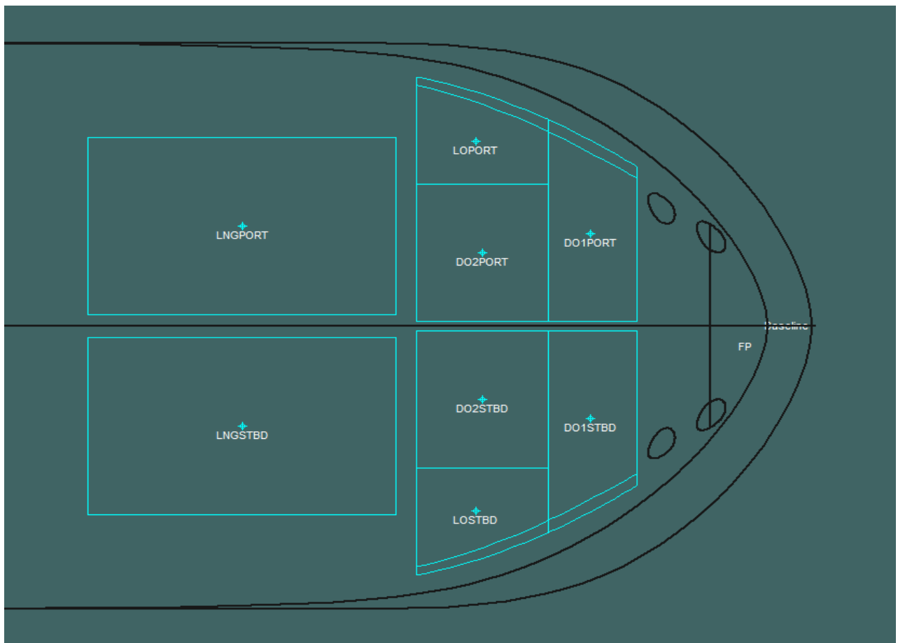
Figure 5-33 Plan of LNG and Diesel Oil Tanks
