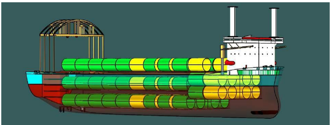
Figure 6-168 Loading of 24 set of MP plus TP (Perspective View)
