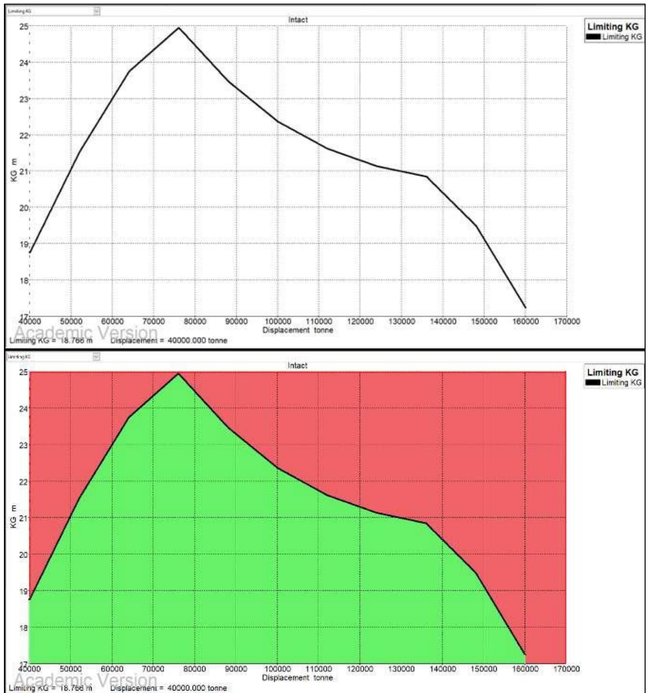
Figure 7-15 KG limit Based on IMO Intact Stability Criteria
