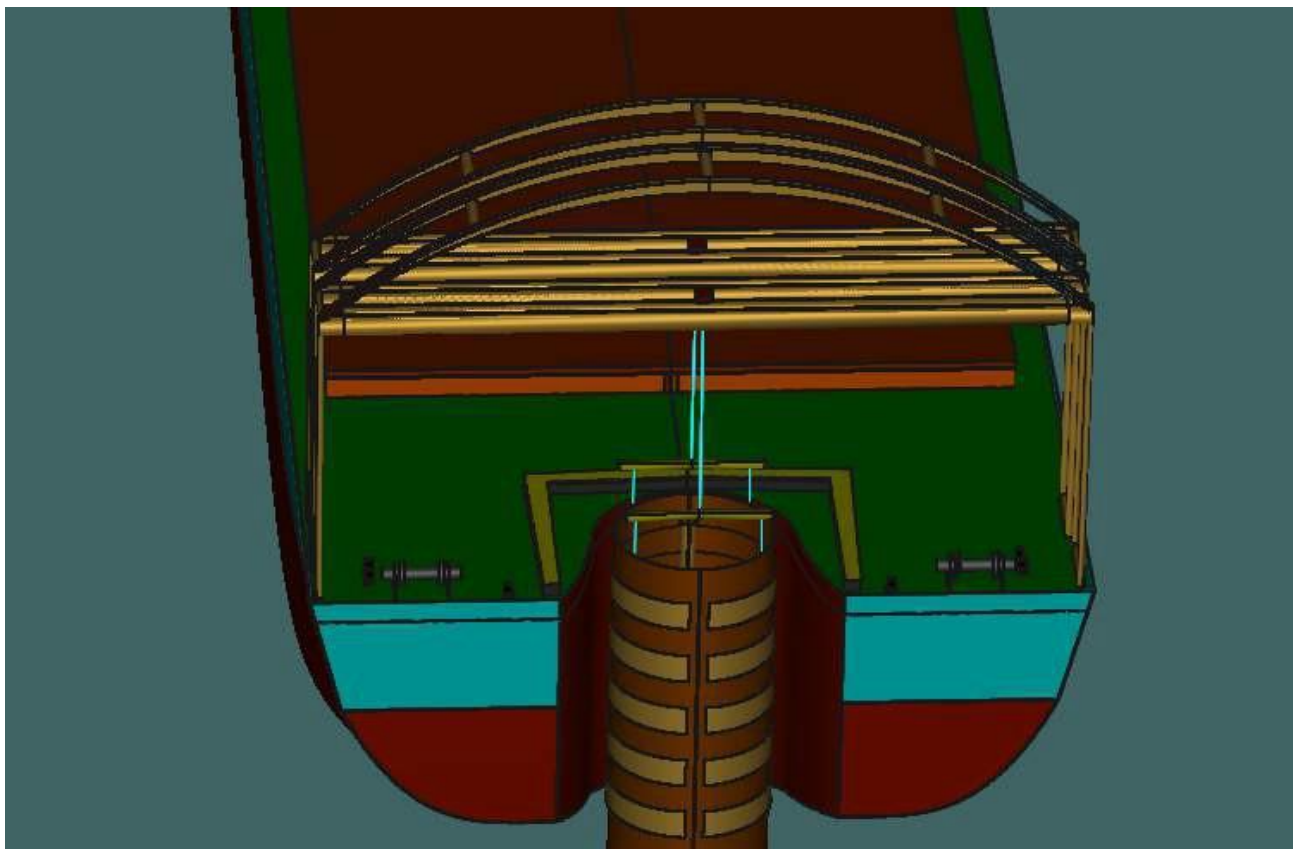
Figure 6-137 Plan of Tandem connection of Cranes to the monopile and Spreader bar
