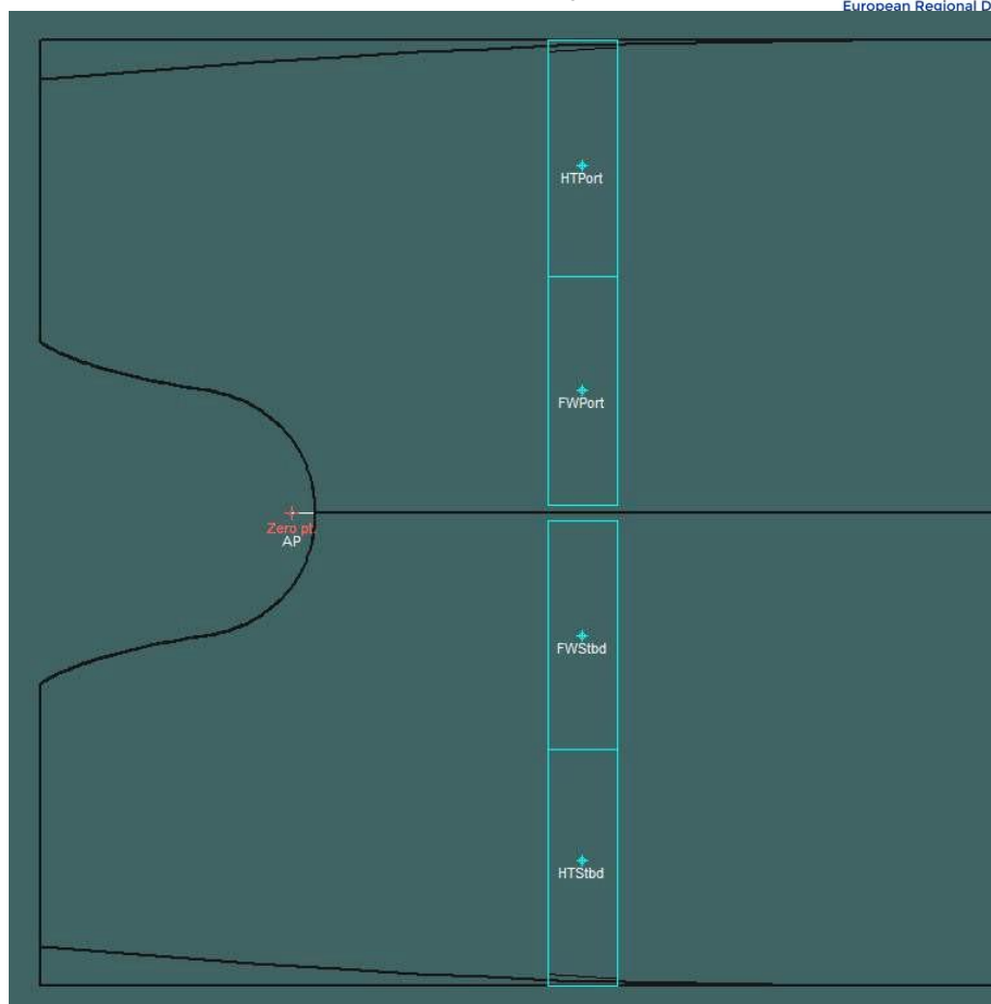
Figure 5-36 Plan of Fresh Water and Heeling Tanks
