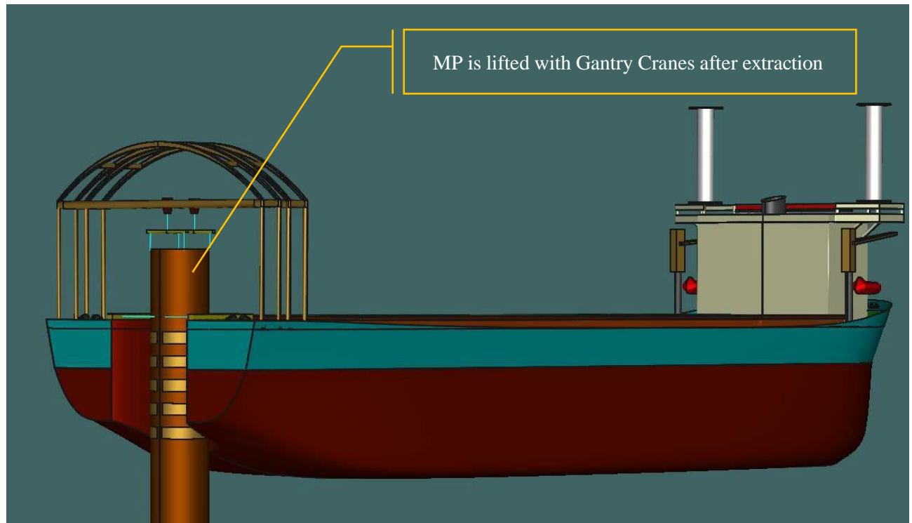
Figure 6-138 Pile is lifted with both cranes after extraction
