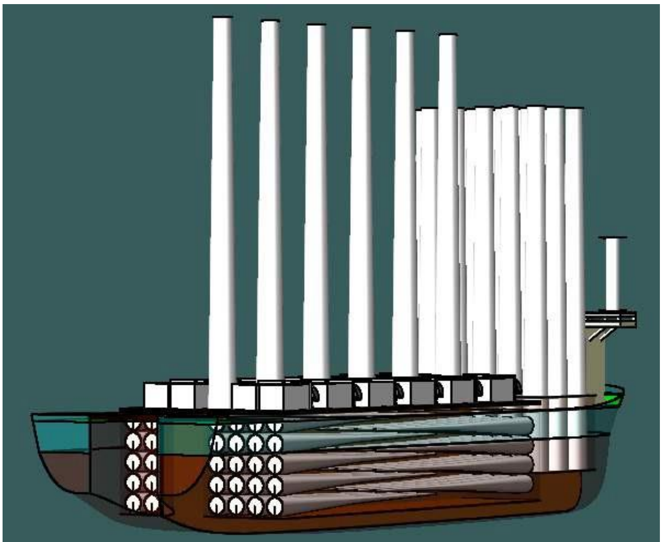
Figure 6-37 Perspective of Load out of 5MW Wind Turbine
