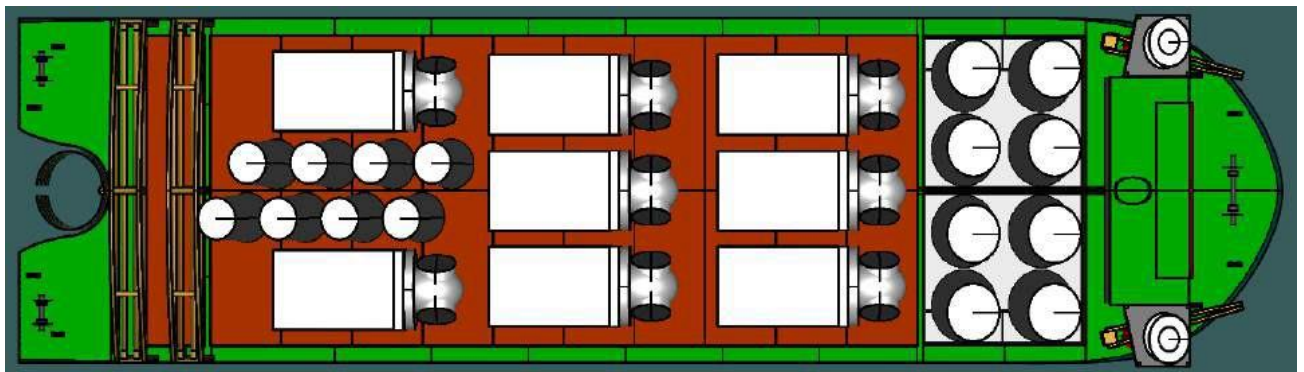
Figure 6-26 Top View of Load out of 12MW Blades, Nacelle & Tower
