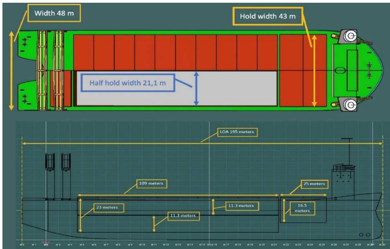
Figure 5-8 Dimension of Decom Tools Vessel
