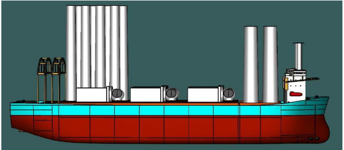
Figure 6-25 Side View of Load out of 12MW Blades, Nacelle & Tower
