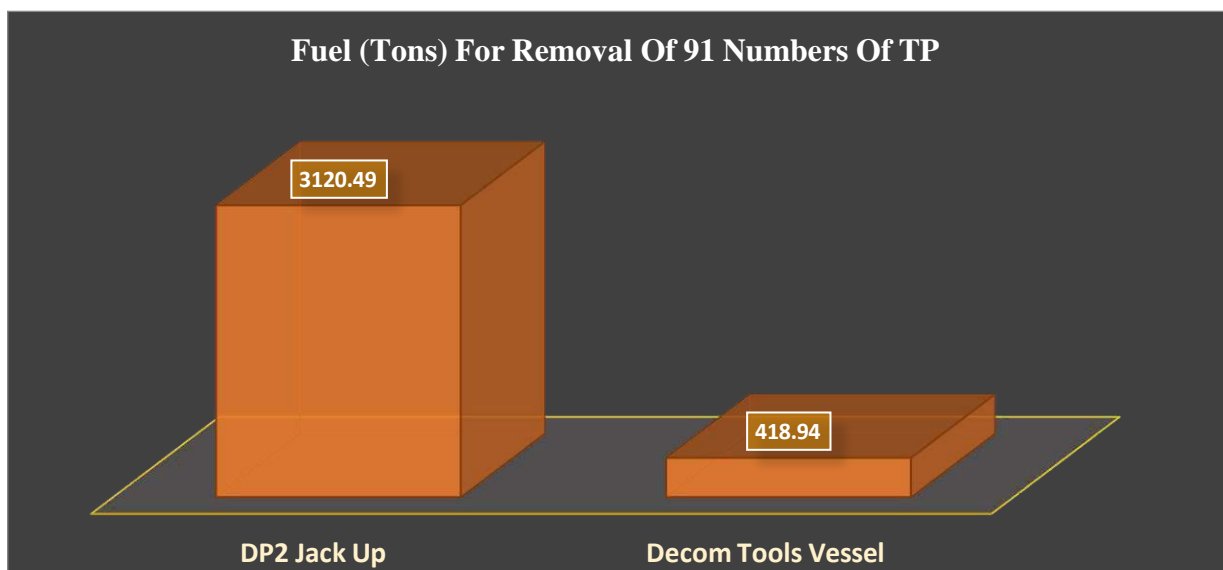
Figure 6-114 Fuel Consumption During Removal of 91 Number of TP
