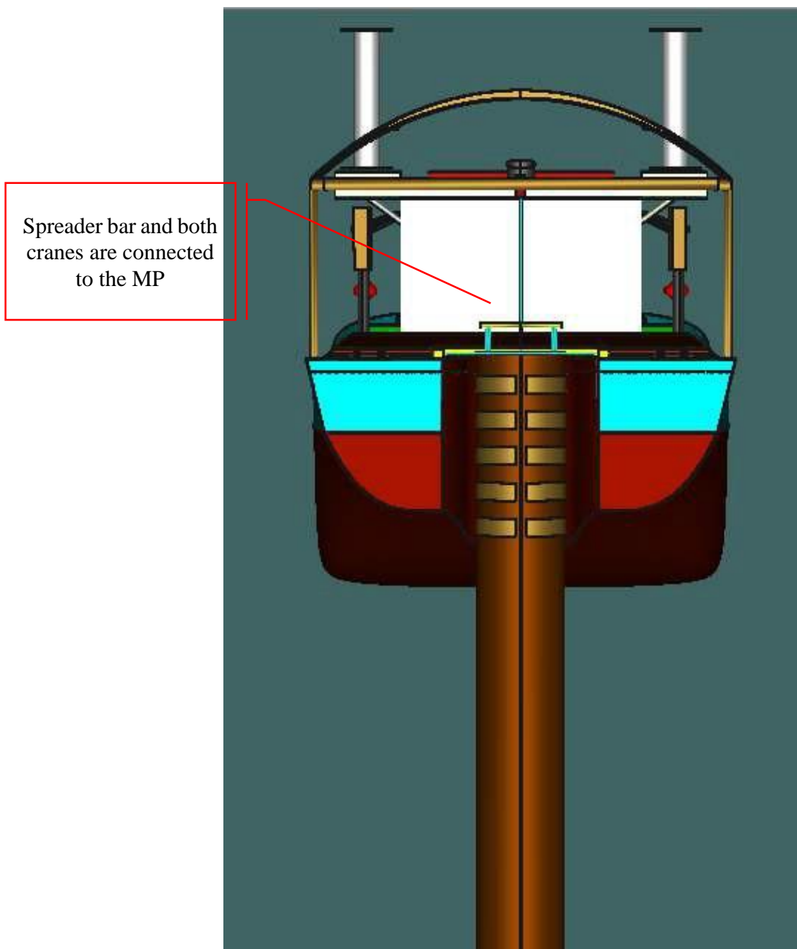
Figure 6-135 Both Cranes are connected to the monopile in tandem configuration
