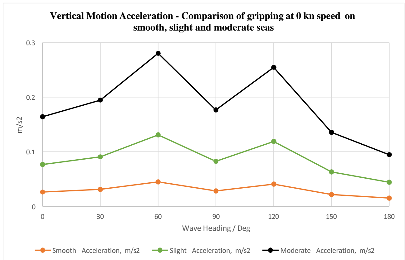
Figure 8-26 Absolute Vertical acceleration at Gripper point on three different Sea States
