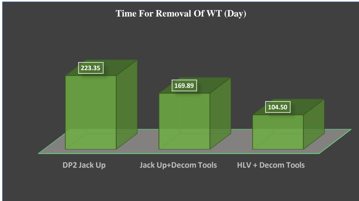
Figure 3-43 Duration of Decommissioning of Hornsea 1 OWP
