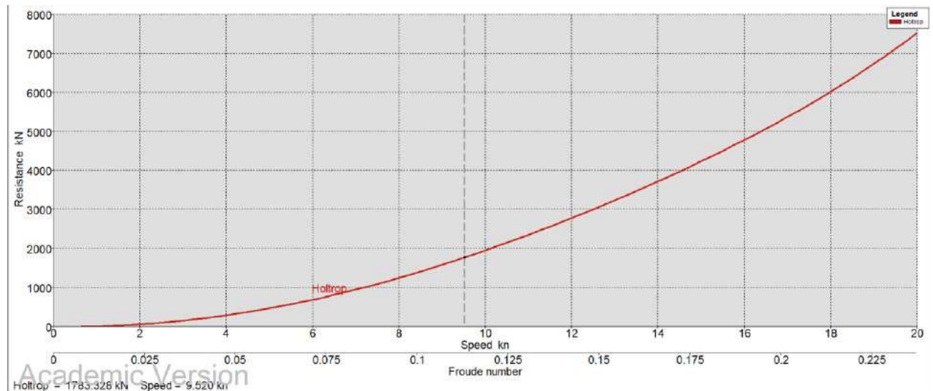
Figure 5-64 Correlation Between Speed and Resistance at Draft of 19.79 meters
