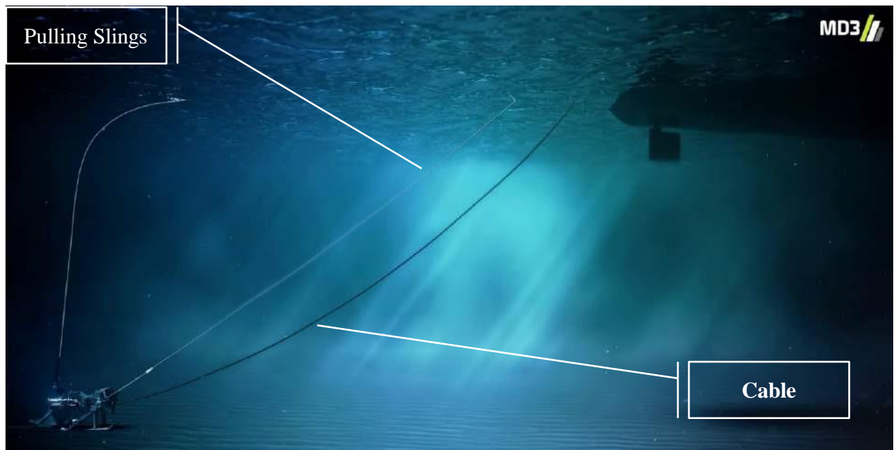
Figure 6-185 Cable Plough (SMD - Subsea Technology 2014)
