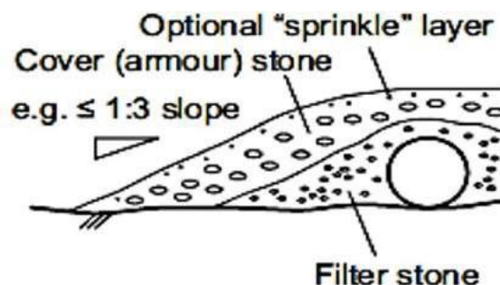
Figure 6-181 Rock Dumped on the cable as means of protection
