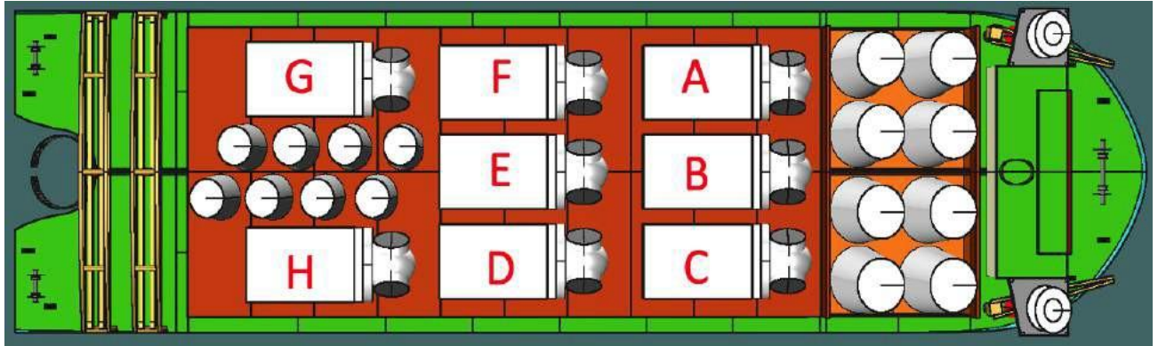
Figure 7-21 12 MW Wind Turbine Arrangement
