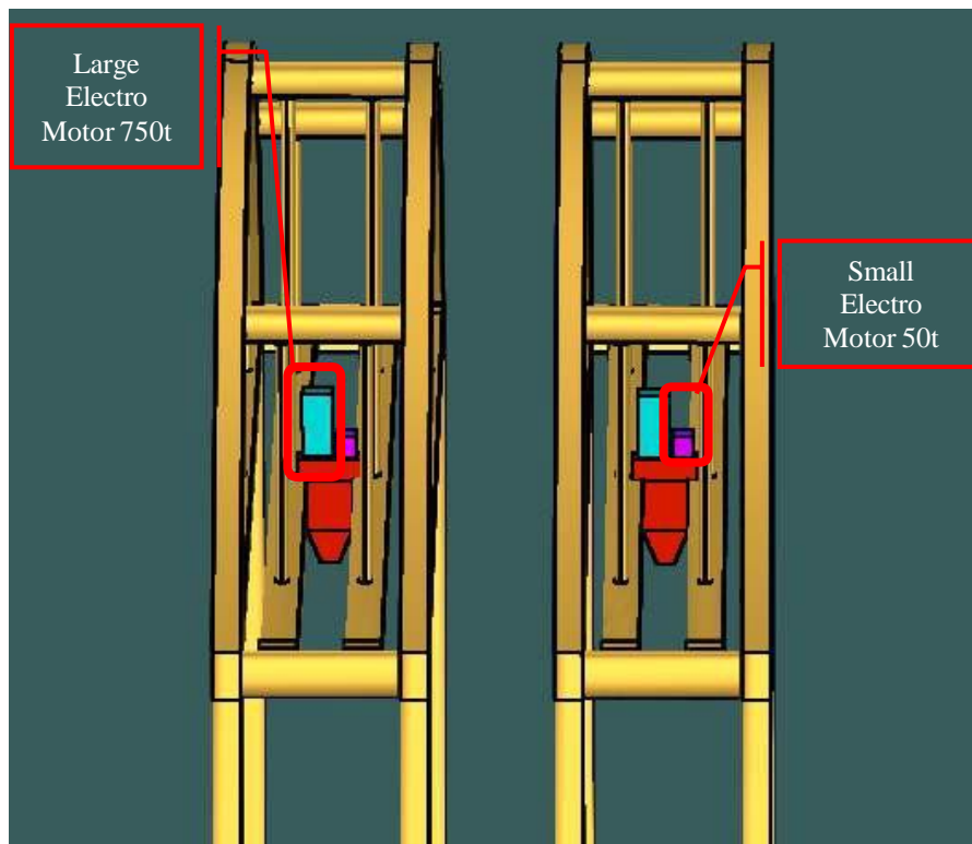
Figure 5-41 Electro Motors of Gantry Cranes
