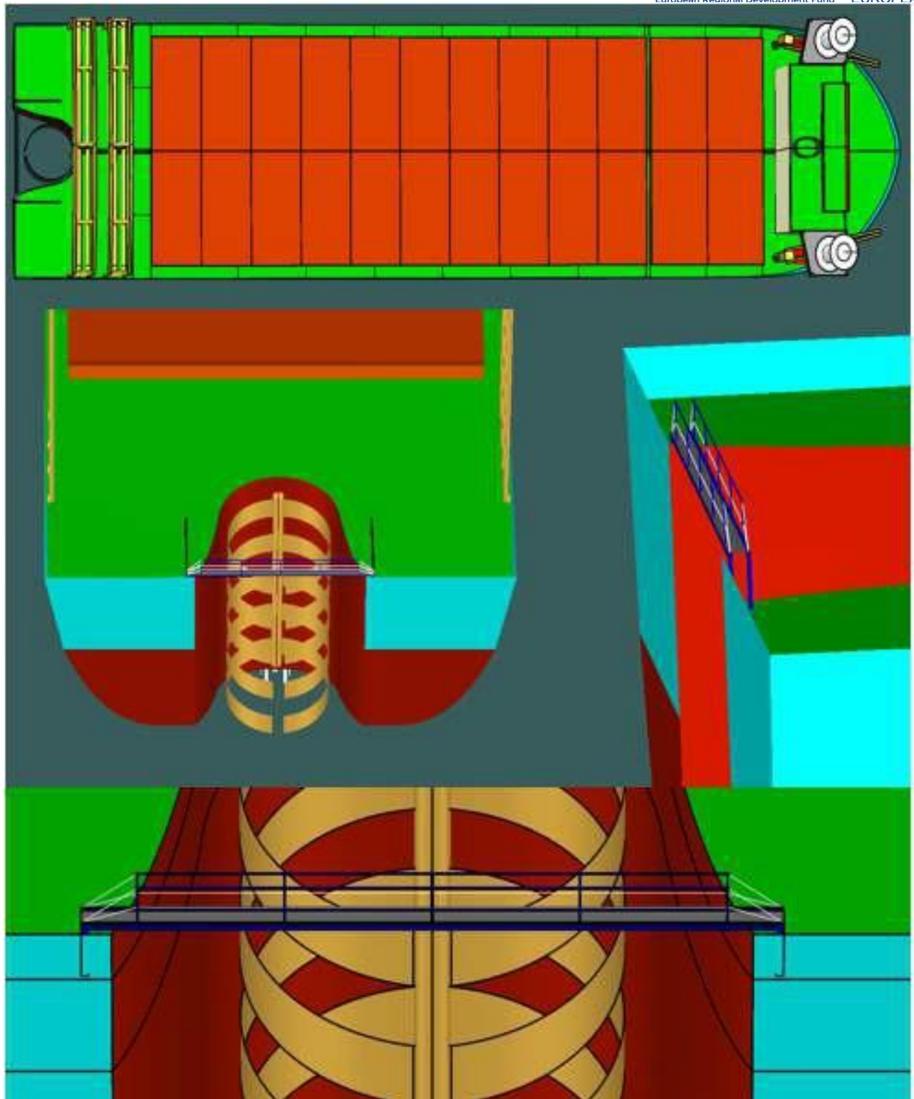
Figure 6-95 Mobile Access Platform for Cutting MP/TP
