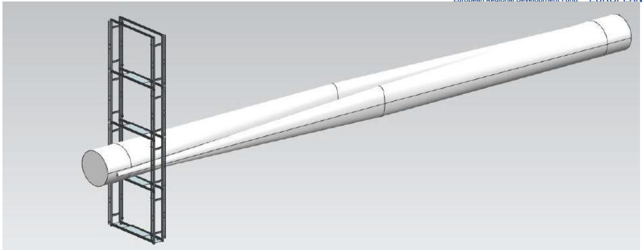
Figure 6-78 Securing 2 numbers of 5MW blades inside the racks
