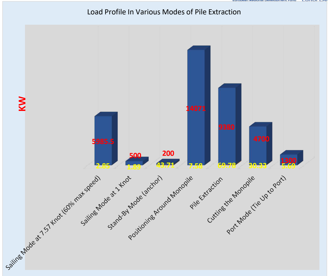
Figure 5-76 Load Profiles During Pile Extraction
