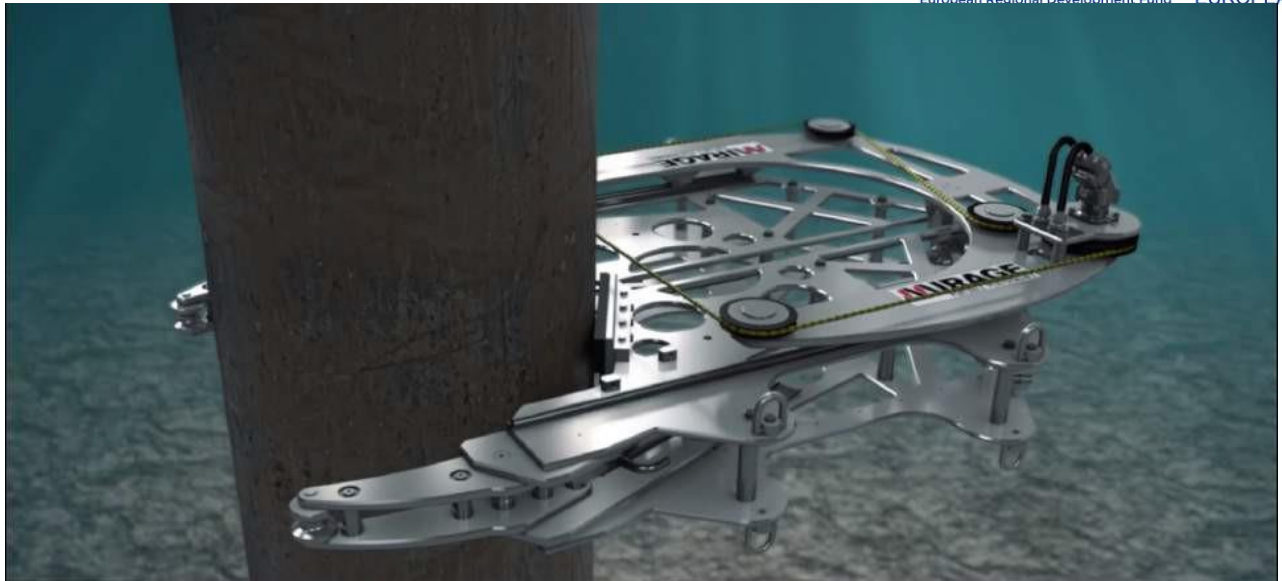
Figure 6-140 Small-Size Diamond Wire saw (MirageMachines 2015)
