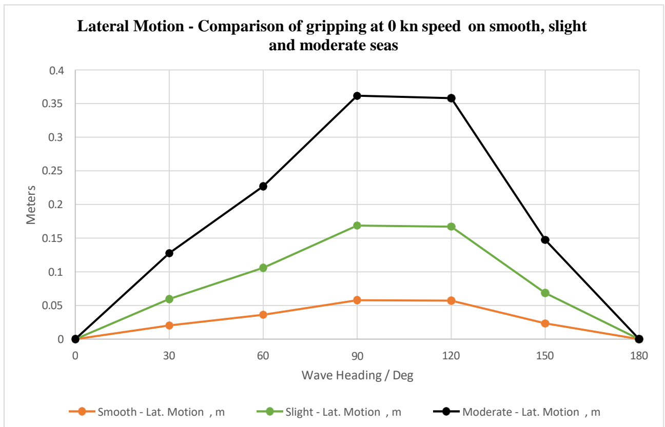
Figure 8-13 Lateral Motion at Gripper point on three different Sea States
