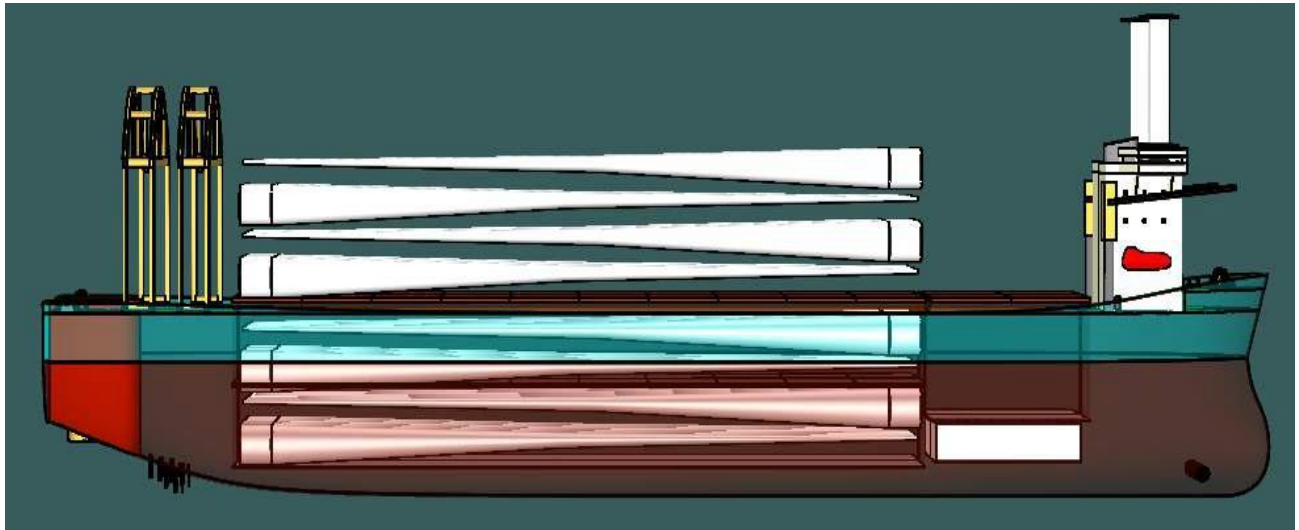
Figure 7-33 Decom Tools Vessel is Loaded with 48 Numbers of Blades
