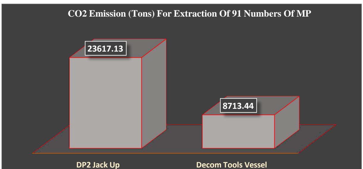
Figure 6-175 Comparison of CO2 Emission for MP Extraction
