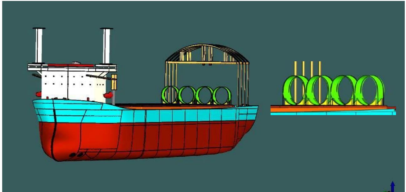
Figure 6-169 Seafastening of MP & TP After Cutting & MGR (Perspective View)
