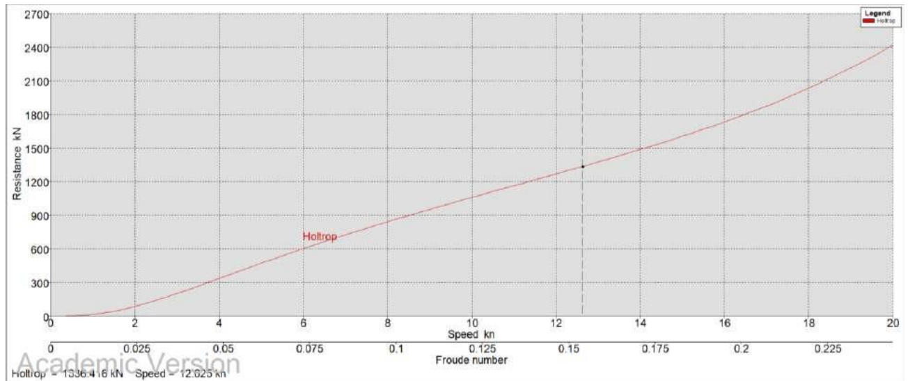
Figure 5-62 Correlation Between Speed and Resistance at Draft of 6 meters
