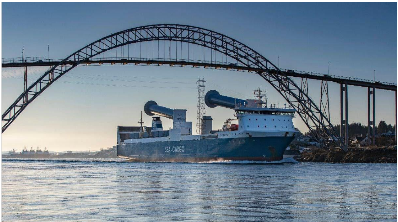
Figure 5-53 Tiltable Flettner Rotor (VPO 2021)
