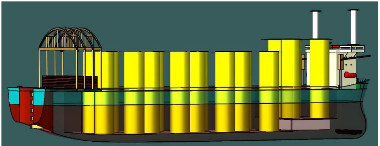
Figure 6-47 Perspective View of Load of 12MW TP with Decom Tools Vessel
