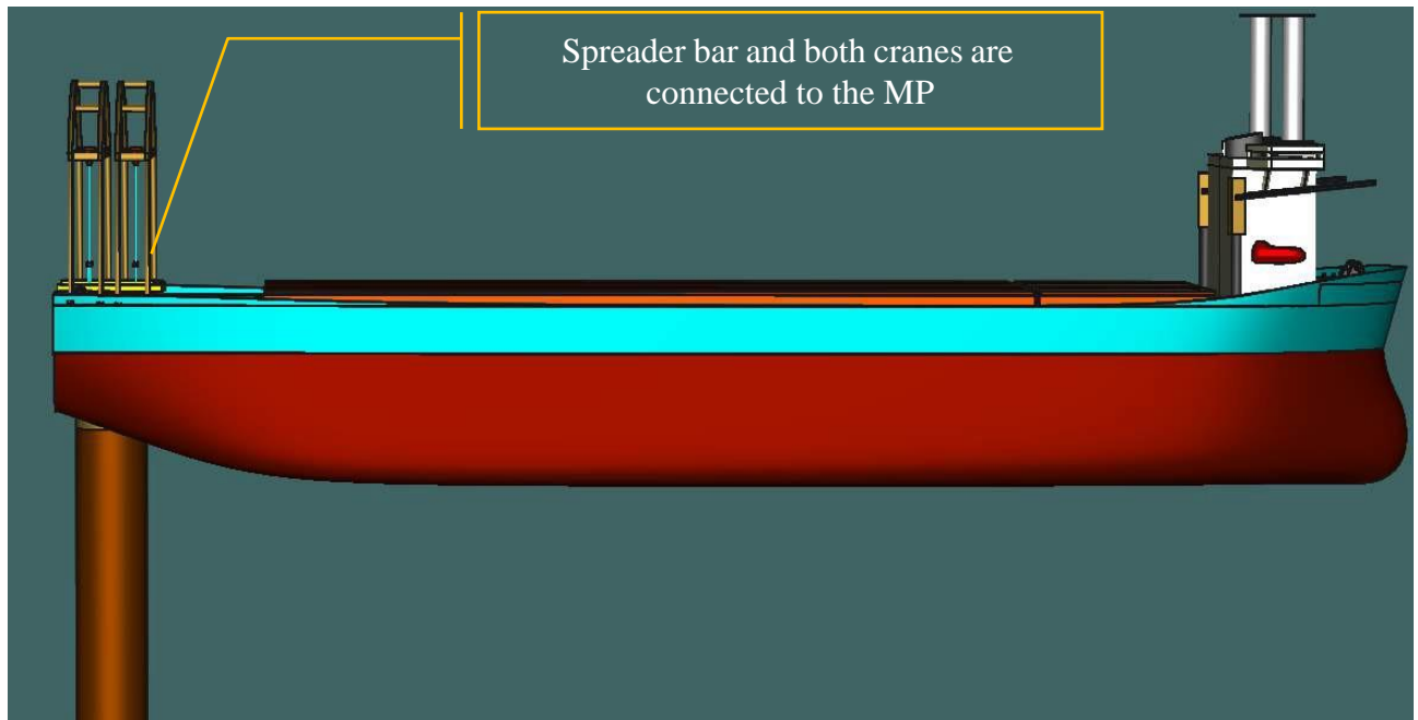
Figure 6-136 Both Cranes are connected to the monopile in tandem configuration
