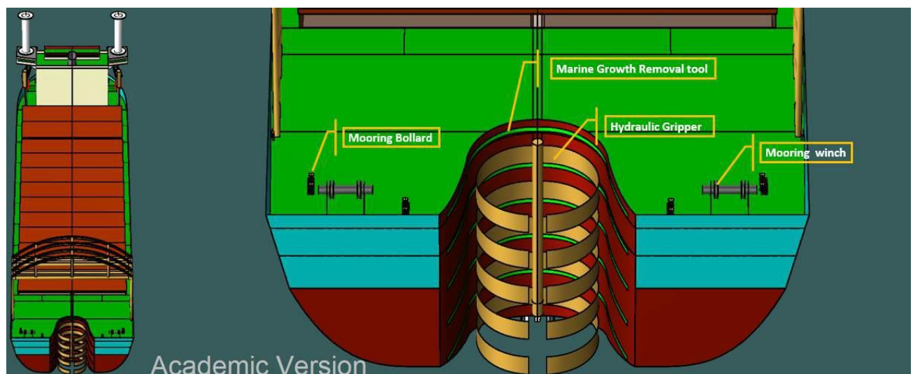
Figure 6-157 The Marine Growth System (In green colour)
