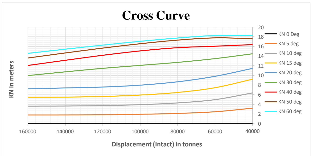
Figure 7-18 KN Curves of Decom Tools Vessel
