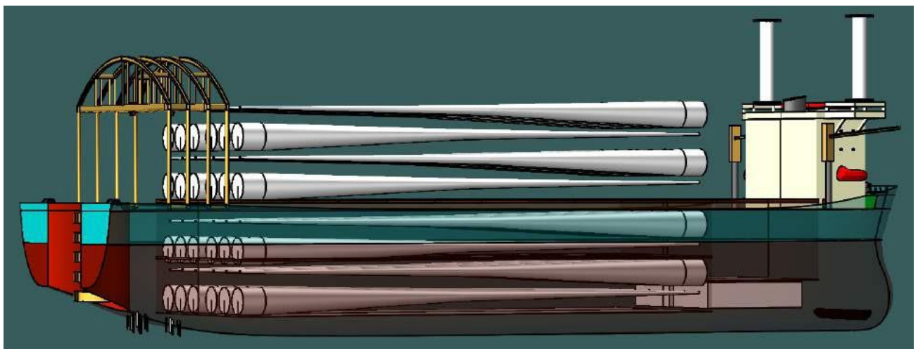
Figure 6-48 Perspective View of Load of 12MW Blade with Decom Tools Vessel
