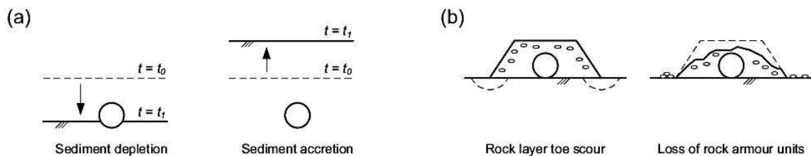
Figure 6-179 Change of Depth of lowering of the Cable during lifetime (DNV.GL 2016)
