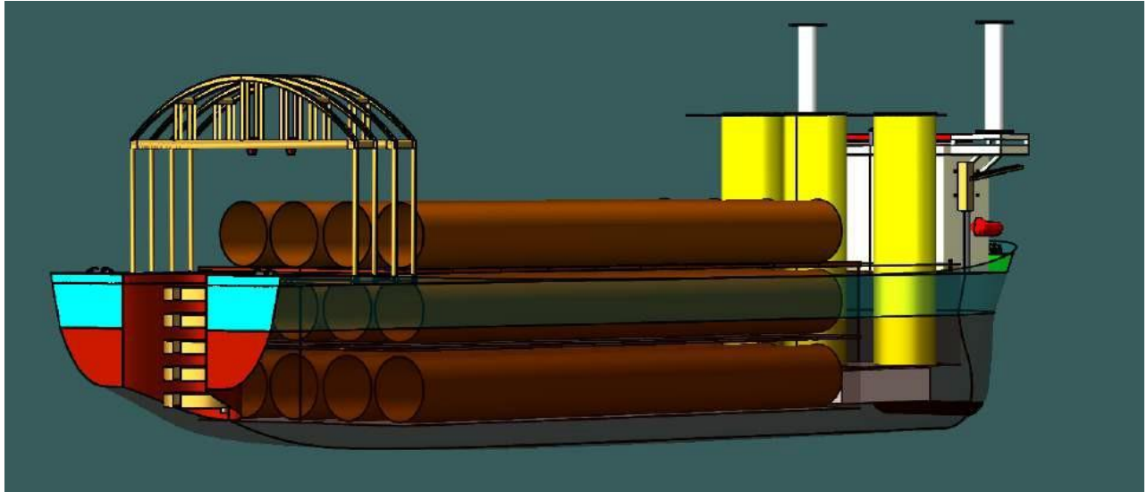
Figure 6-33 Perspective of Load out of TP and Monopile (Second Arrangement)
