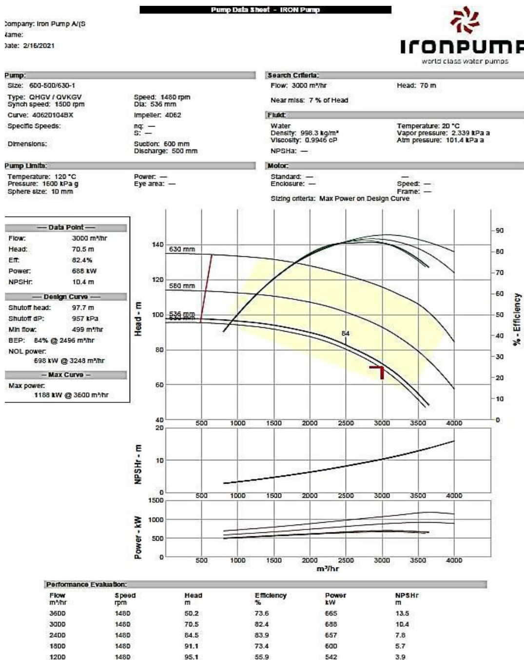
Figure 5-61 Specification of Ballast Pump
