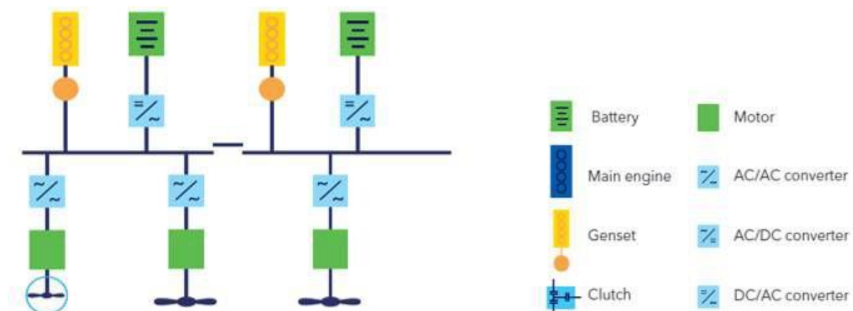
Figure 4-32 Hybrid Battery
