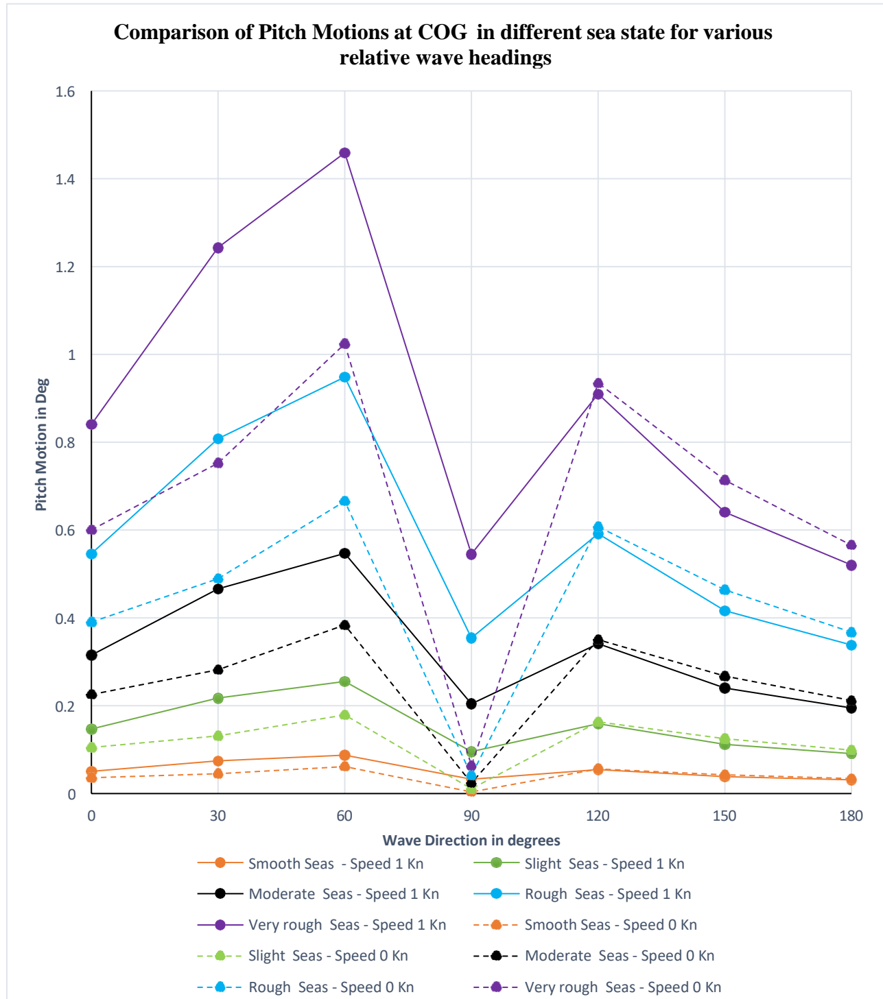
Figure 8-8 Comparison of Pitch Motions at COG in different sea state
