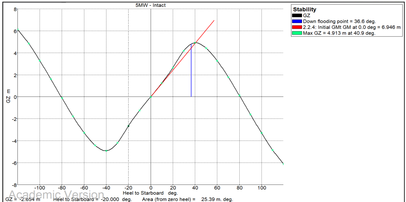
Figure 7-36 GZ Curve after Loading 24 sets of 5 MW Wind Turbine
