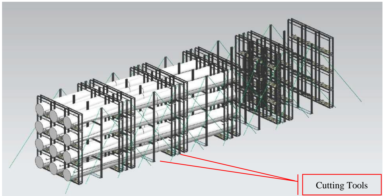
Figure 6-76 5MW blades inside the racks
