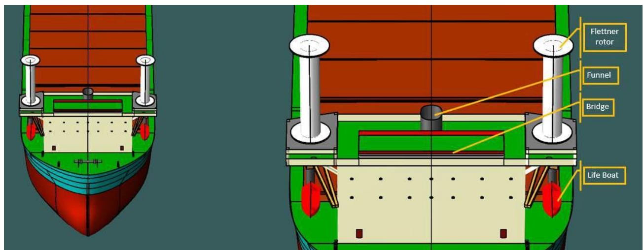
Figure 5-89 Details of Bow of the Decom Tools Vessel
