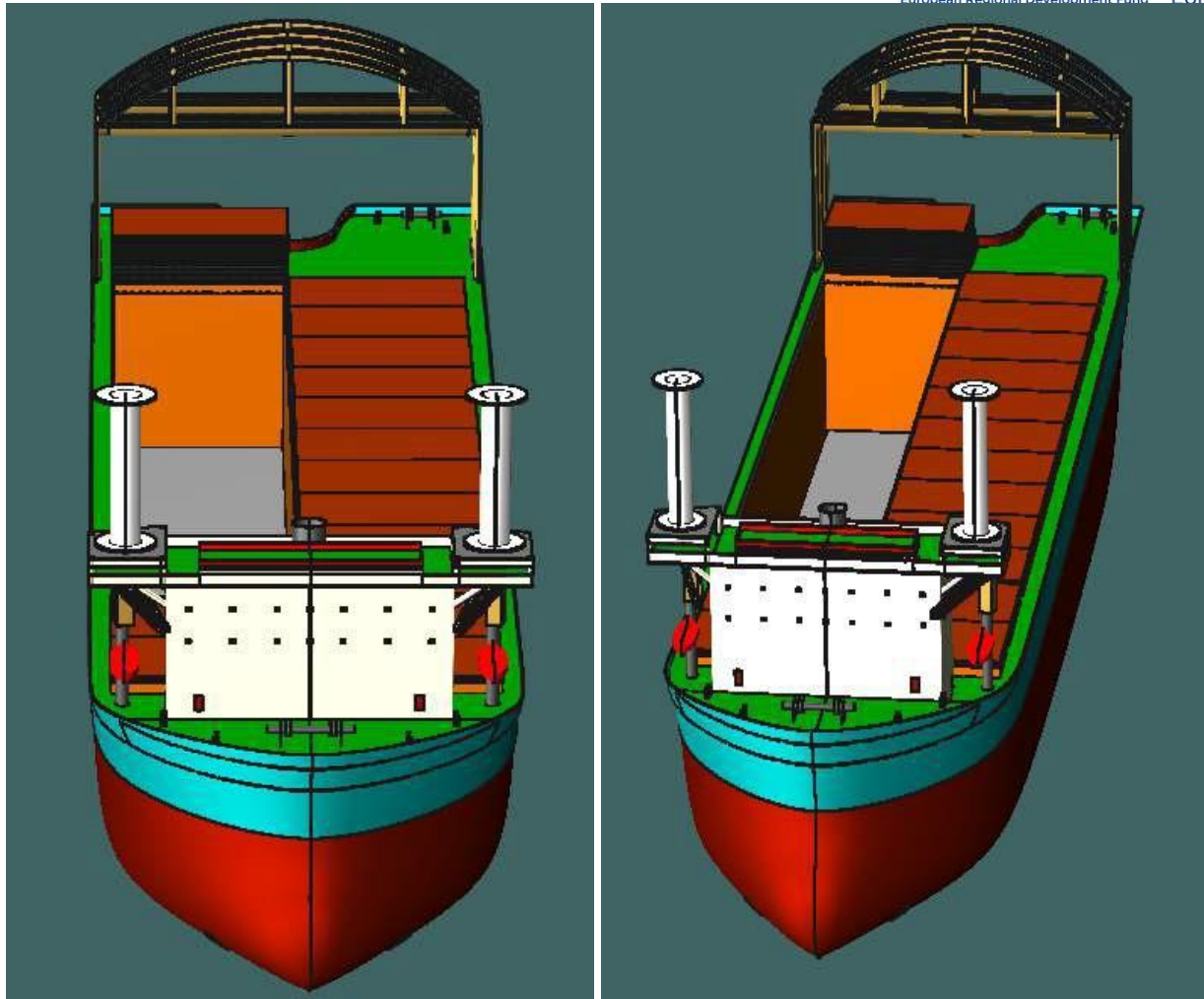
Figure 5-98 Bird's-eye view of the Vessel after Opening the Hatch covers
