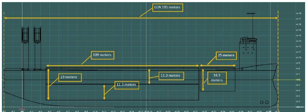
Figure 5-19 Dimension of Decks and Holds
