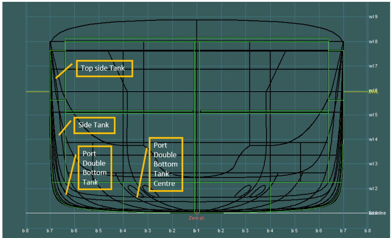
Figure 5-25 Bow View of Double Bottom Tanks, Side Tanks and Topside Tanks
