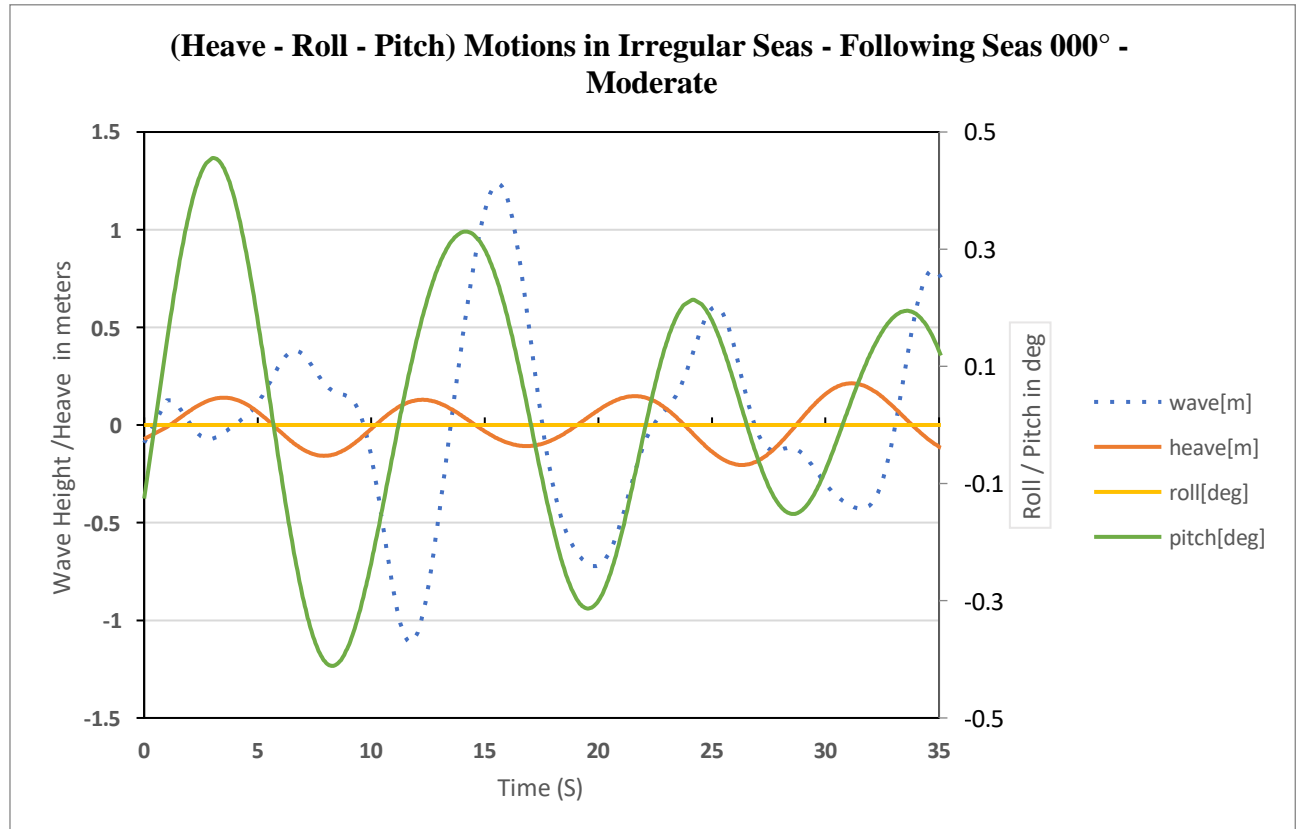
Figure 8-25 Motion in irregular following seas 000° – Moderate
