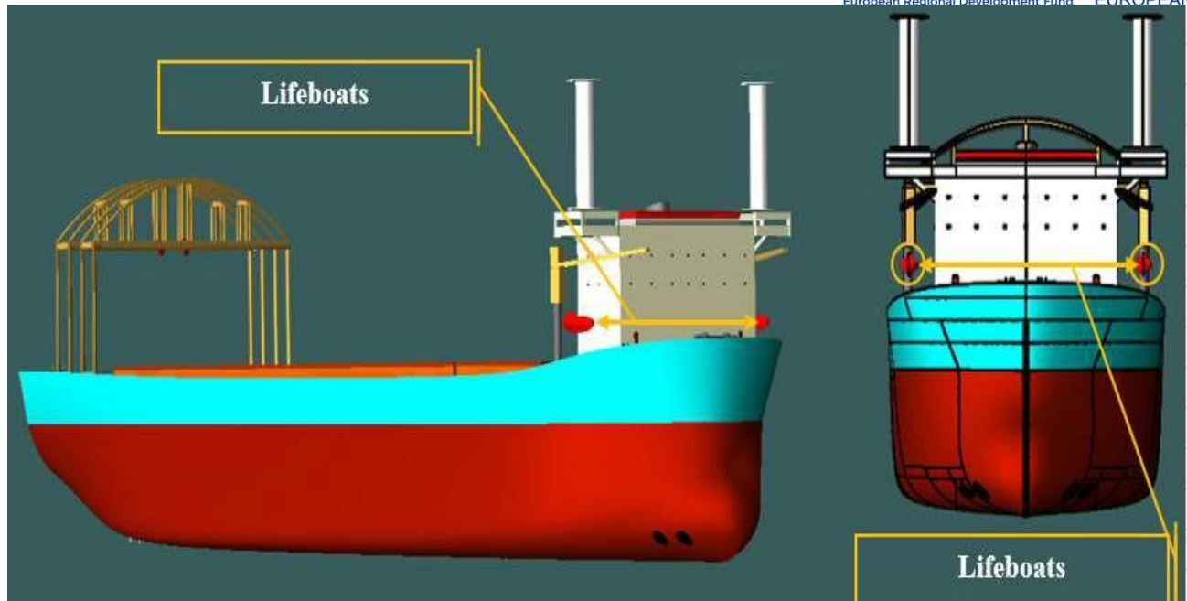
Figure 5-85 Perspective and Front (Bow) View of Lifeboats
