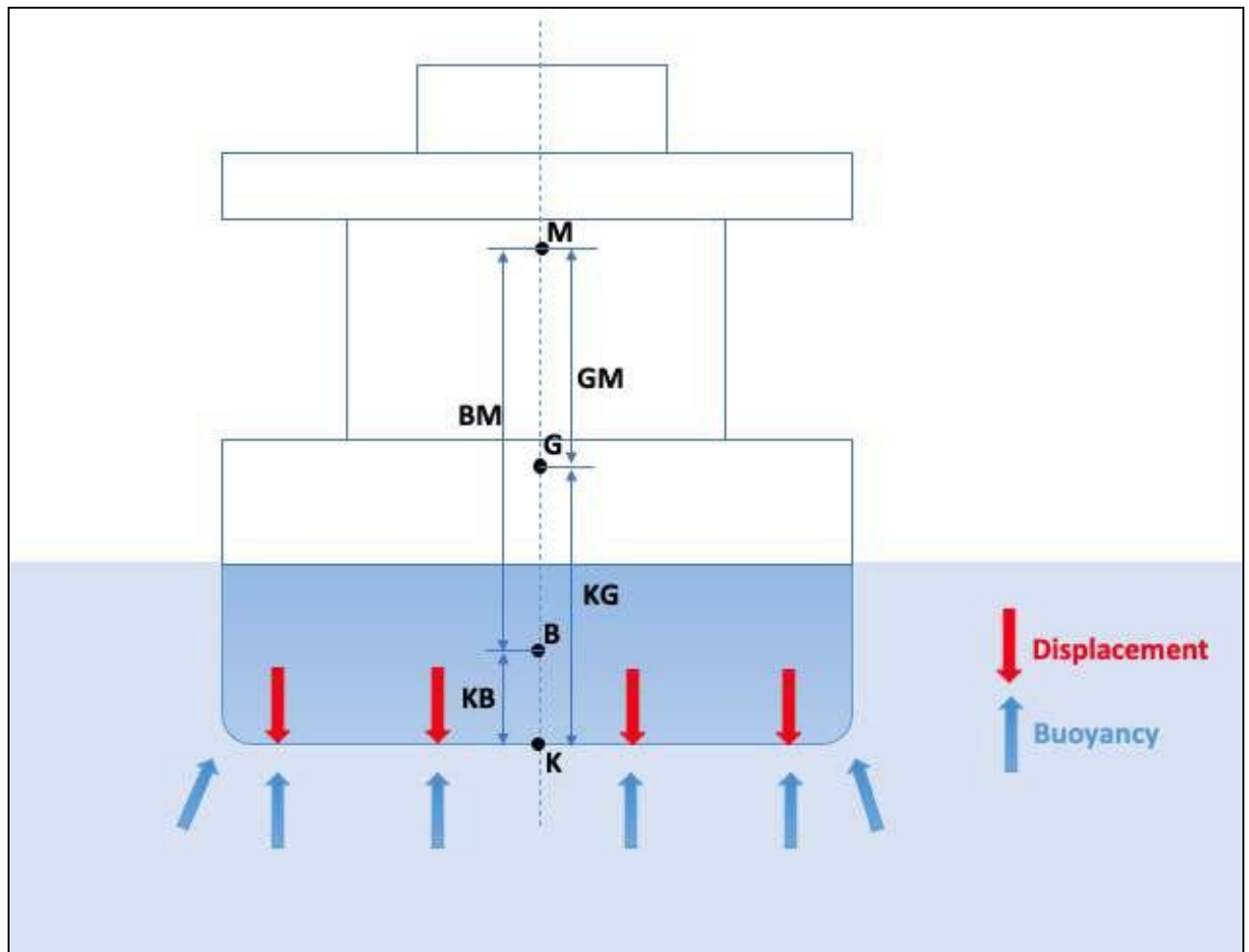
Figure 7-8 Displaying the M, GM, BM, B, KB & K
