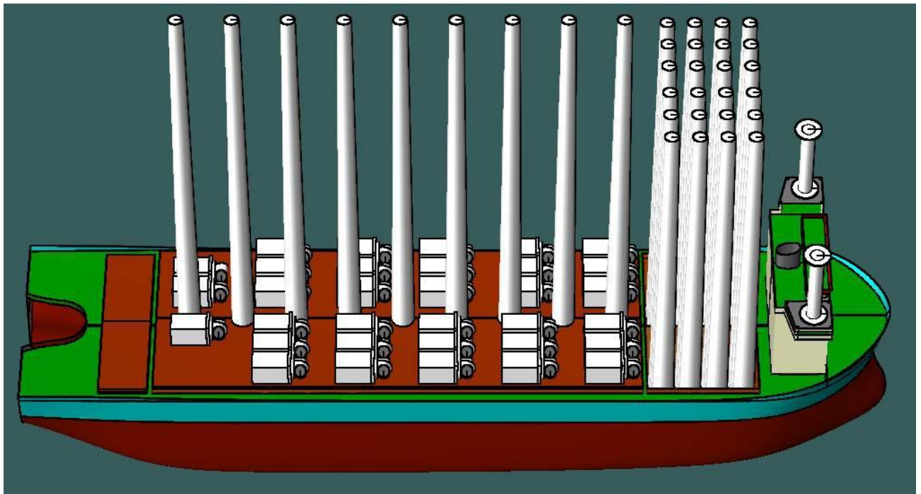
Figure 7-37 33 Sets of 3.6 MW WT Loaded on the Decom Tools Vessel
