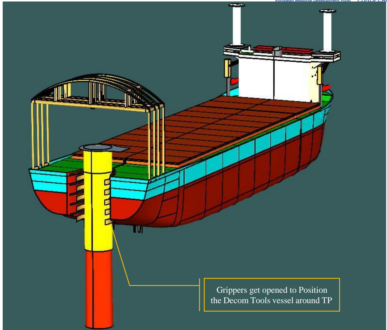
Figure 6-94 Positioning the TP Inside the Grippers
