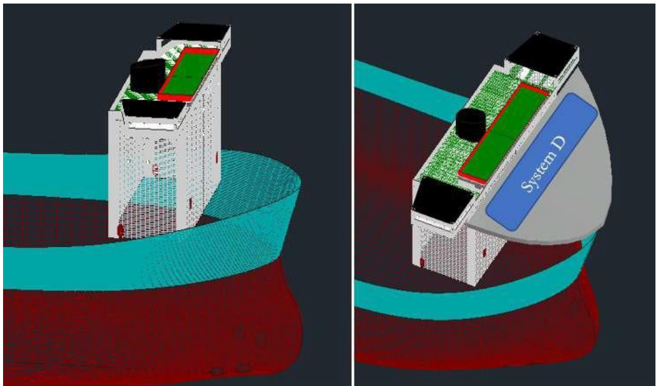
Figure 5-55 Location of Solar Panel on Decom Tools Vessel (System D)
