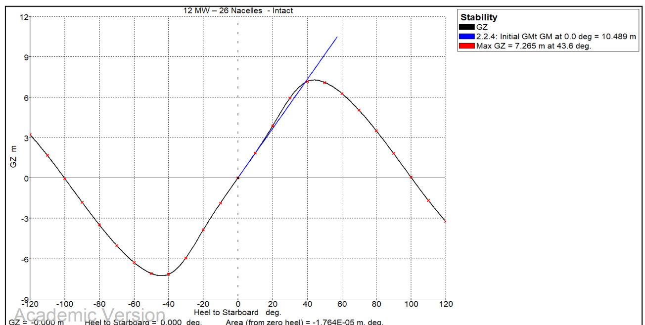
Figure 7-32 GZ Curve after Loading 26 numbers of 12MW Nacelle
