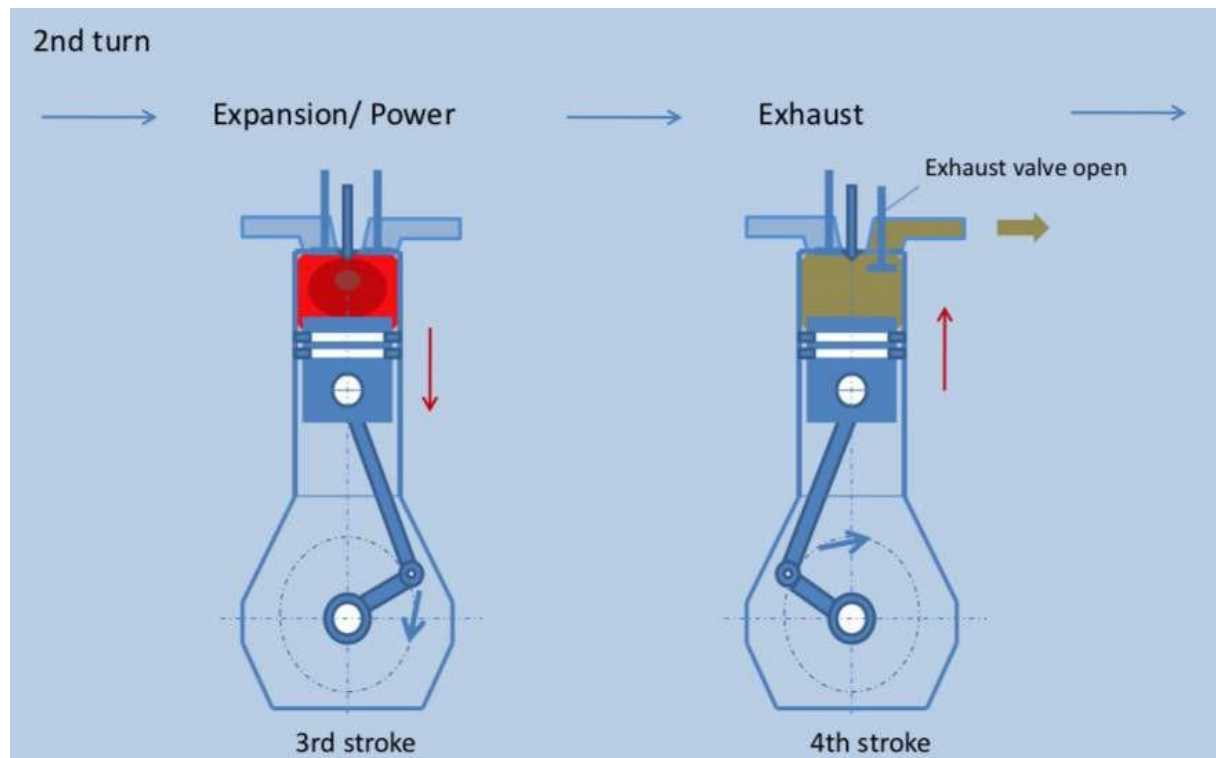
Figure 4-4 Third and Fourth Stroke of 4-Stroke Engine
