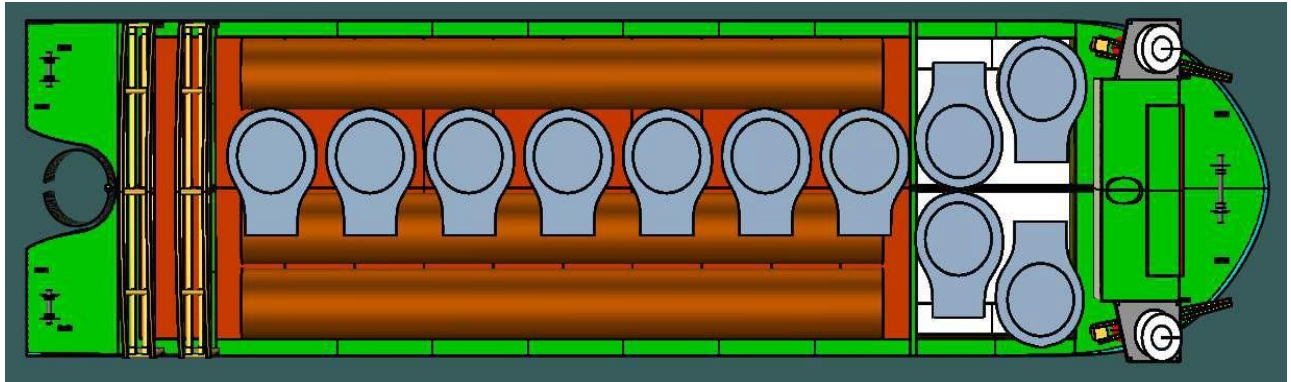
Figure 6-30 Top view of Load out of 12MW TP & Monopile (First Arrangement)
