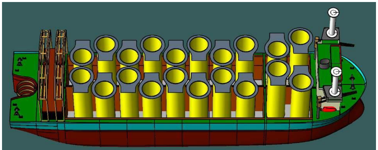
Figure 6-45 Top View of Load of 12MW TP with Decom Tools Vessel
