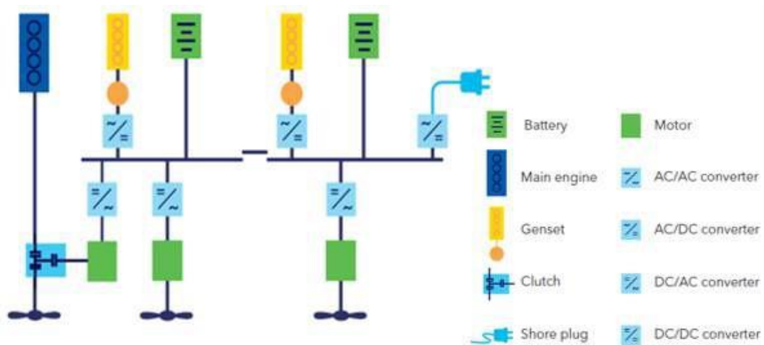
Figure 4-34 Hybrid Battery, Electrical, Mechanical Propulsion & DC Distribution
