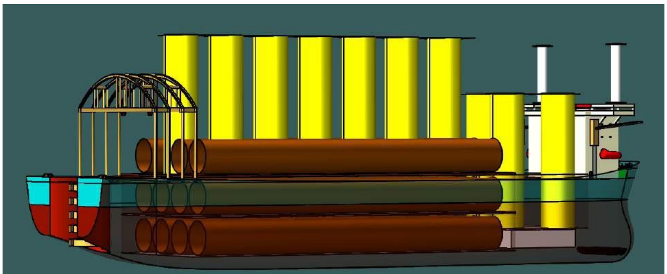
Figure 6-32 Perspective of Load out of 12MW TP & Monopile (First Arrangement)
