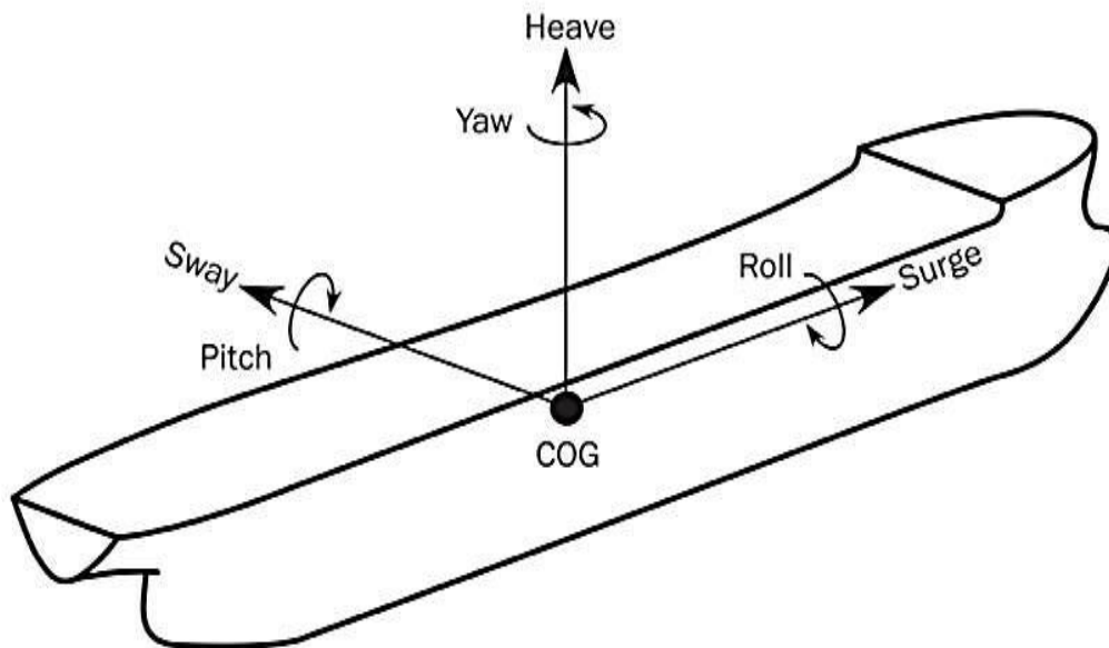
Figure 8-1 Motions of a Floating Vessel
