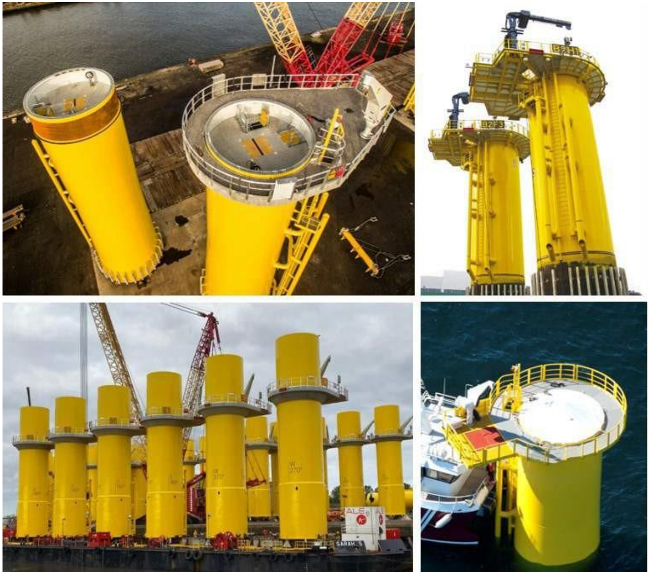
Figure 6-88 Different Design of Transition Pieces
