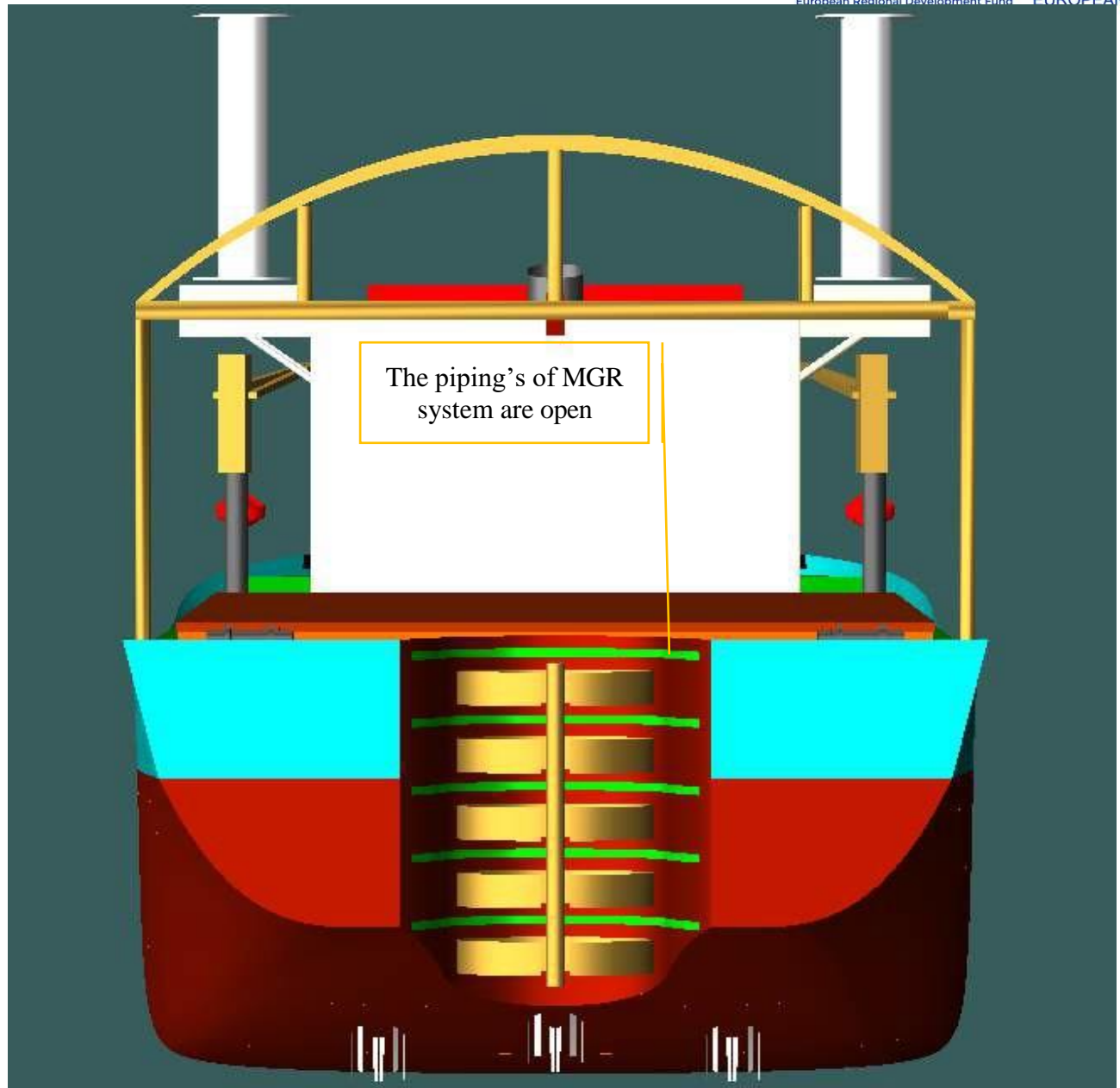
Figure 6-158 The Marine Growth System (In green colour)
