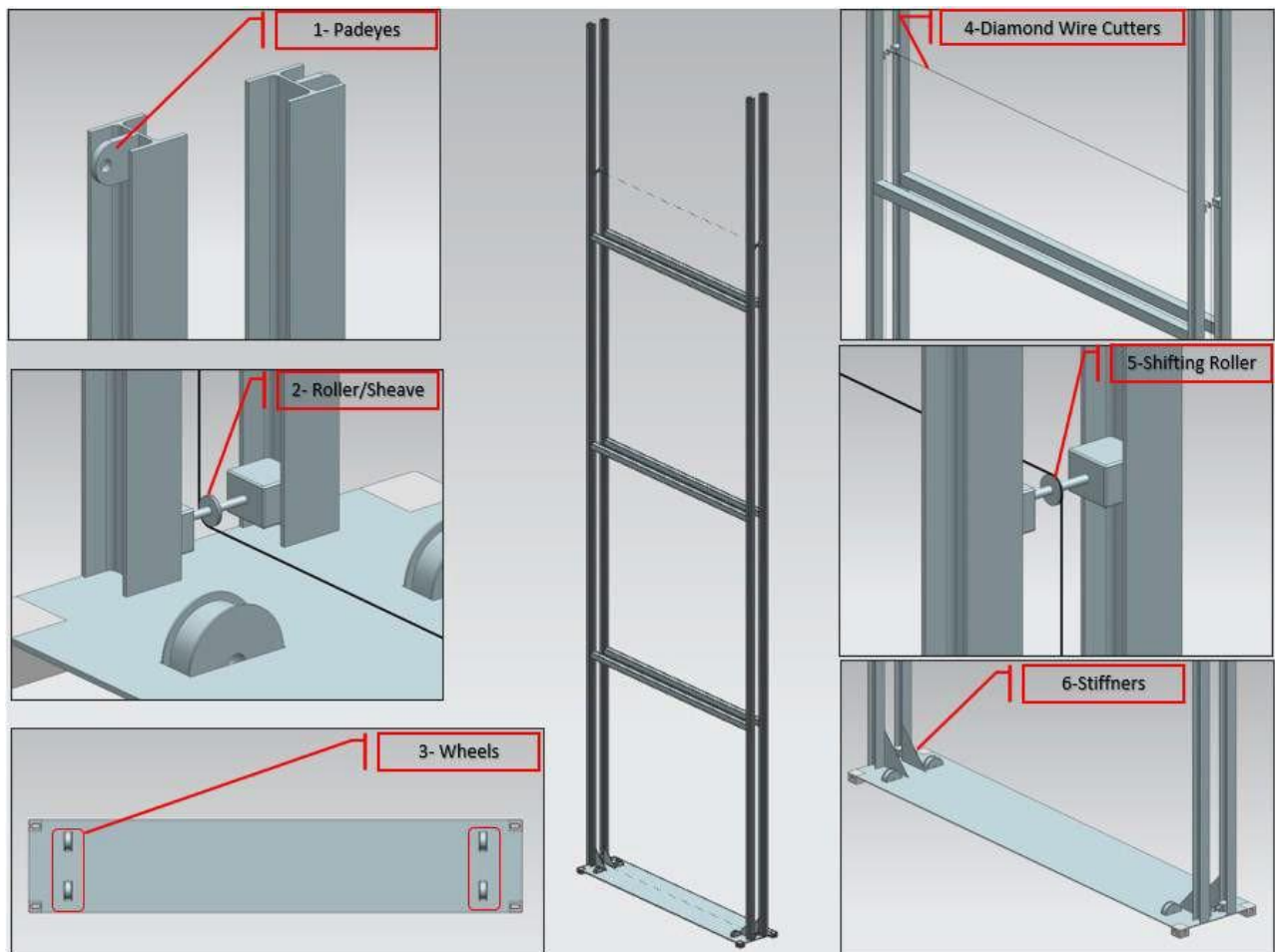
Figure 6-73 Details of Blade Cutting Tool
