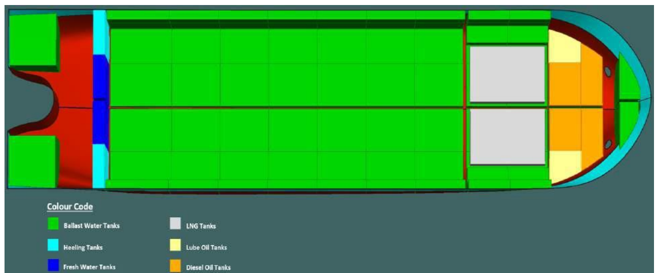
Figure 7-9 Plan of Tanks of Decom Tools Vessel
