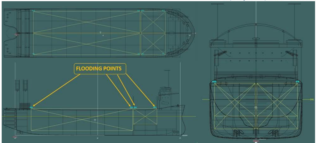
Figure 7-19 Flooding Point of the Decom Tools Vessel
