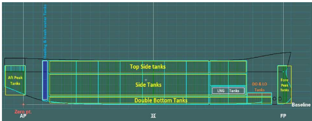
Figure 5-21 Side View of Decom Tools Vessel's Tanks
