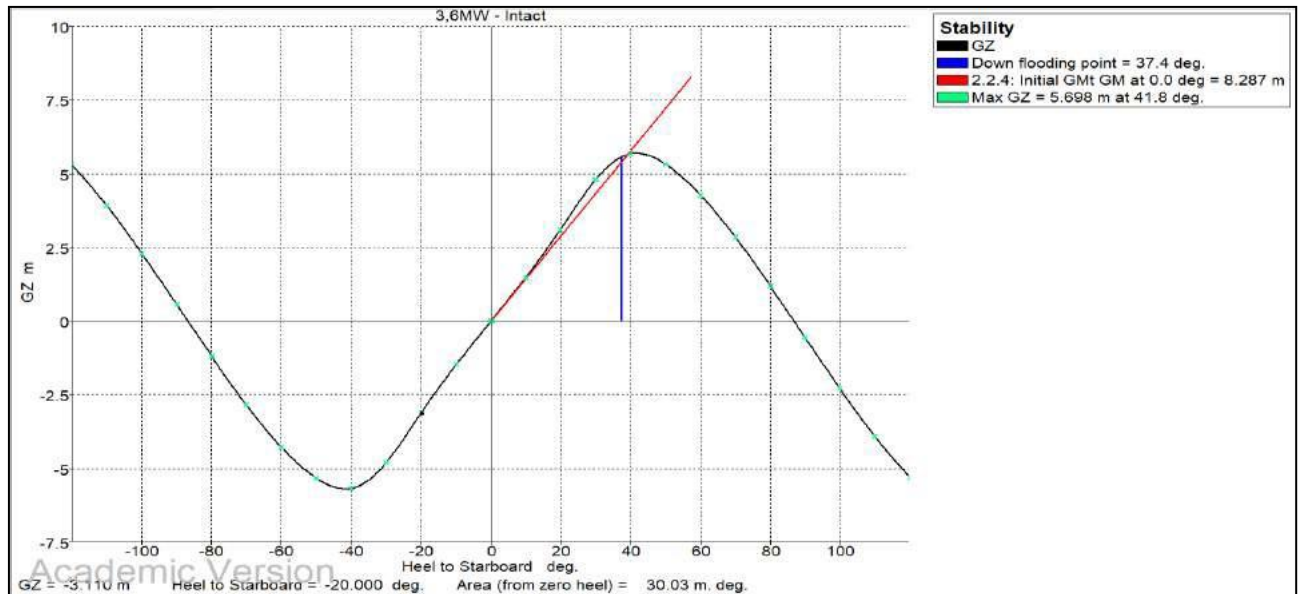
Figure 7-38 GZ Curve after Loading 33 sets of 3.6MW Wind Turbine
