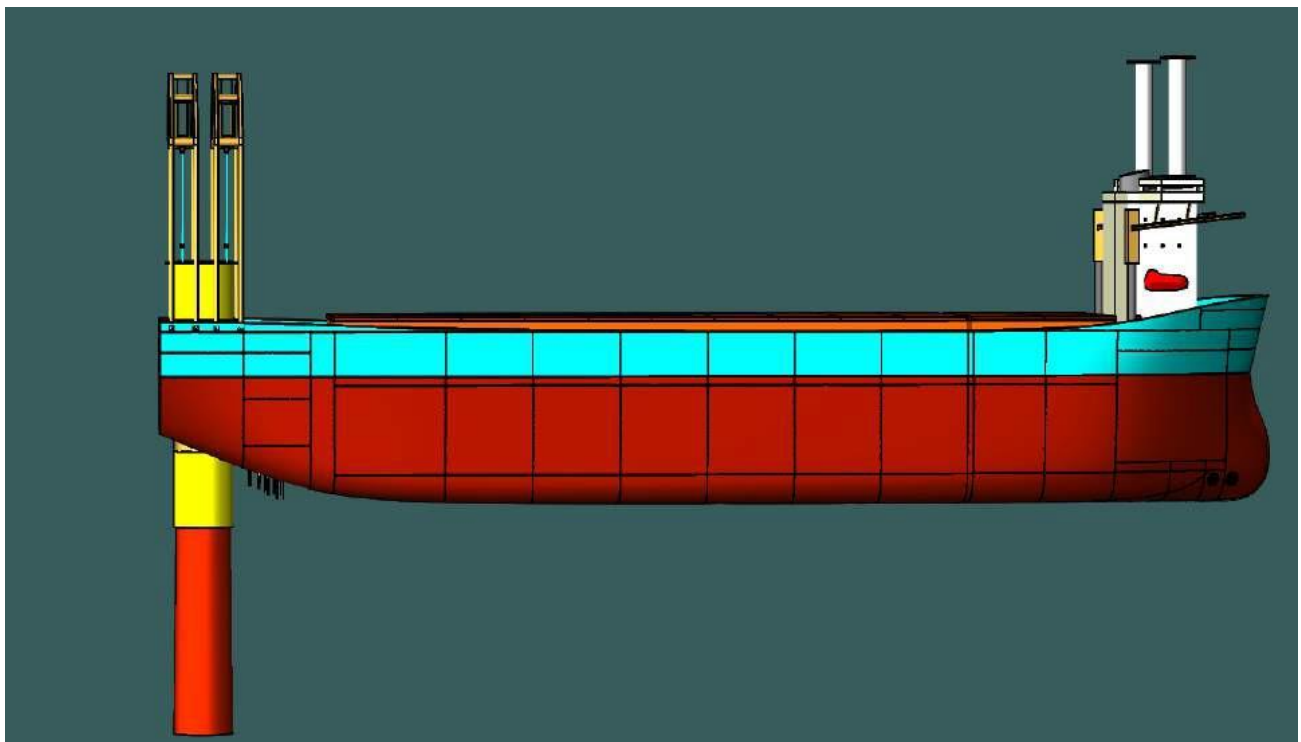
Figure 6-97 Transition Piece are rigged to both gantry cranes (Side view)
