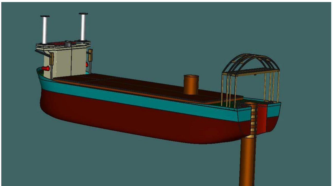
Figure 6-154 The Cut Section is Transferred for further relocation
