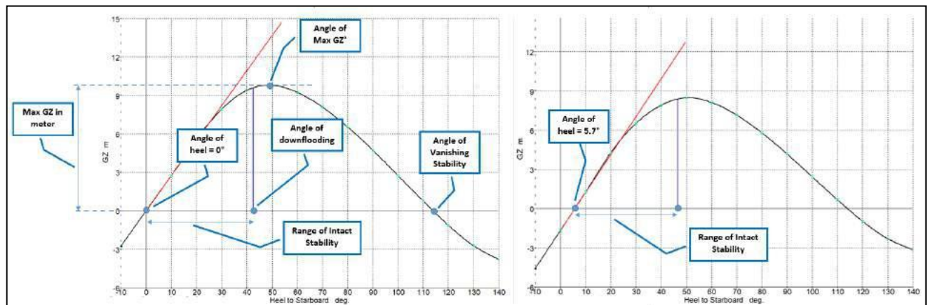
Figure 7-17 GZ Curve for Upright and Heeled Decom Tools Vessel
