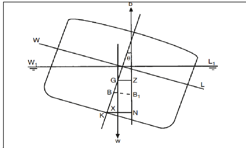
Figure 7-16 Heeled Vessel Due to External Loads (Barrass and Derrett 2006)
