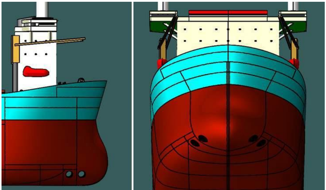
Figure 5-72 Bow Thrusters of Decom Tools Vessel
