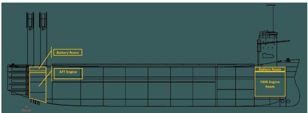
Figure 5-29 Location and Dimension of Engine Rooms
