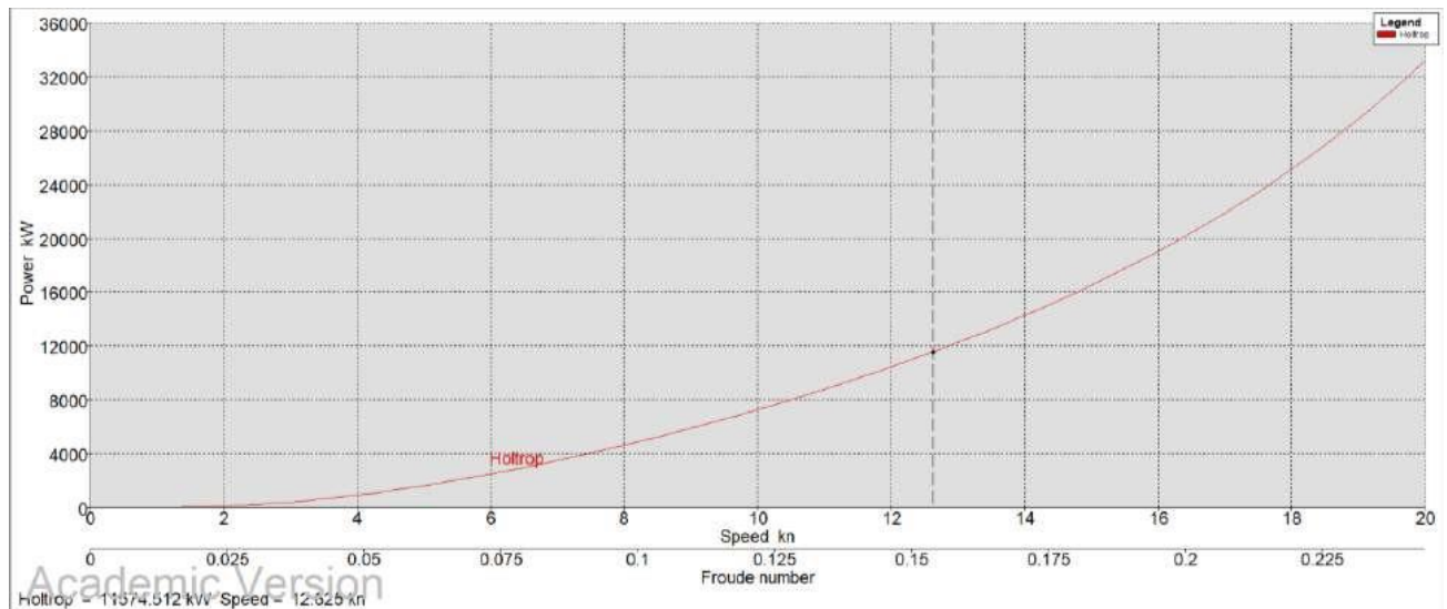
Figure 5-63 Correlation Between Speed and Power at Draft of 6 meters
