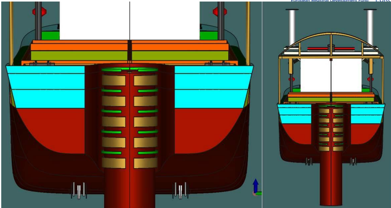
Figure 6-160 Marine Growth Removal Piping's are closed around the monopile
