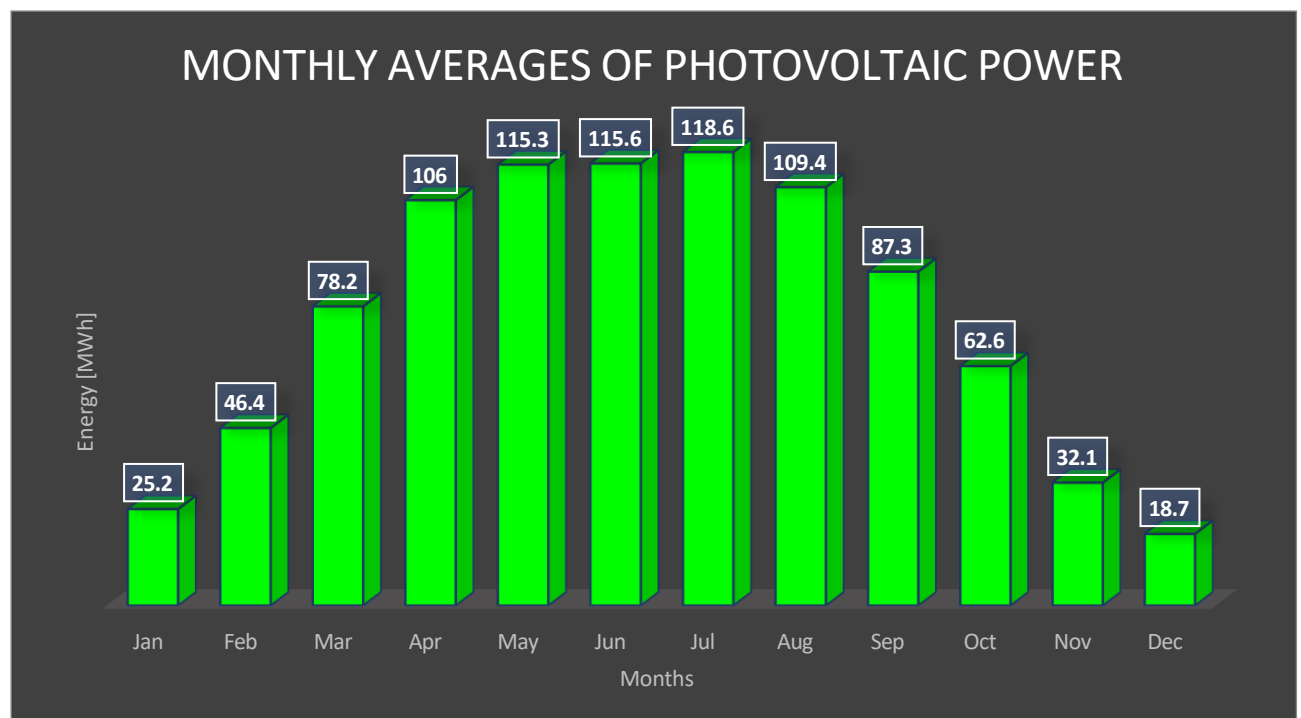
Figure 5-60 Produced Energy by Fixed and Portable Solar Panels During a Year
