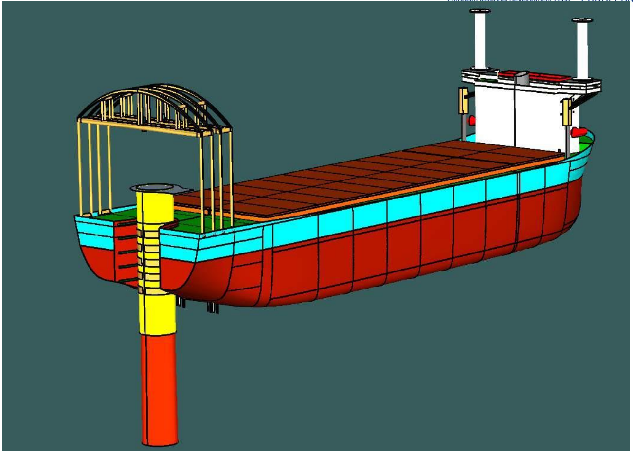
Figure 6-96 Grippers Hold the TP
