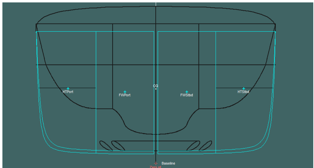
Figure 5-35 Back View of Fresh Water and Heeling Tank
