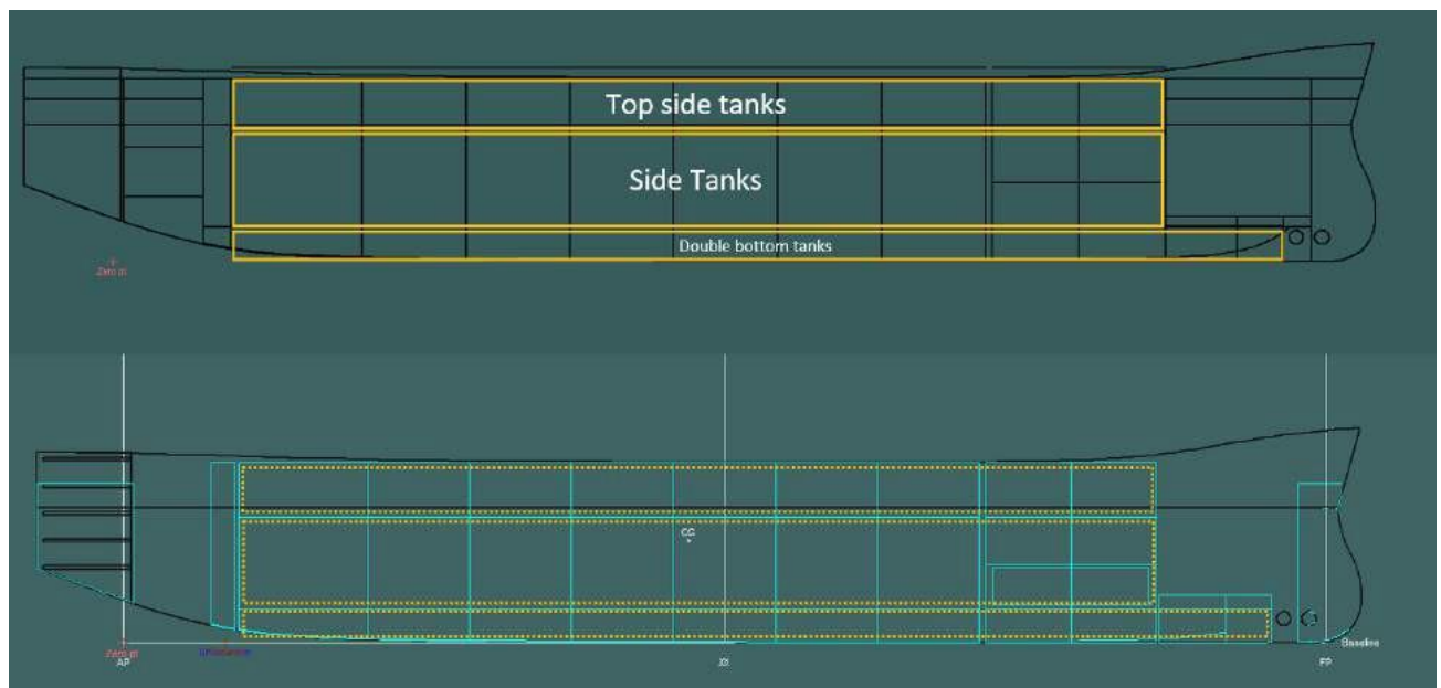
Figure 5-24 Side, Topside and Double Bottom Tanks of Decom Tools Vessel
