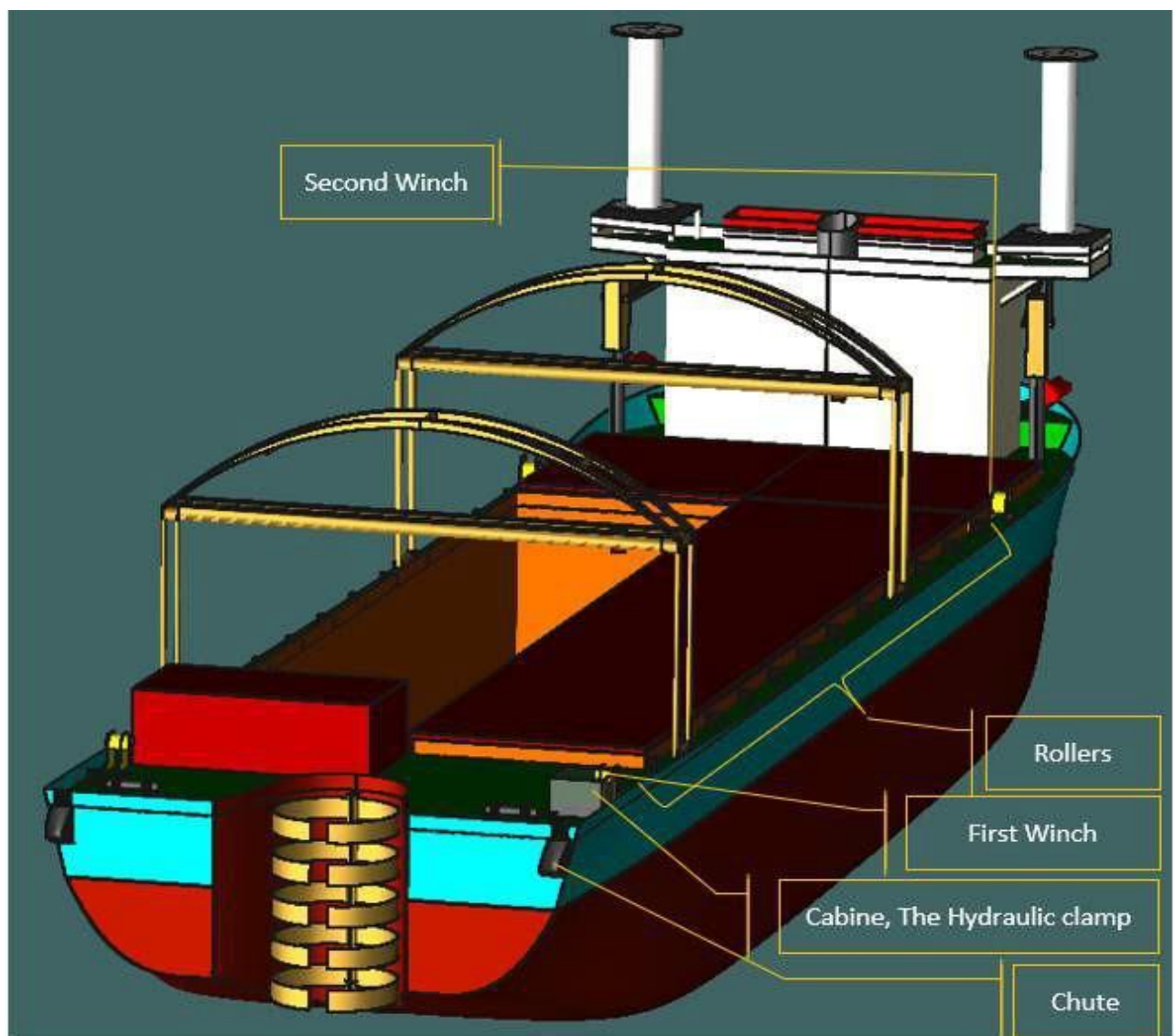
Figure 6-212 Overall View of Decom Tools Vessel & Cable Extraction Tools
