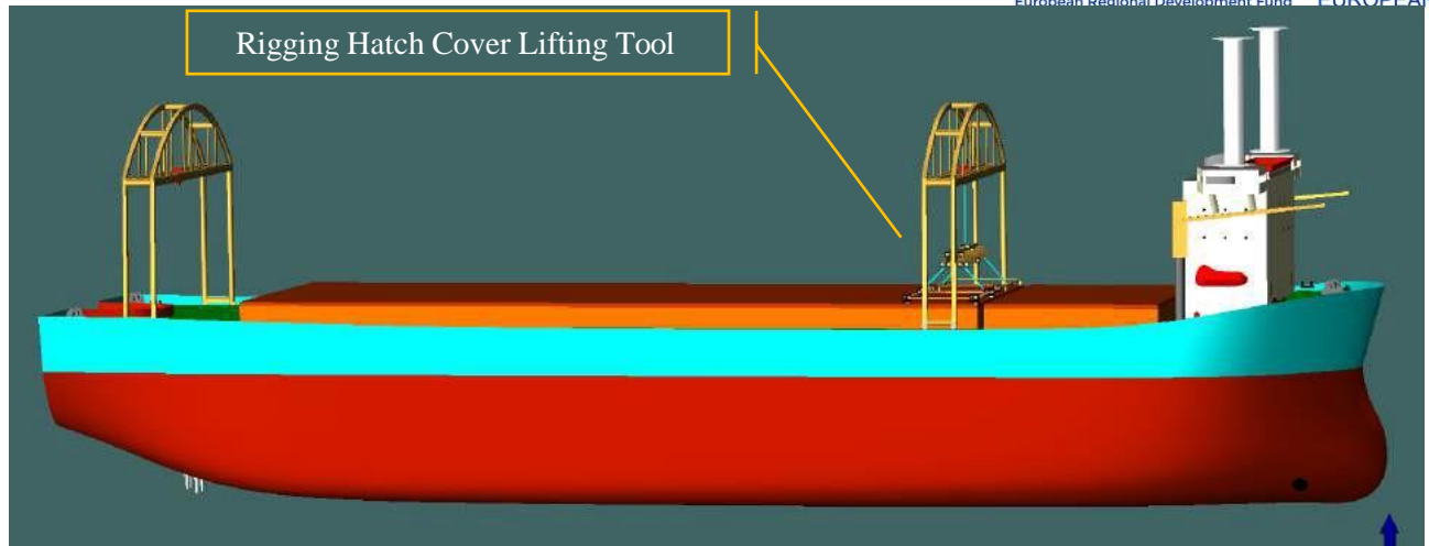
Figure 5-92 Procedure to open the Hatch Cover-Step 1 Rigging Lifting Tool
