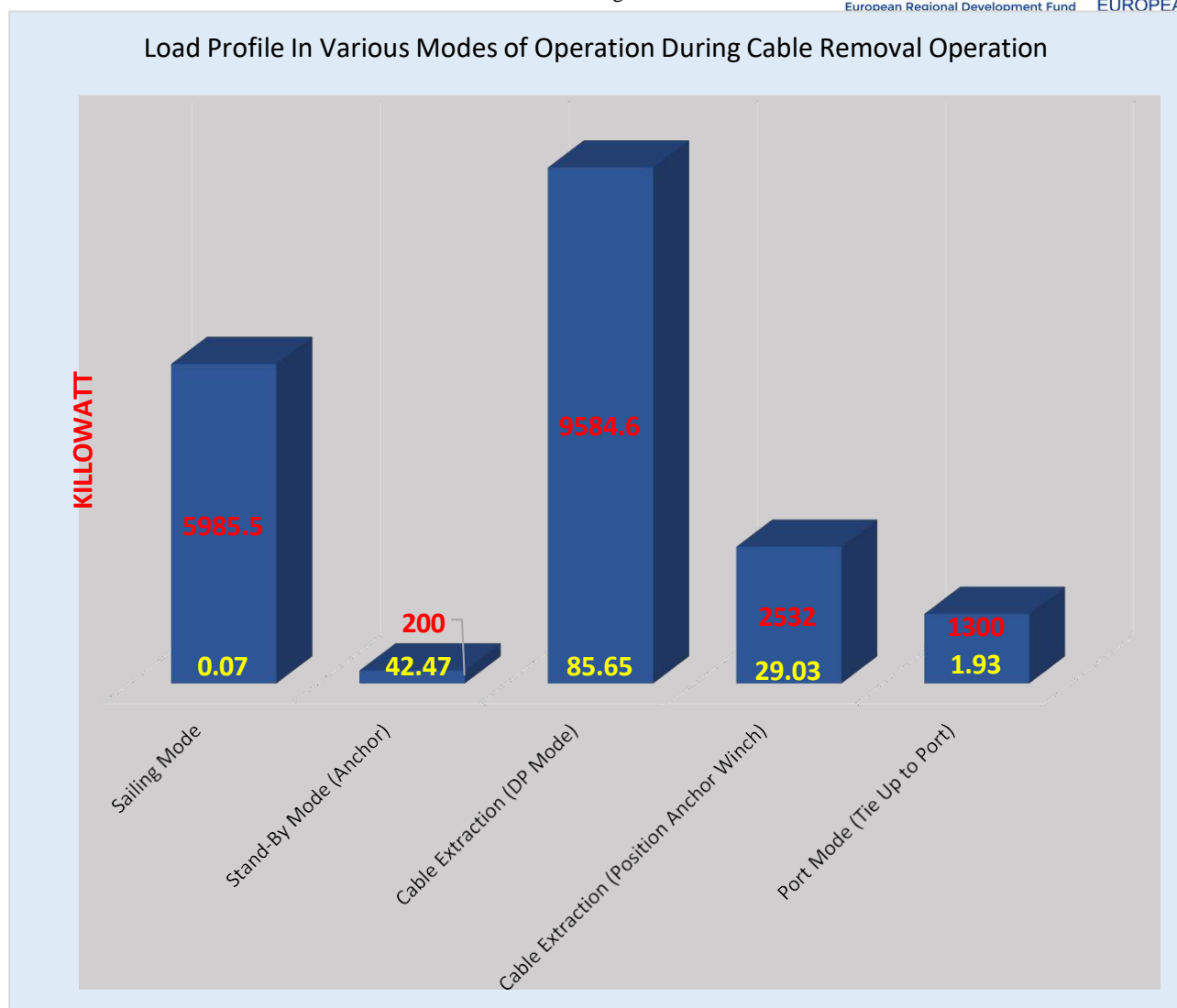
Figure 5-73 Load Profile for Cable Removal Operation
