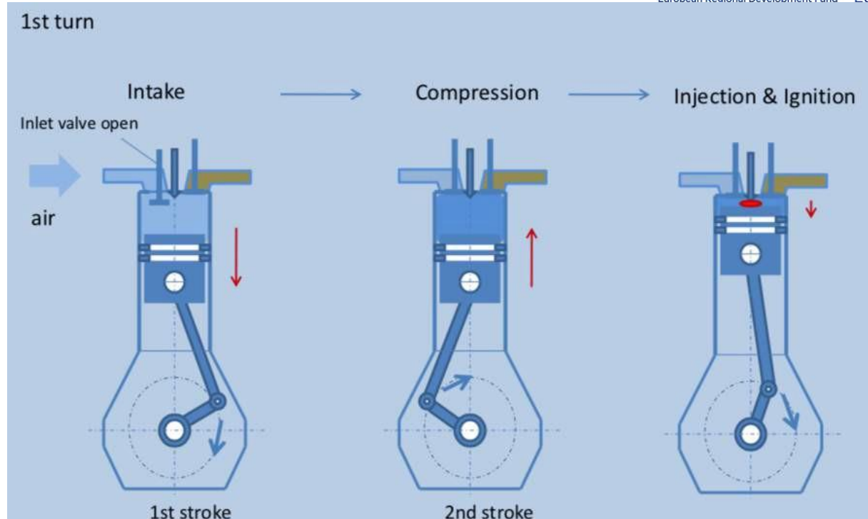
Figure 4-3 First and Second Stroke of 4-Stroke Engine
