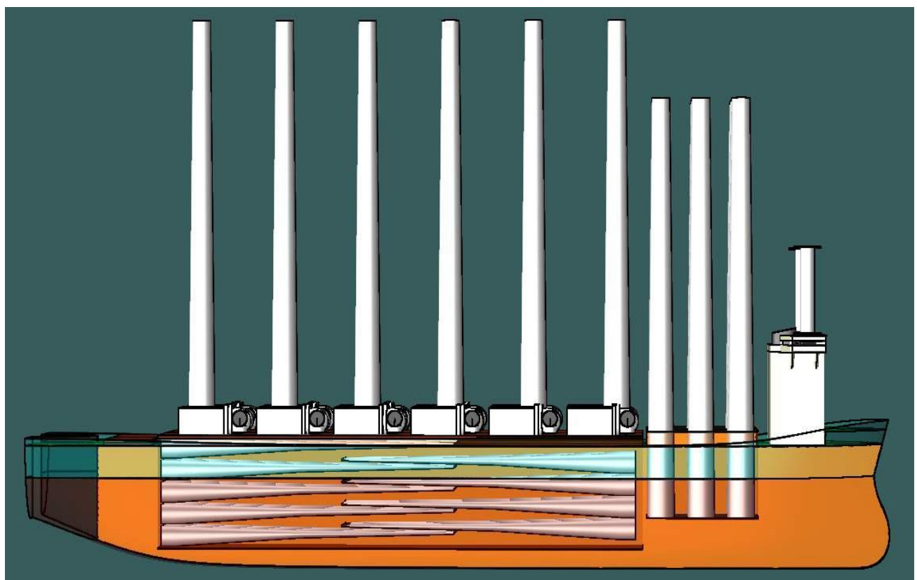
Figure 6-39 Side View of Load out of 5MW Wind Turbine
