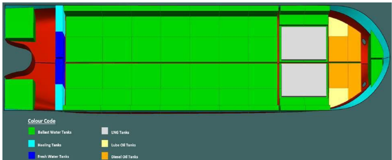
Figure 5-20 Plan of Tanks of Decom Tools Vessel
