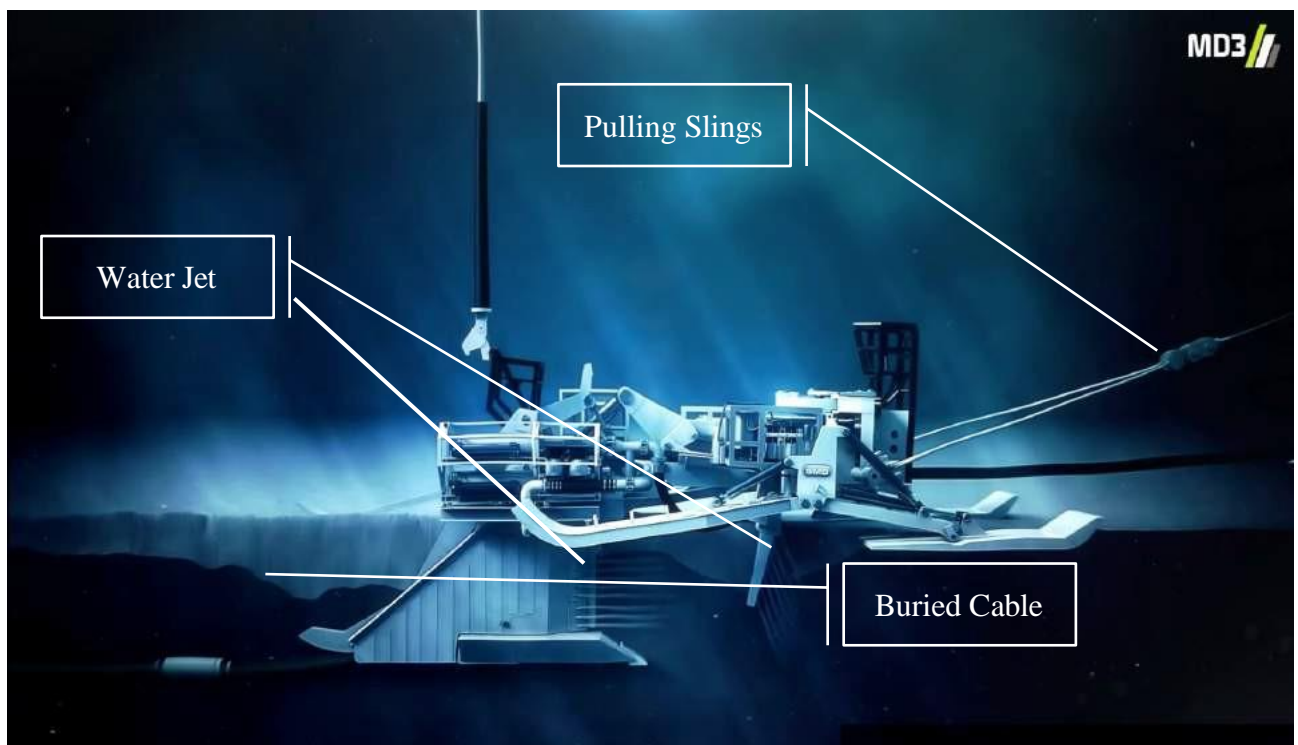
Figure 6-186 Cable Plough (SMD - Subsea Technology 2014)
