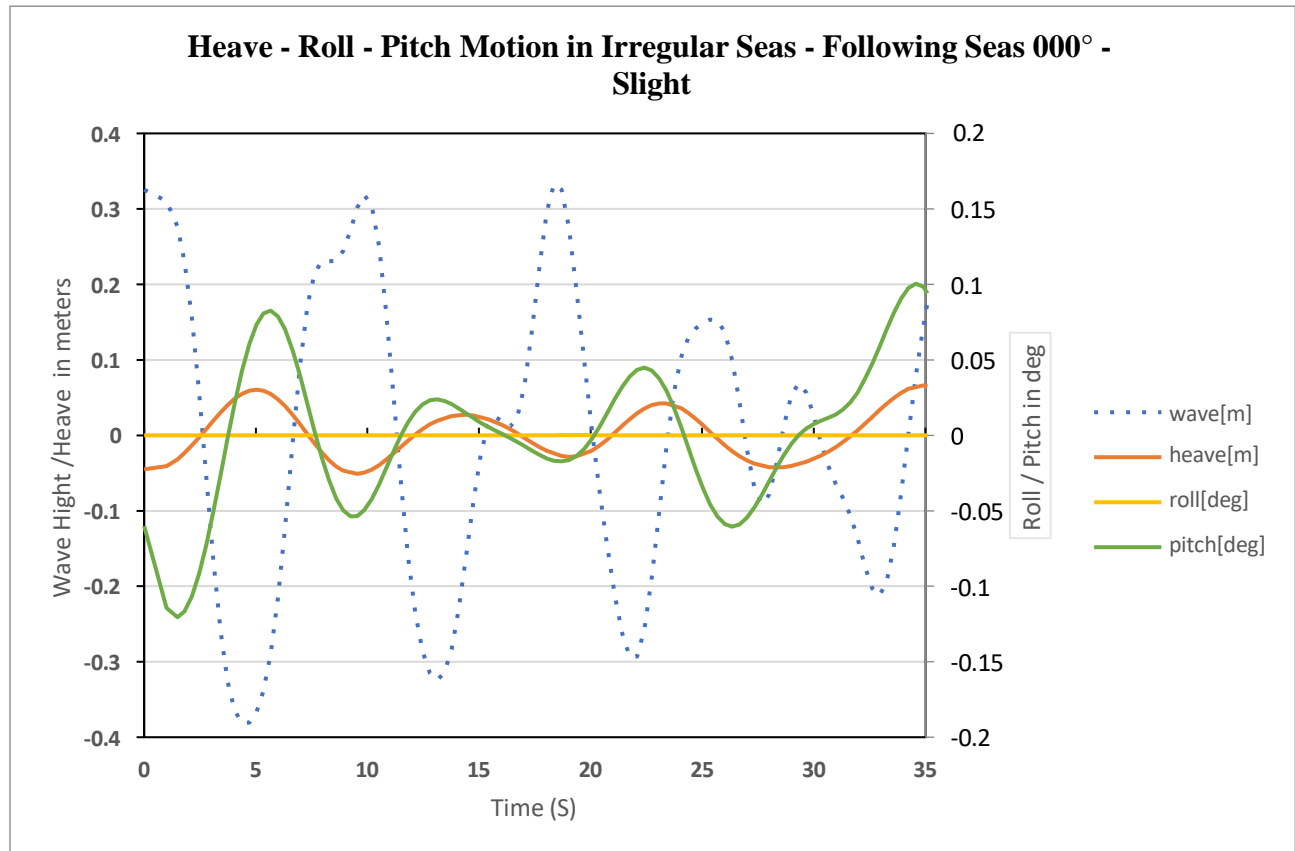
Figure 8-15 Motion in irregular following seas – Slight
