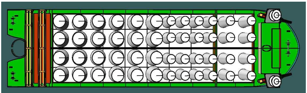
Figure 6-50 Top View of Load of 12MW Tower with Decom Tools Vessel
