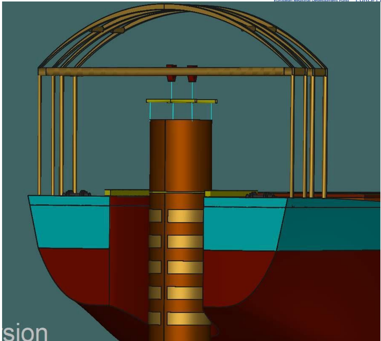
Figure 6-148 Cutting of extracted monopile is in progress with Diamond wire Cutter
