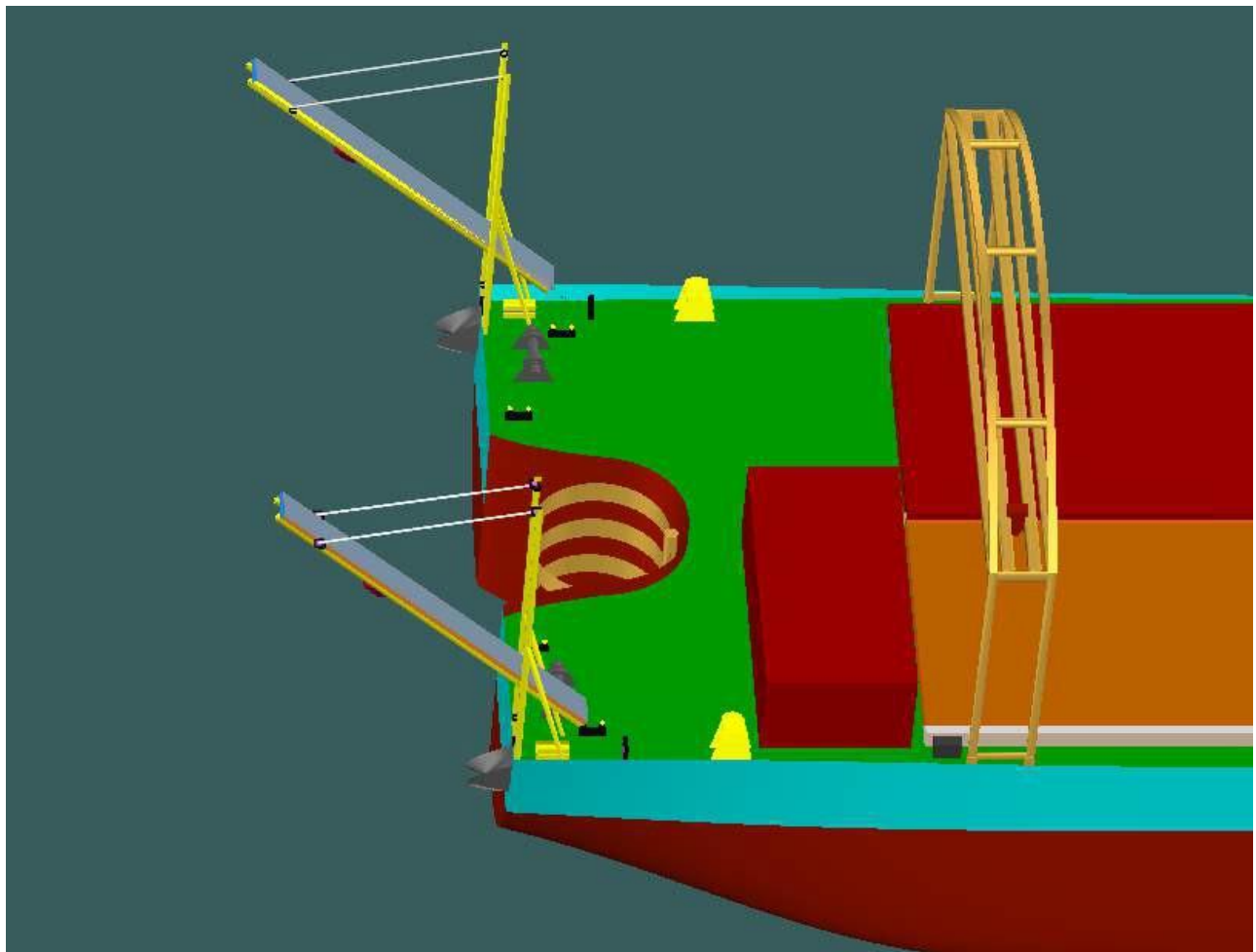
Figure 6-210 Tilting the LARS Structure
