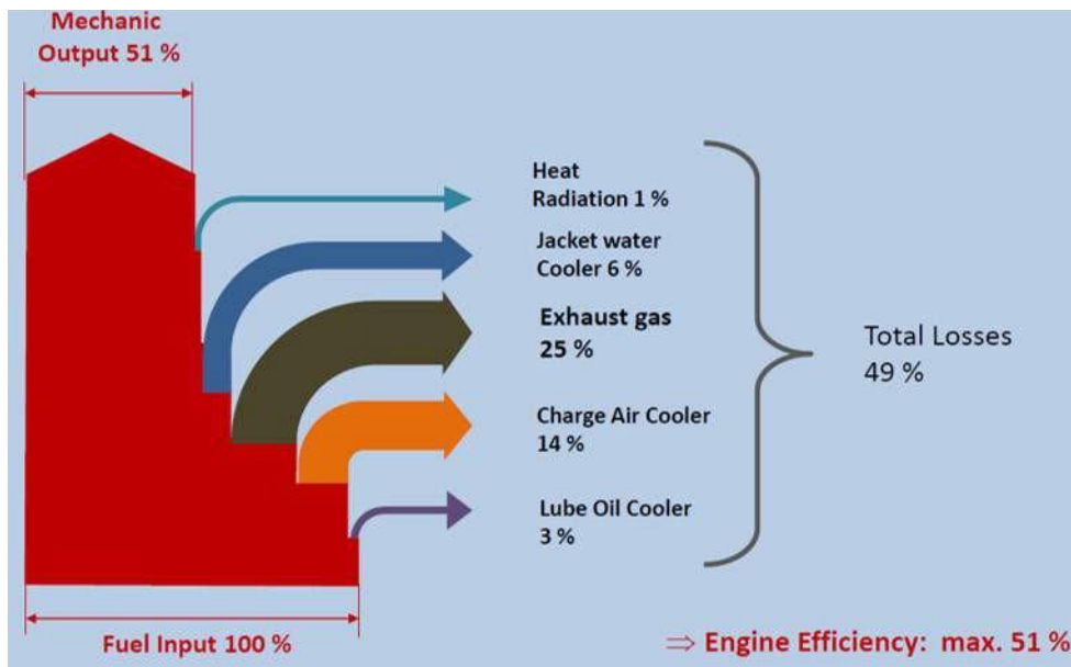
Figure 4-7 Thermal energy balances or Sankey-diagram of 2-Stroke Cross Head Engine (Meyer 2019)
