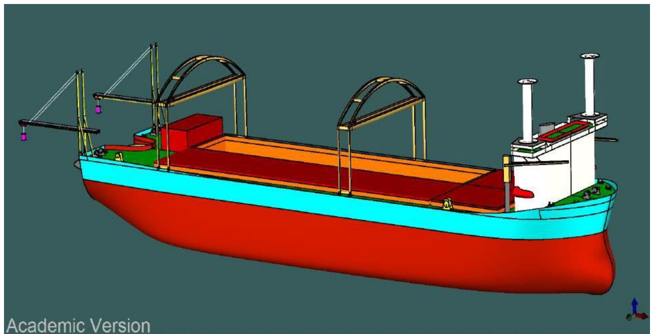
Figure 6-208 Decom Tools LARS Structure (perspective View)
