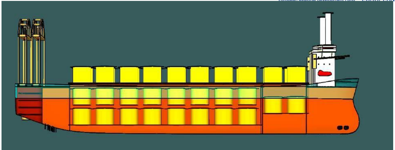
Figure 6-111 TPs loading arrangement (Side View)
