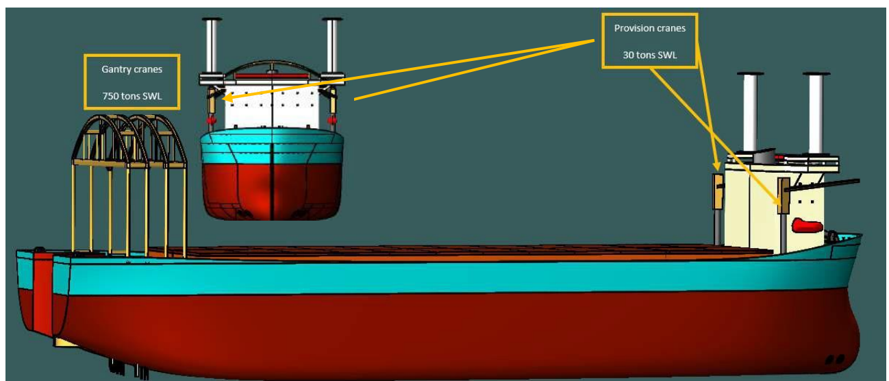
Figure 5-46 Gantry and Provision Pedestal Cranes
