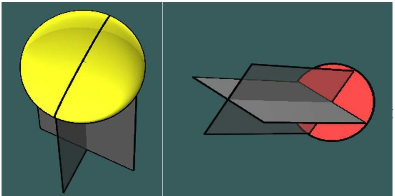
Figure 6-130 Structure to Prevent Pile Collapse (Pile Collapse Preventor)
