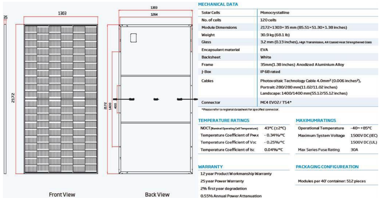
Figure 5-56 Mechanical Specification & Dimension of Trina Vertex Panel (Trina Solar n.d.)
