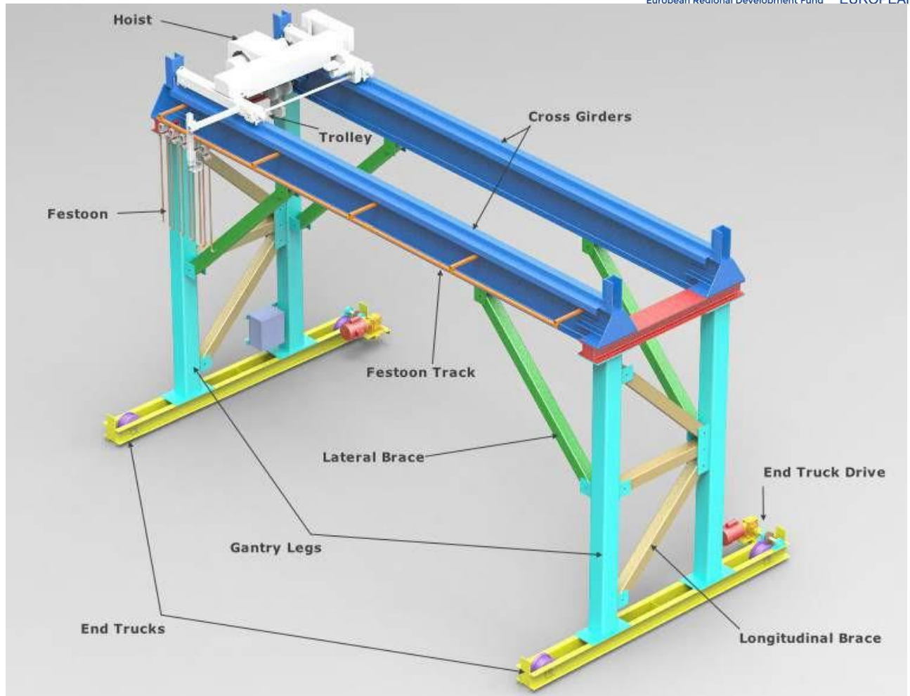
Figure 5-40 Elements of a Gantry Crane (NAICRANES n.d.)
