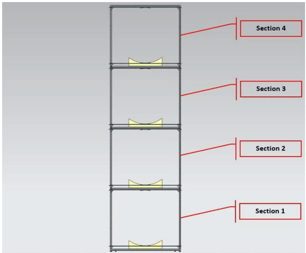
Figure 6-62 One rack for the Seafastening 4 blades (12 MW)
