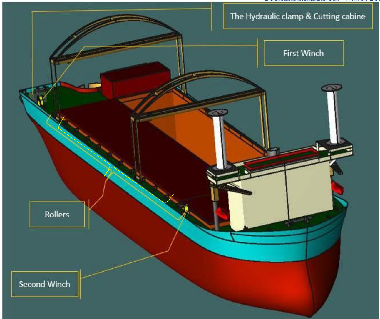
Figure 6-213 Overall View of Decom Tools Vessel & Cable Extraction Tools
