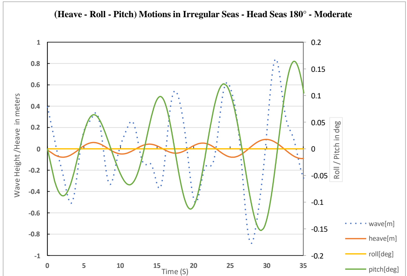
Figure 8-19 Motions in irregular head Seas – Moderate
