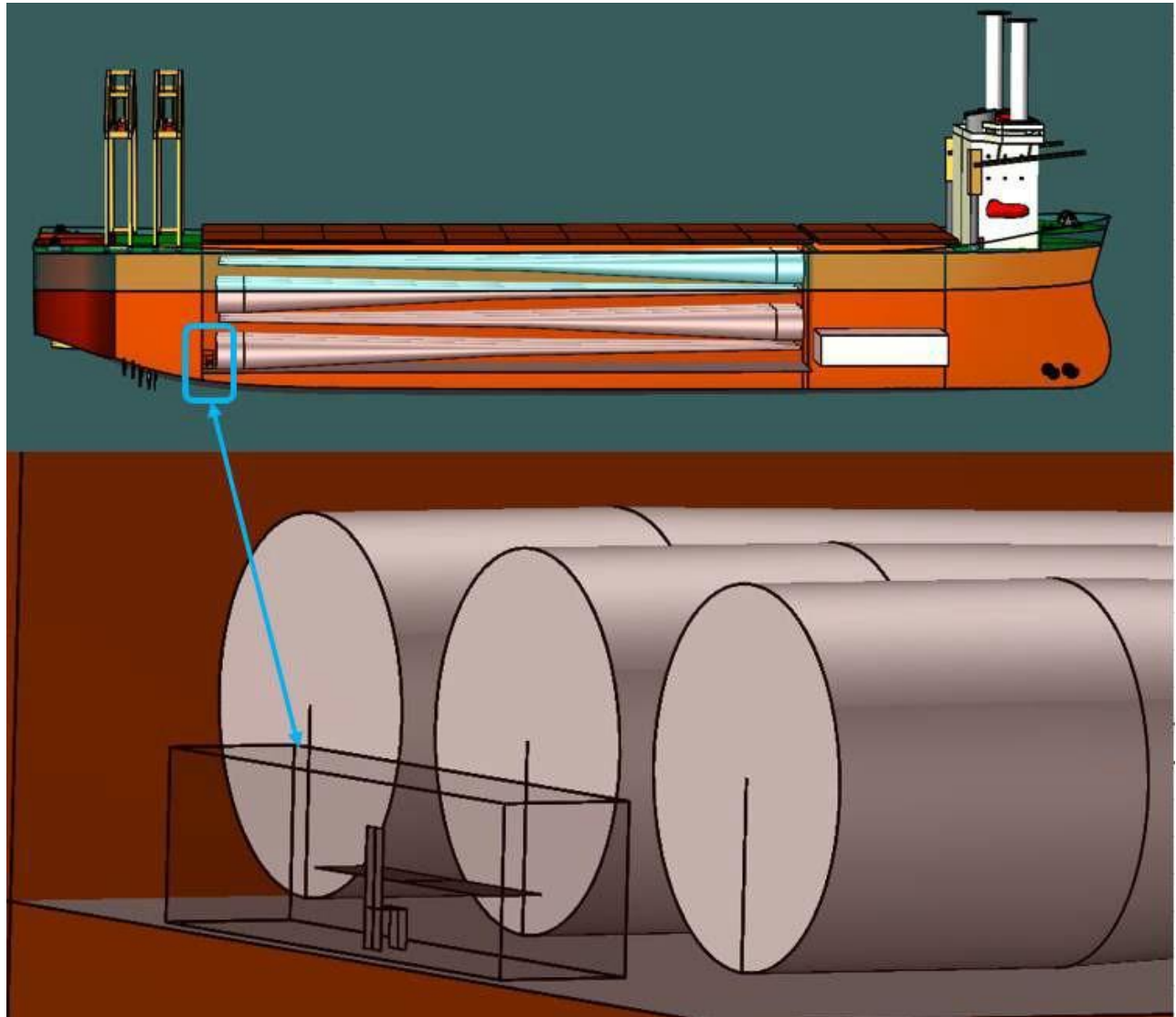
Figure 6-86 The Portable Cabin for Operator for Cutting
