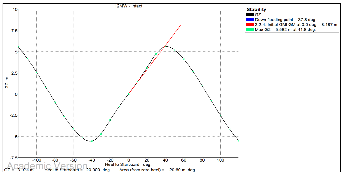
Figure 7-23 GZ Curve Departure Condition While Loading 8x12MW WT
