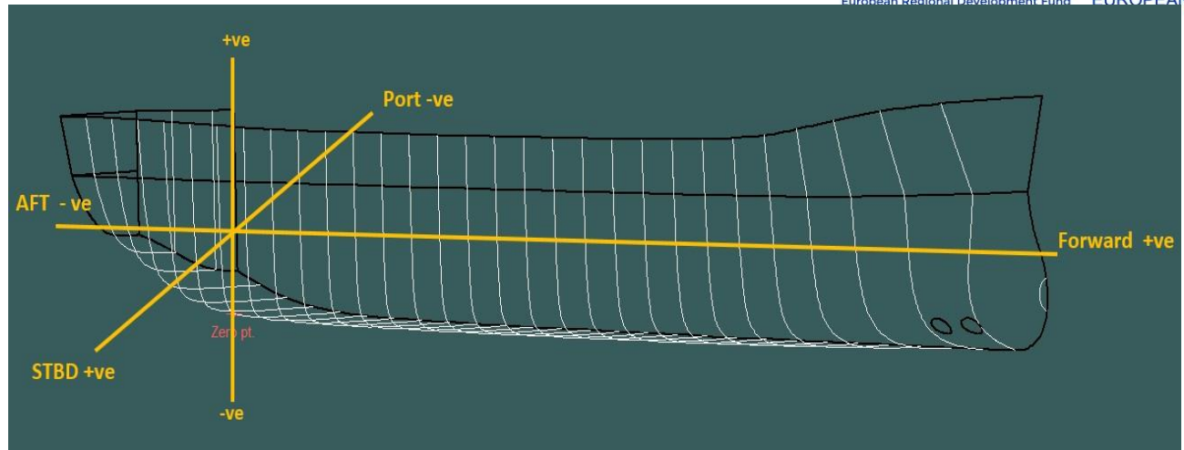
Figure 7-2 Direction and Coordinate of the Vessel
