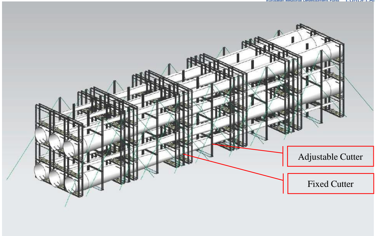
Figure 6-75 12 MW blades inside the racks (Ready for cutting)
