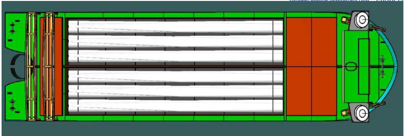
Figure 6-22 Top view of Load out of 12 MW Blades inside the holds
