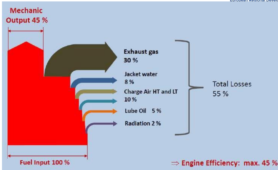
Figure 4-6 Thermal energy balances or Sankey-diagram of 4-Stroke Cross Head Engine (Meyer 2019)
