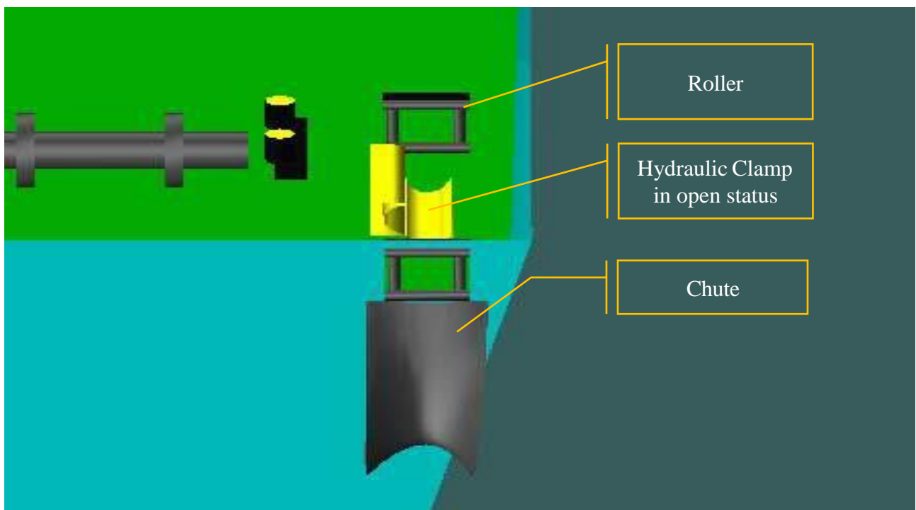
Figure 6-216 Chute, Hydraulic Clamp and Rollers
