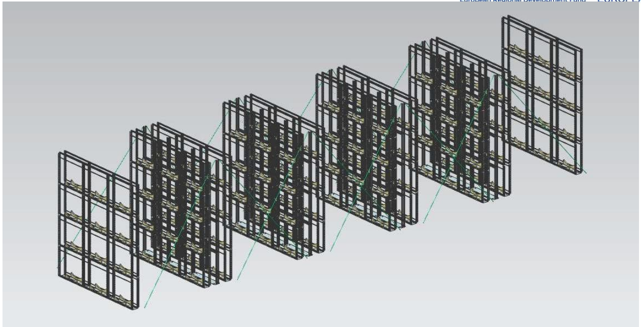
Figure 6-61 Blade's Seafastening of the Decom Tools Vessel
