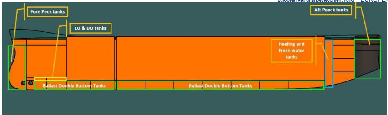
Figure 5-22 Side View of Decom Tools Vessel's Tanks
