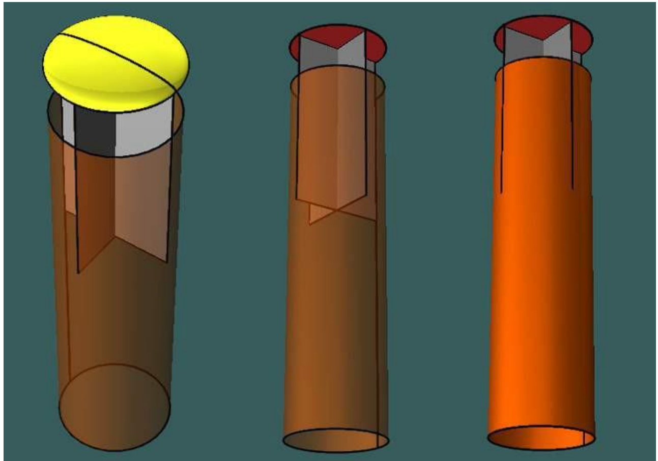
Figure 6-131 Different Views of Pile Collapse Preventer Inside Monopile
