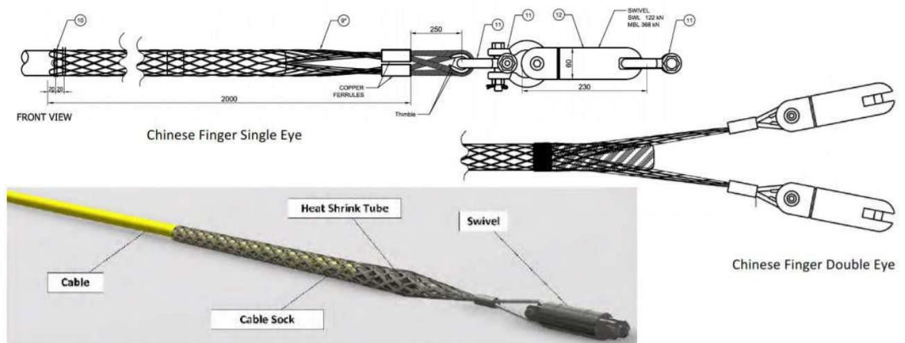
Figure 6-199 Chinese Finger and Drawing of Connection
