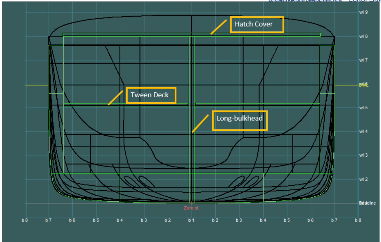
Figure 5-12 Aft View of Decom Tools Vessel's Deck
