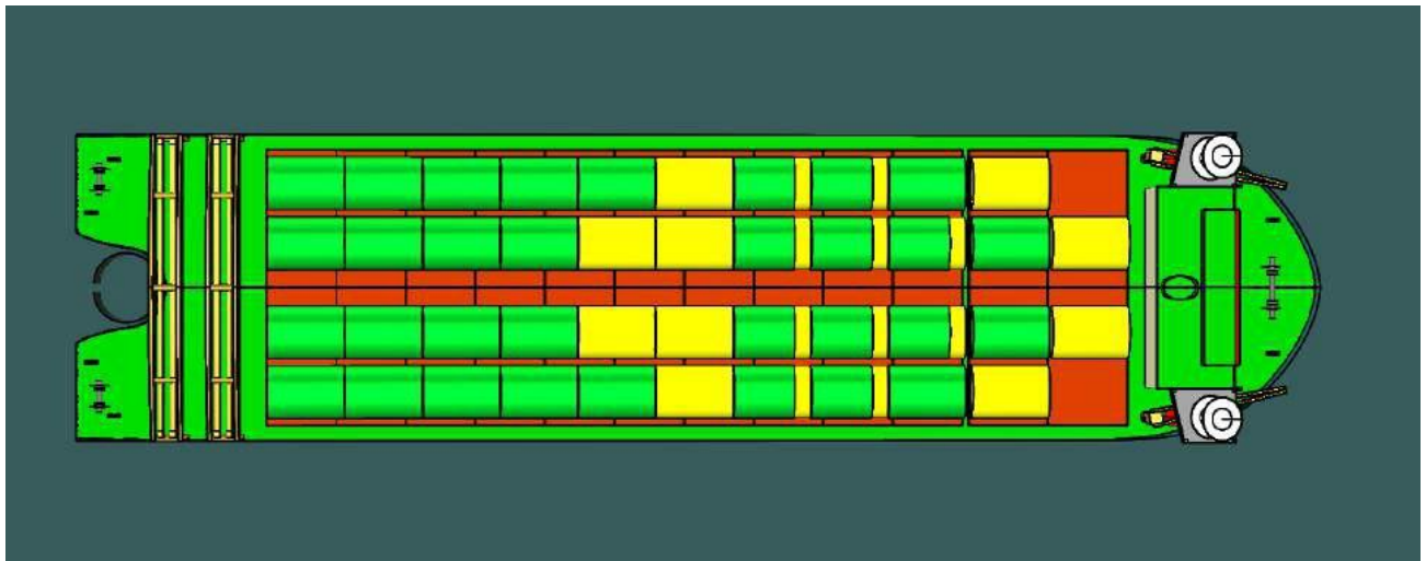
Figure 6-167 Load out of 24 Numbers of MP plus TP (Plan View)
