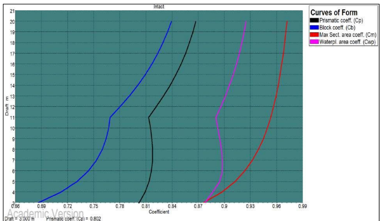
Figure 7-14 Curves of Form with Respect to Various Draft
