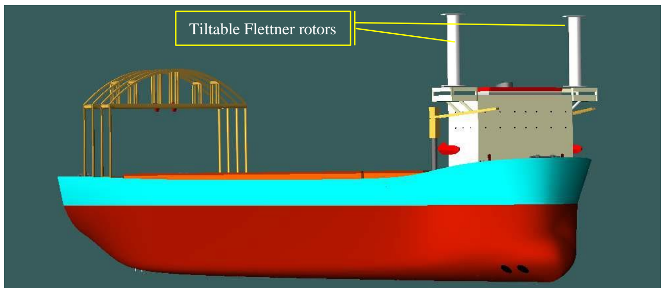
Figure 5-50 Perspective View of Flettner Rotors
