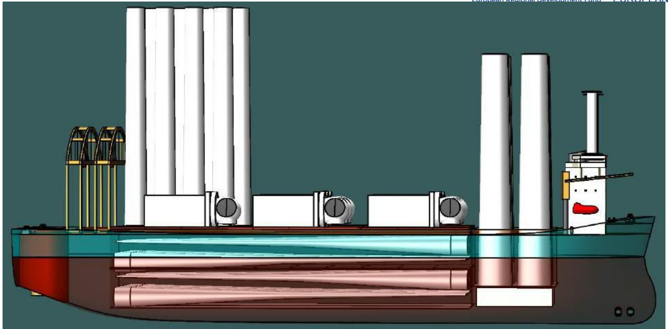
Figure 6-28 Side View of Load out of 12MW Blades, Nacelle & Tower
