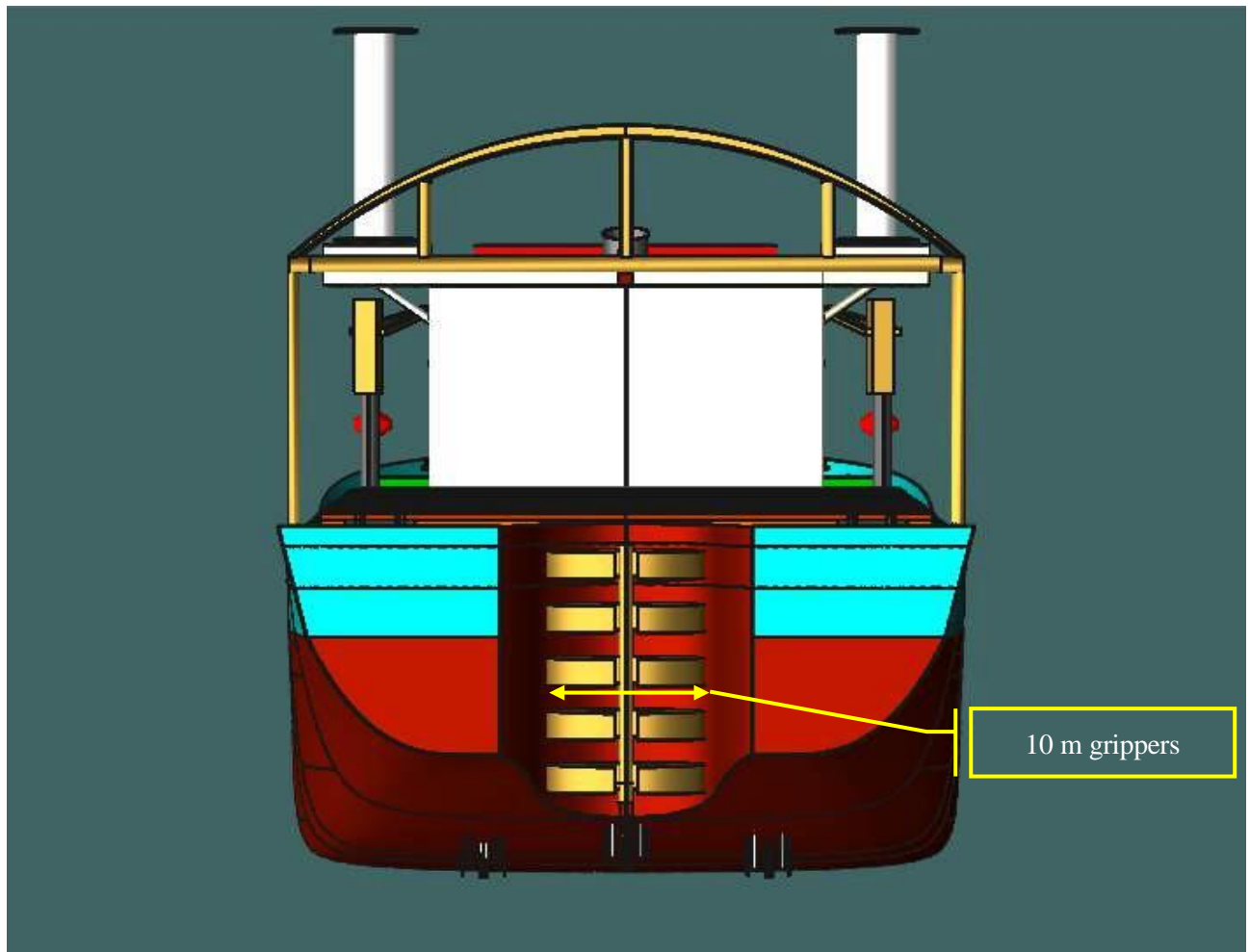
Figure 6-124 Dimension of Grippers
