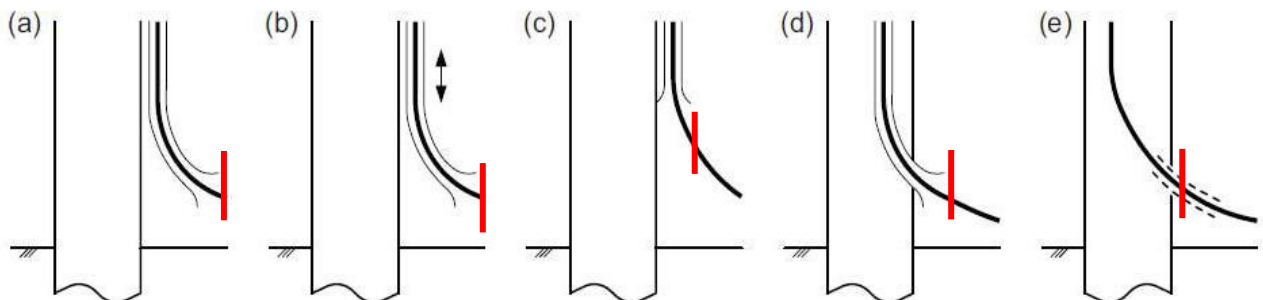
Figure 6-221 Different Types of J/I tube (DNV.GL 2016)
