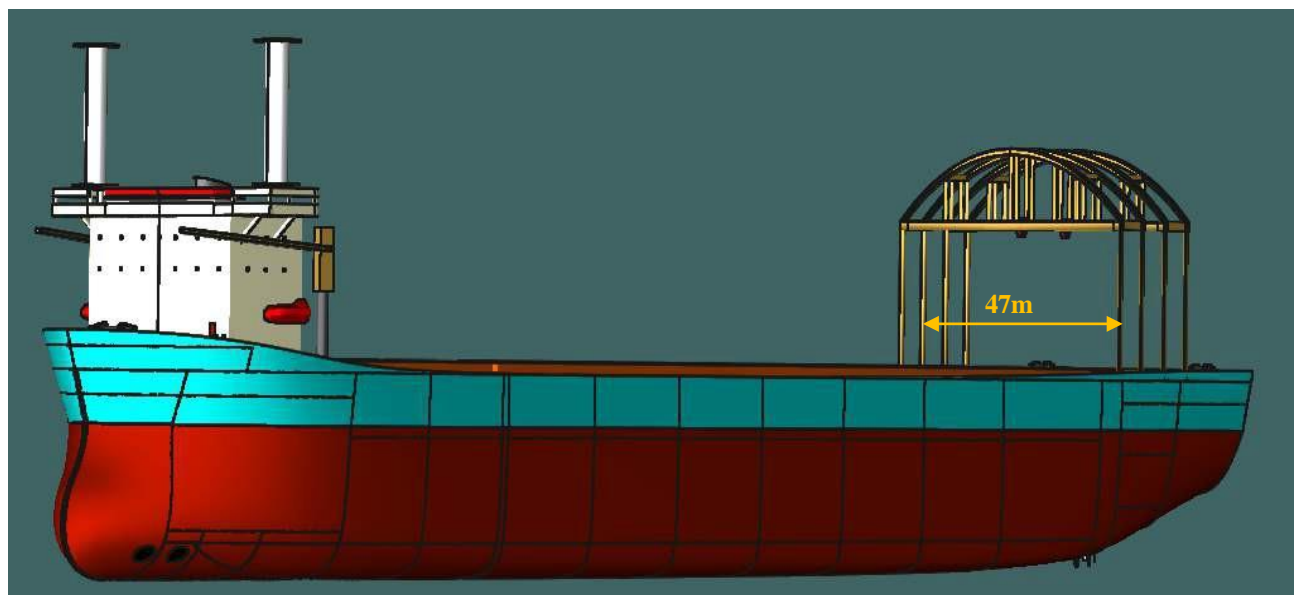
Figure 5-43 Dimension of Gantry Cranes
