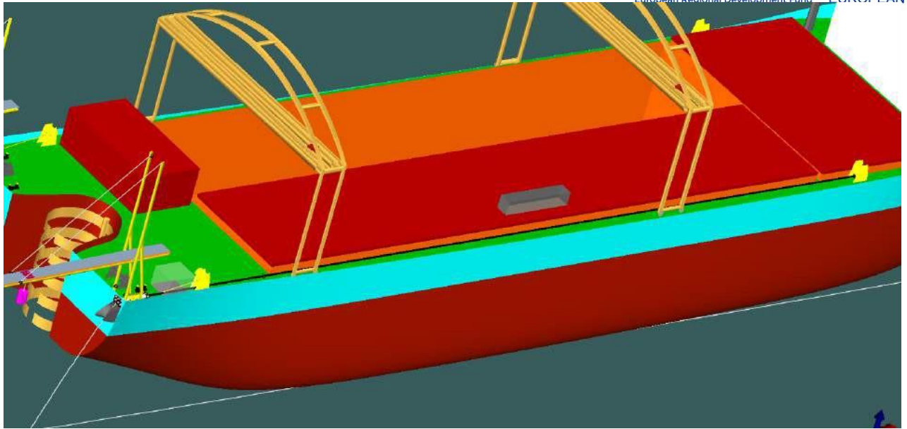
Figure 6-230 The Wire of second winch is released in order to take over the cable head from first winch
