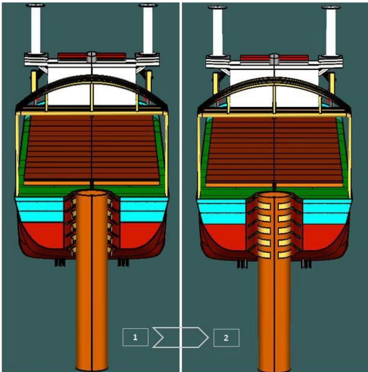
Figure 6-133 Decom Tools Vessel Positioned Around the Monopile
