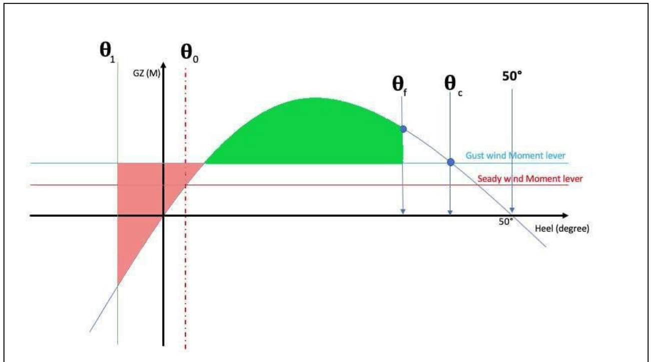
Figure 7-25 Sever Wind and Rolling GZ Curve
