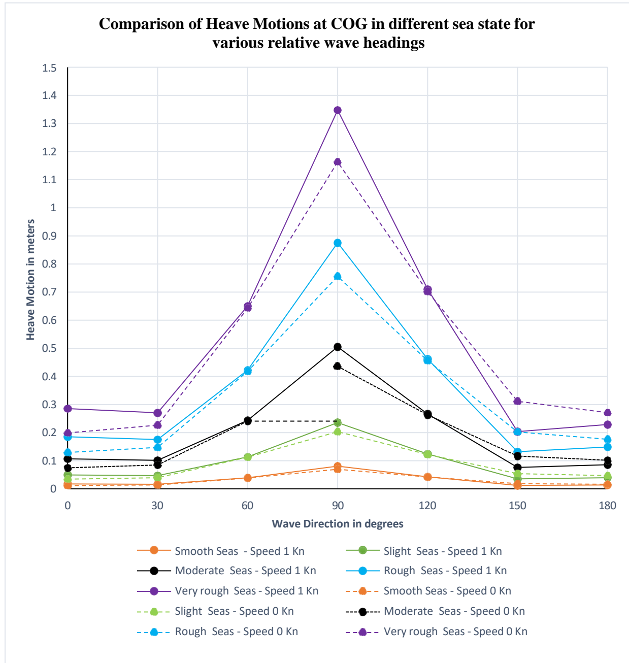
Figure 8-6 Comparison of Heave Motions at COG in different sea states
