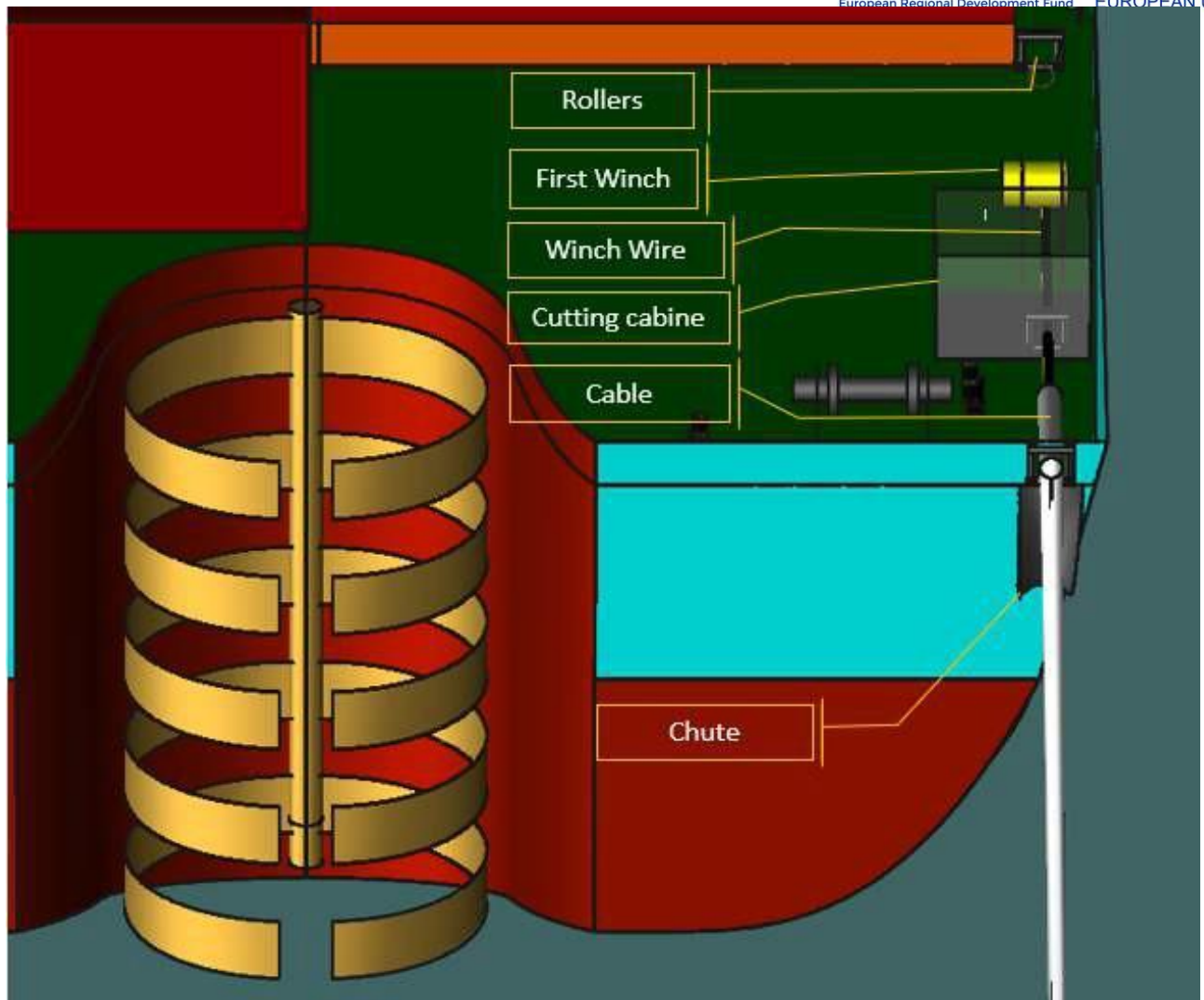
Figure 6-215 Chute, Hydraulic Cable Clamp and 1st Winch
