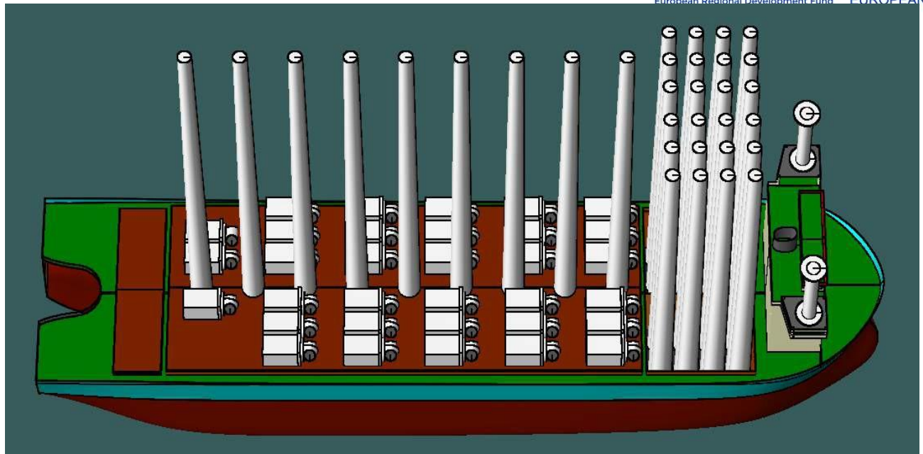
Figure 6-42 Top View of Load out of 3.6 MW Wind Turbine
