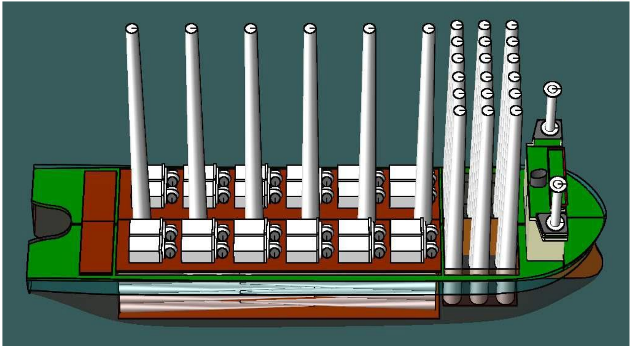
Figure 7-35 24 Sets of 5MW Wind Turbine are Loaded Out
