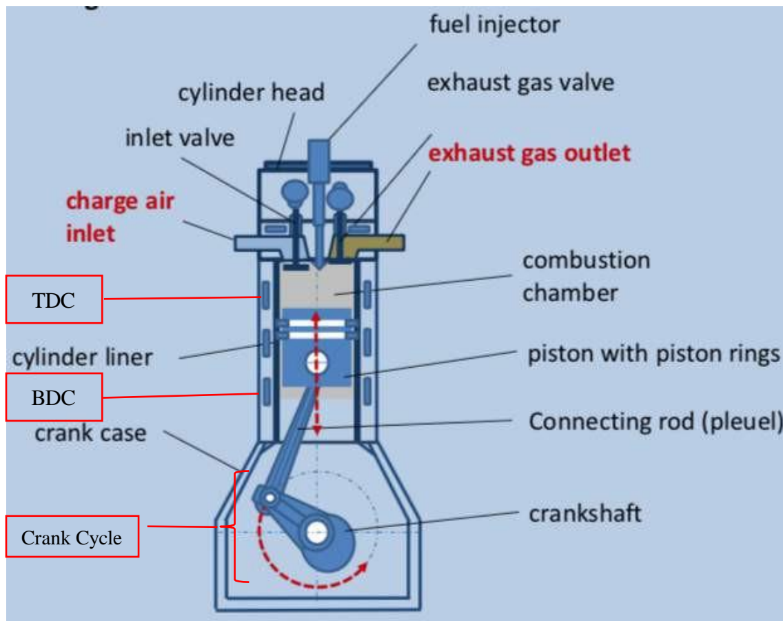
Figure 4-2 Cross Section of 4 Stroke Diesel Engine
