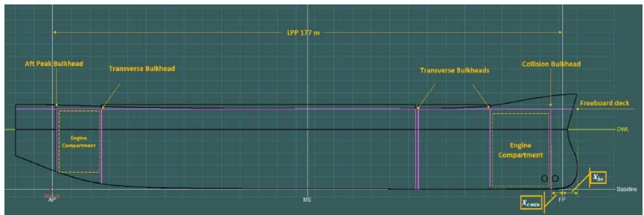
Figure 7-6 Watertight Hull and Subdivision of Decom Tools Vessel
