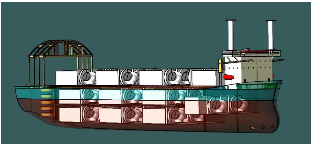
Figure 6-51 Perspective View of Load of 12MW Nacelle with Decom Tools Vessel
