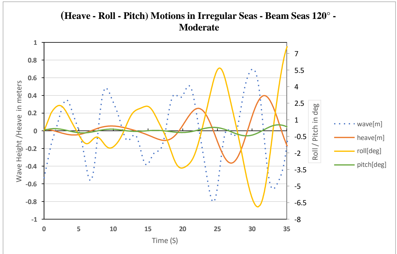
Figure 8-21 Motion in irregular beam seas 120° – Moderate
