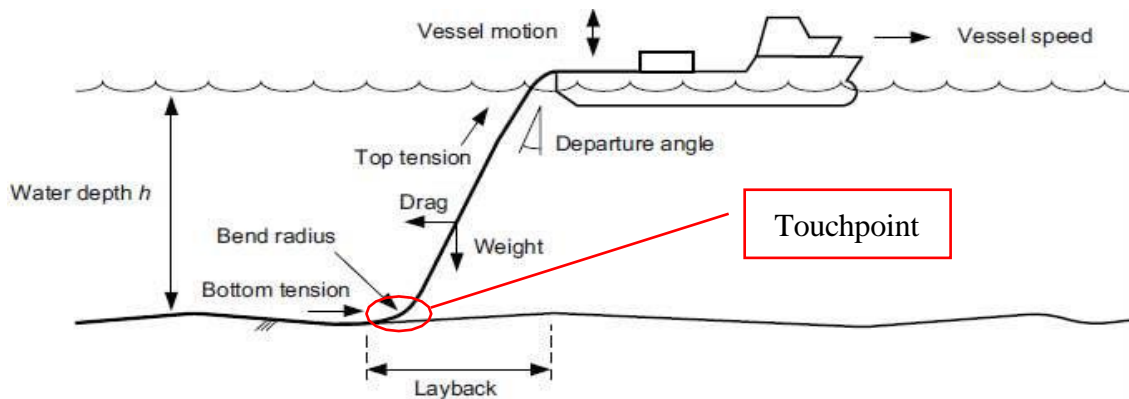
Figure 6-204 Cable Laying Process
