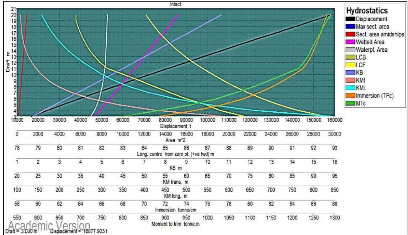
Figure 7-13 Hydrostatic Parameters of Decom Tools Vessel with respect to the draft
