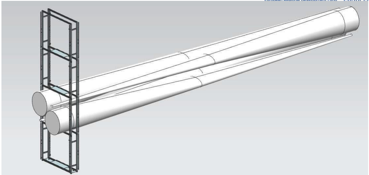
Figure 6-84 Securing 4 numbers of 3.6 MW blades inside the racks
