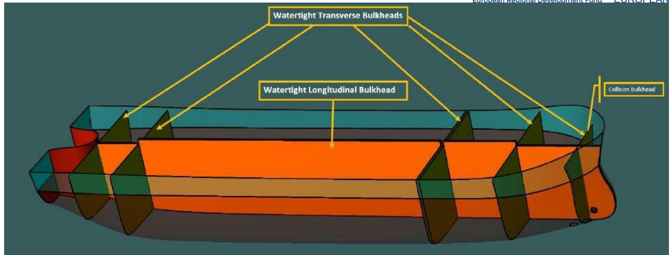
Figure 5-17 Longitudinal and Transverse Bulkhead of Decom Tools Vessel
