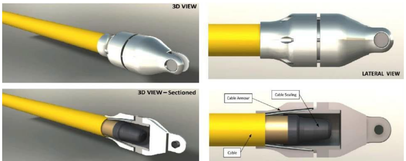
Figure 6-197 Submarine Power Cable Pulling Head (PCS Italiana n.d.)
