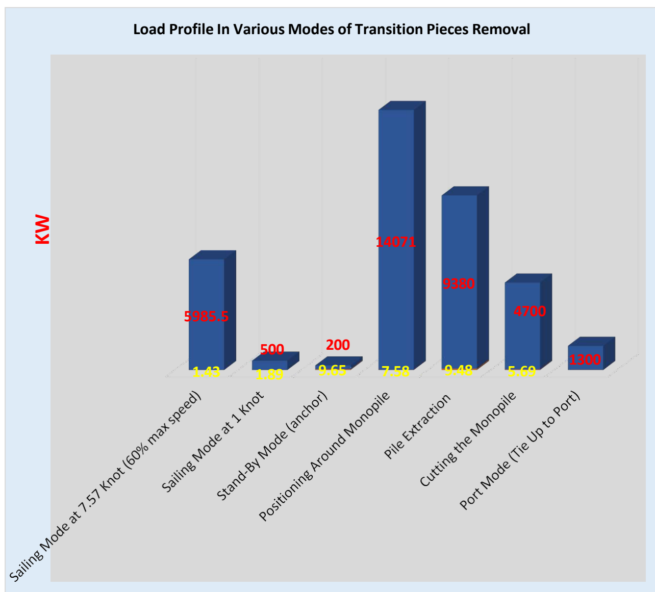
Figure 5-77 Load Profiles During Transition Piece Removal
