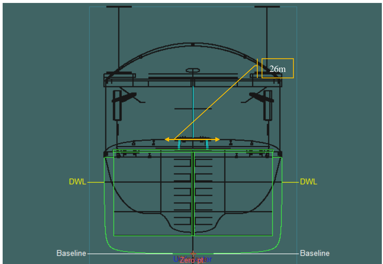
Figure 6-123 Location of Pile Extraction System
