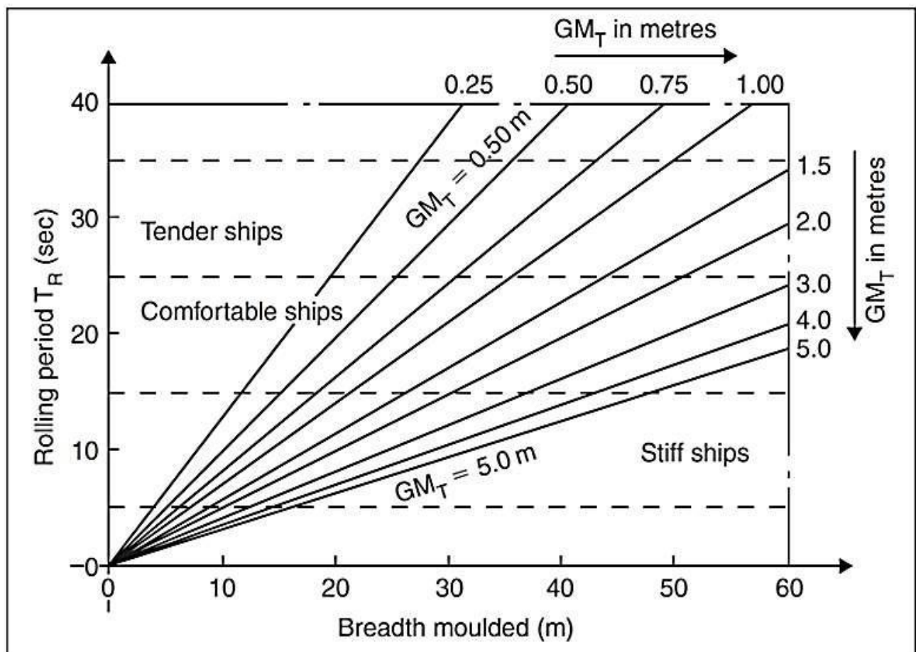
Figure 7-28 Relation Between Rolling Period and GM
