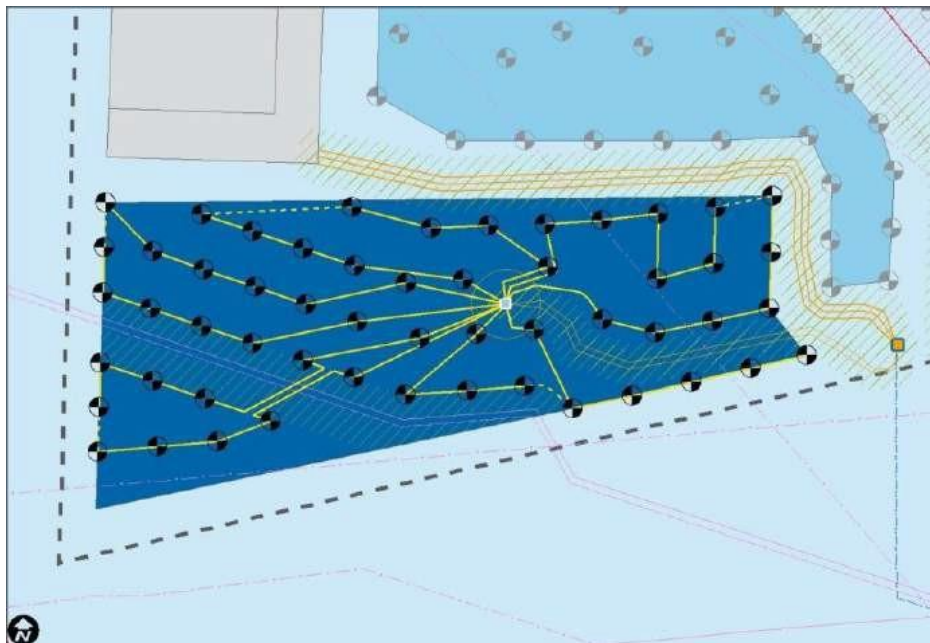
Figure 6-176 Topology of Nordsee 1 wind farm
