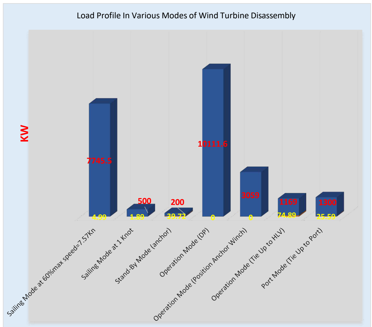
Figure 5-75 Load Profiles During Disassembly of Wind Turbines
