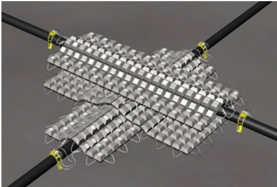
Figure 6-182 Mattress installed on the cables as means of protection
