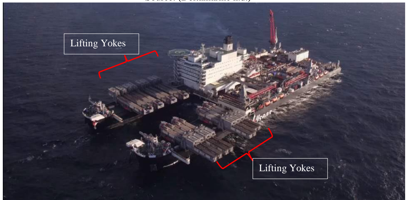
Figure 6-126 Lifting Yokes
