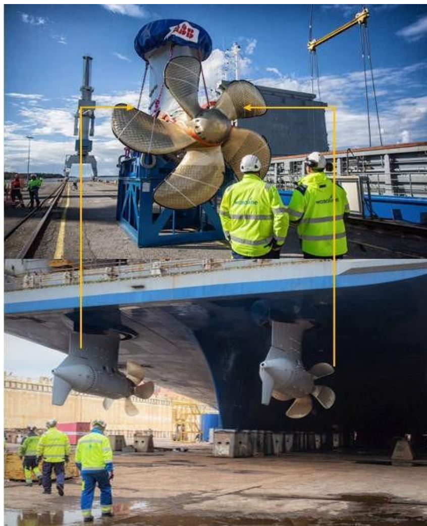
Figure 4-15 ABB Azipod Propeller Installed on a Ferry
