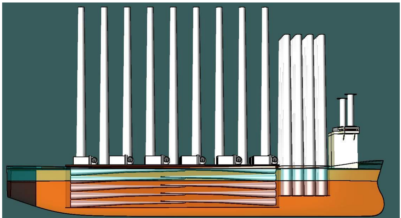
Figure 6-43 Side View of Load out of 3.6 MW Wind Turbine
