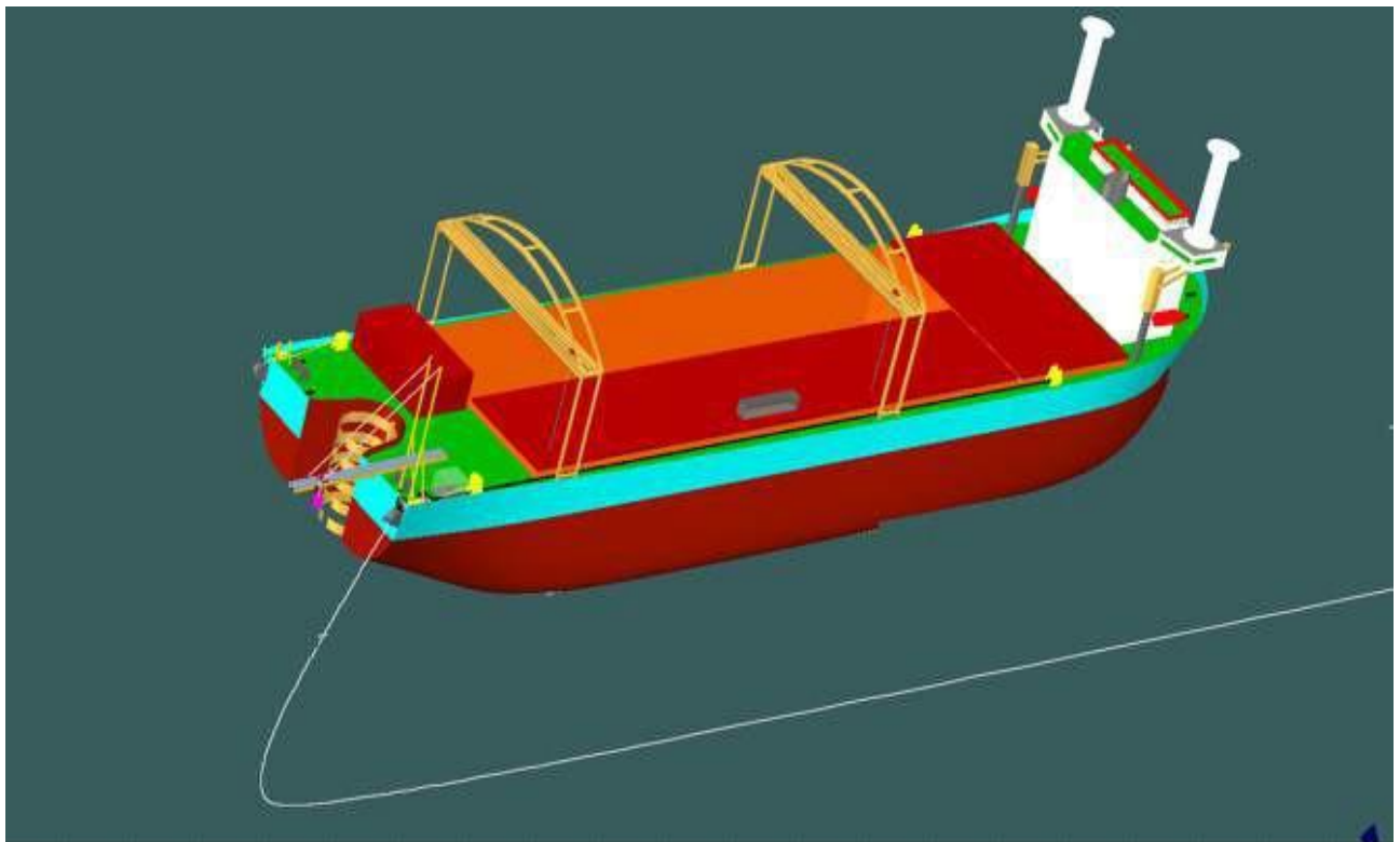
Figure 6-229 The Wire of second winch is released in order to take over the cable head from first winch
