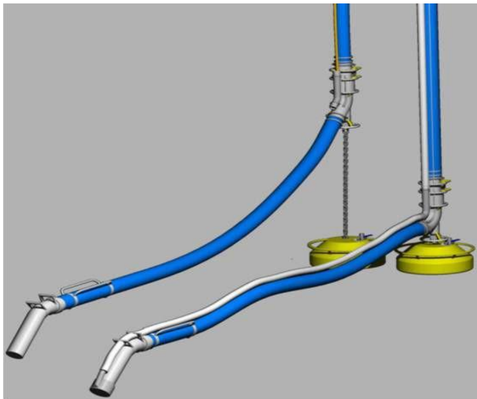
Figure 6-190 Common Type of Airlift (inzenjering n.d.)
