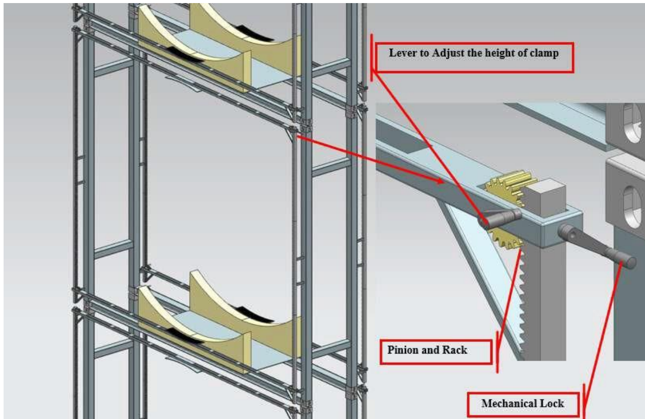
Figure 6-70 Blade Securing System
