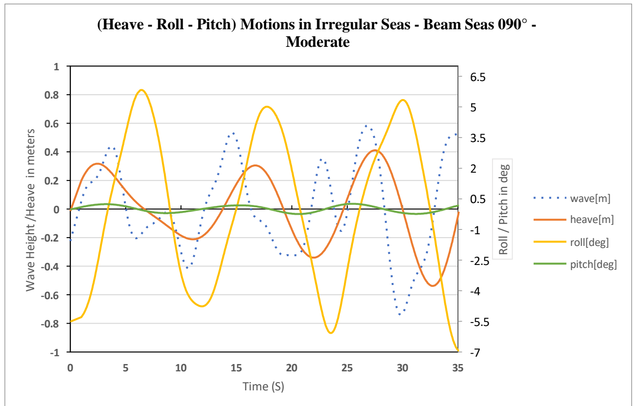
Figure 8-22 Motion in irregular beam seas 090° – Moderate
