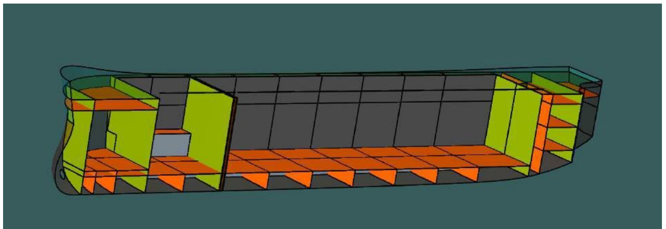
Figure 5-26 Cross Section of Double Bottom, (top)side Tanks
