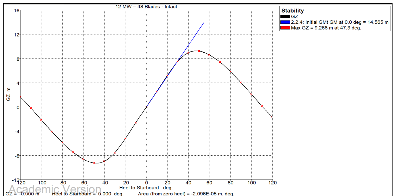
Figure 7-34 GZ Curve after Loading 48 numbers of 12MW Blades
