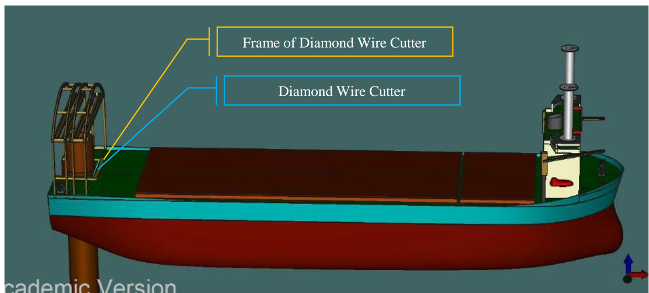
Figure 6-147 Cutting of Extracted monopile has been completed by Diamond wire cutter
