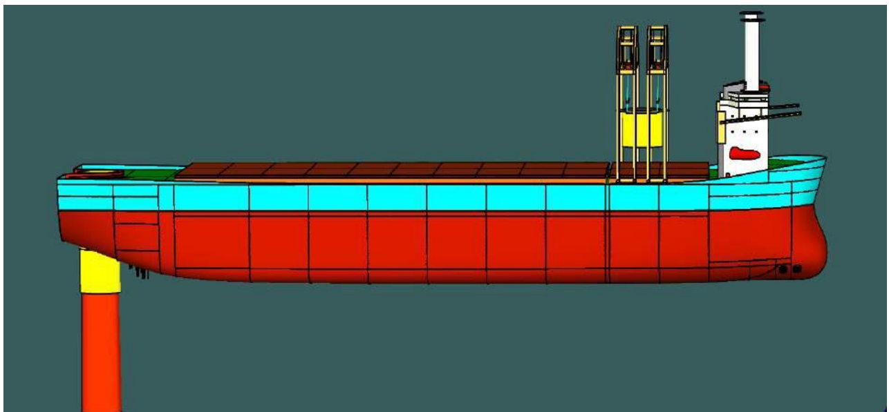
Figure 6-107 Loading of cut section of TPs (Side View)
