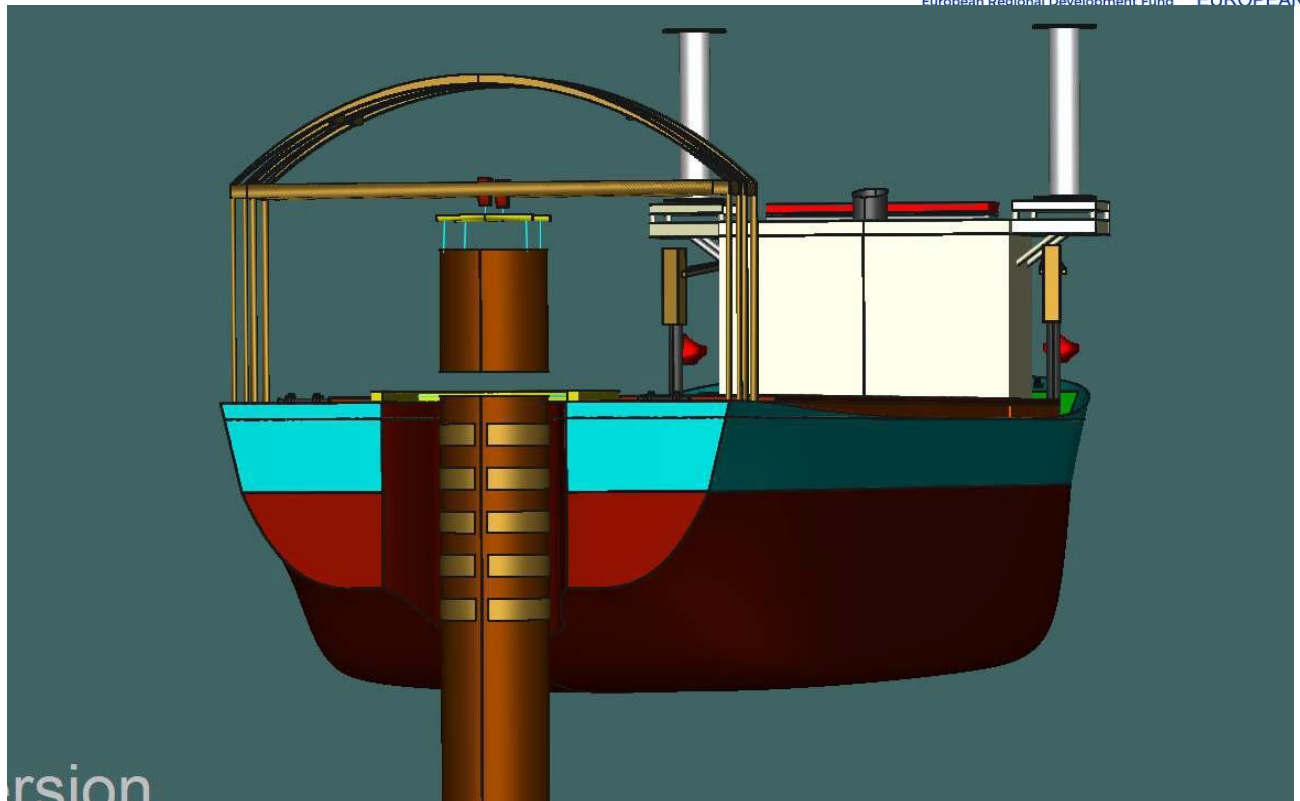
Figure 6-151 Lifting and Transferring the Cut section of Monopile (Perspective view)
