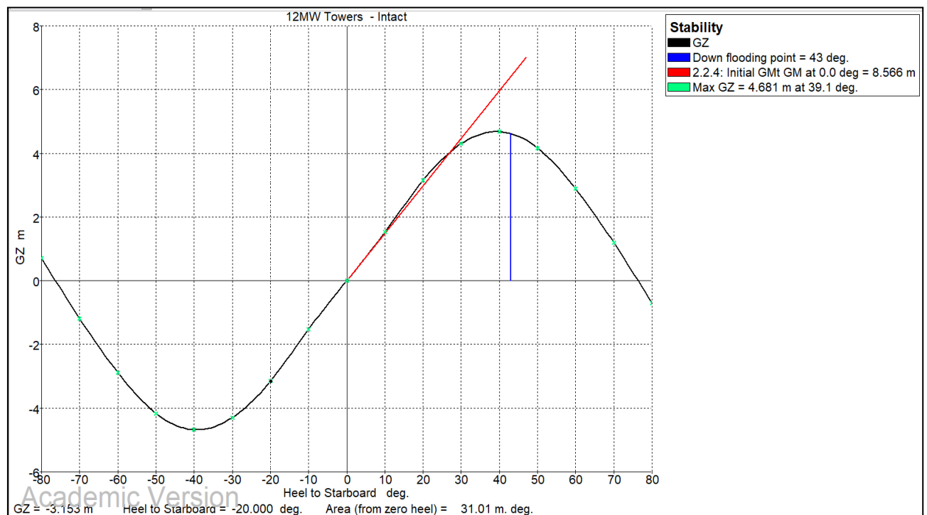
Figure 7-30 GZ Curve after Loading 24 Sets of 12MW Tower
