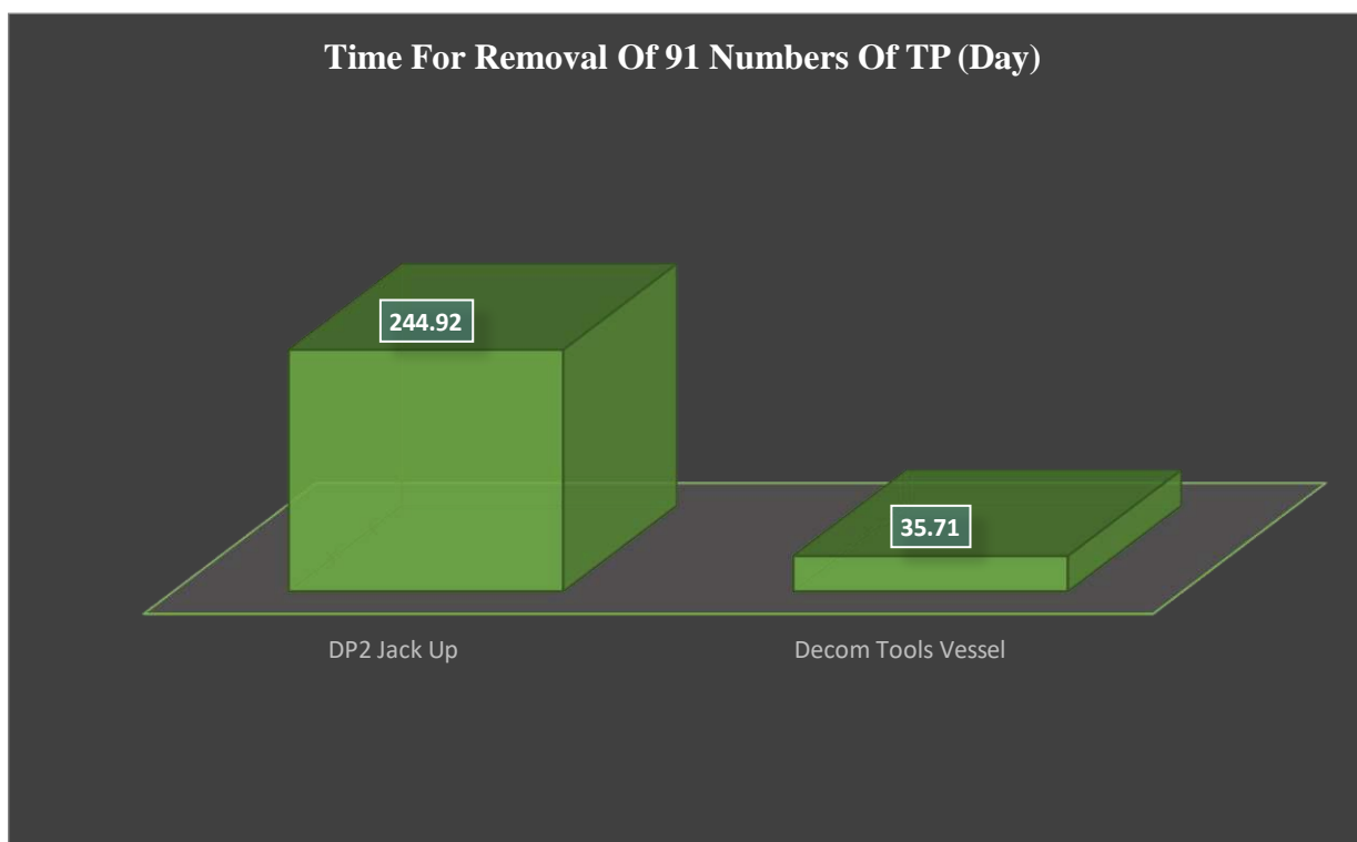
Figure 6-112 Duration for Removal of 91 Numbers of TP
