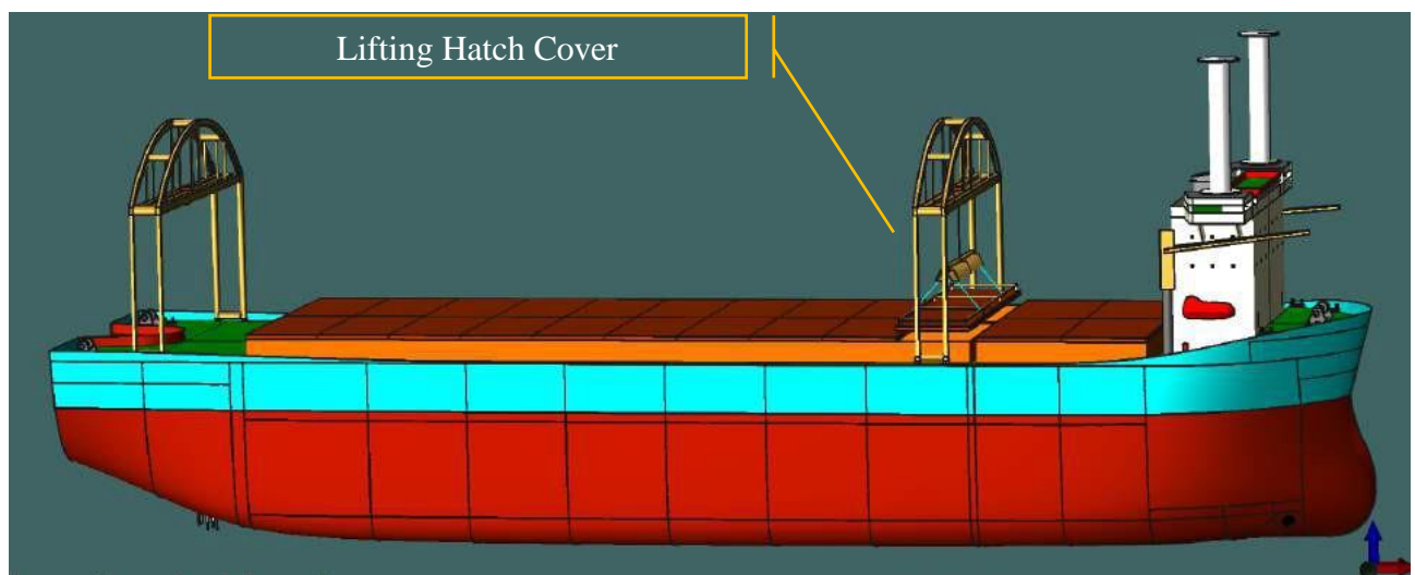
Figure 5-94 Procedure to open the Hatch Cover-Step 2 Lifting Hatch Cover
