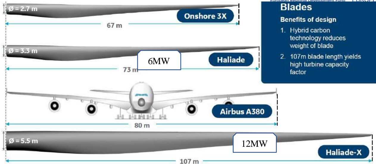
Figure 6-5 Dimension of blades of Various Wind Turbine sizes (LM Windpower 2020)
