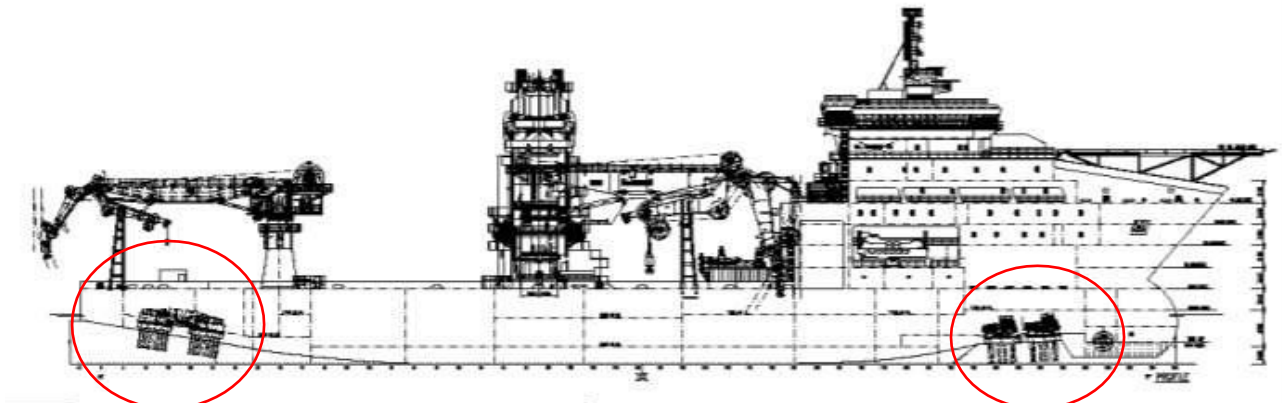
Figure 4-22 Arrangement of Voith Schneider Propeller on North Sea Giant
