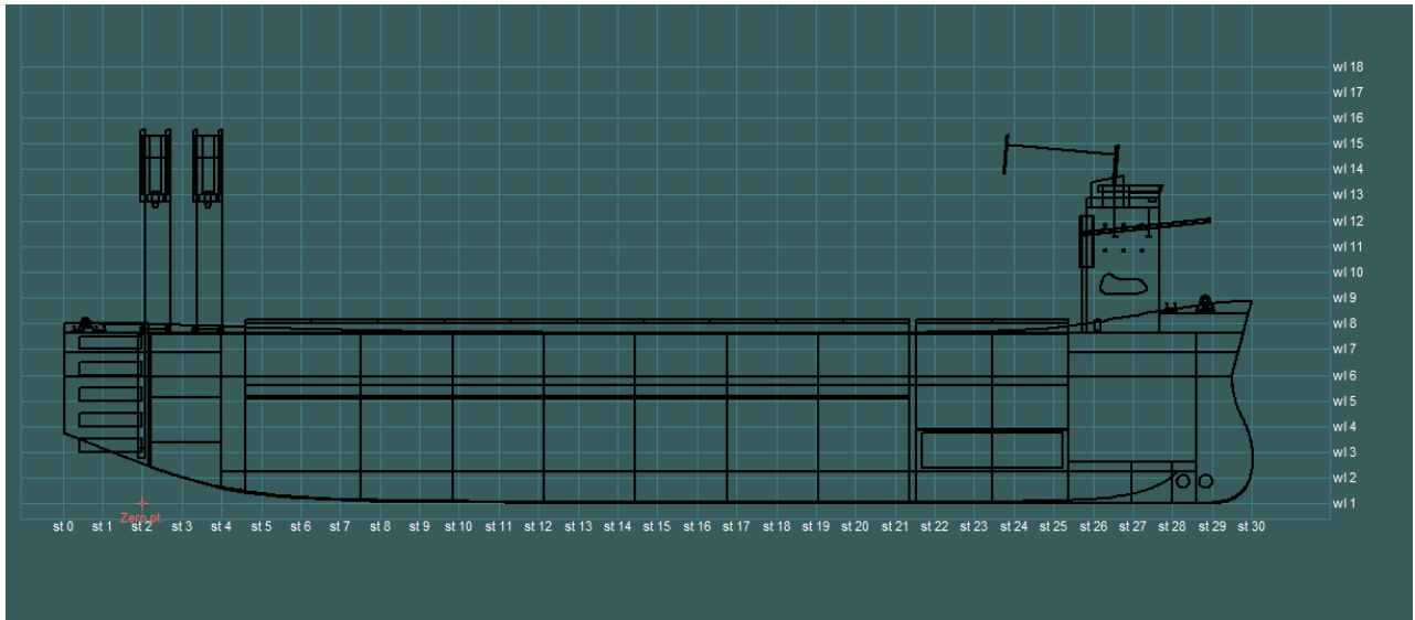
Figure 5-52 Foldable Flettner Rotor
