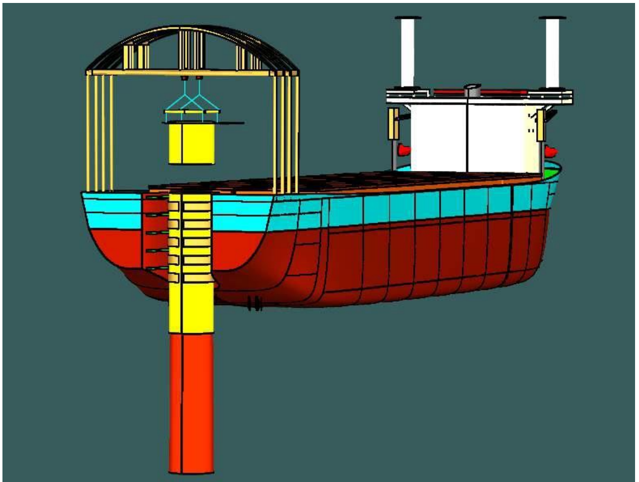
Figure 6-101 The top section of TP is cut
