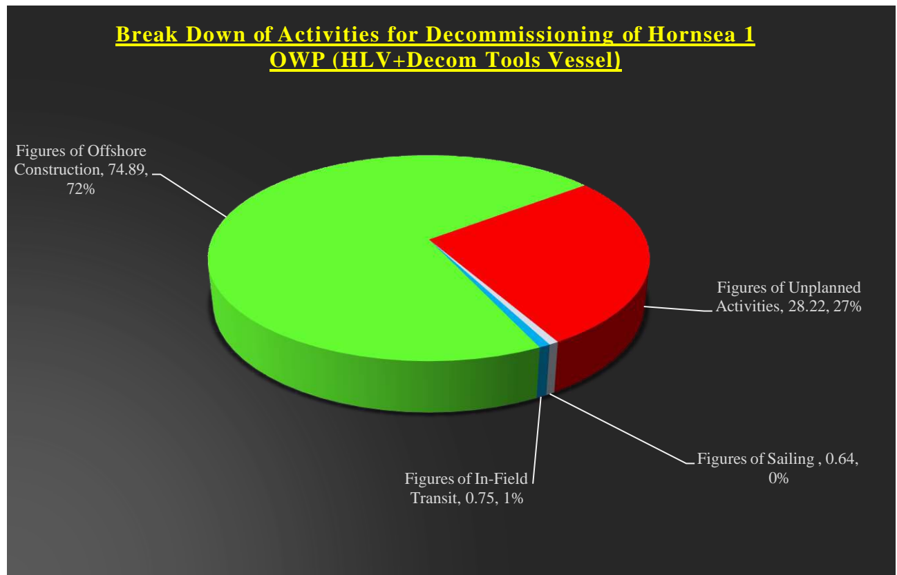
Figure 3-42 Break Down of Hornsea 1 offshore Wind Farm Decommissioning with a HVL + Decom Tools Vessel
