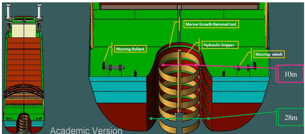
Figure 5-87 Details of Stern of the Decom Tools Vessel (Pile Gripper and MGR System)
