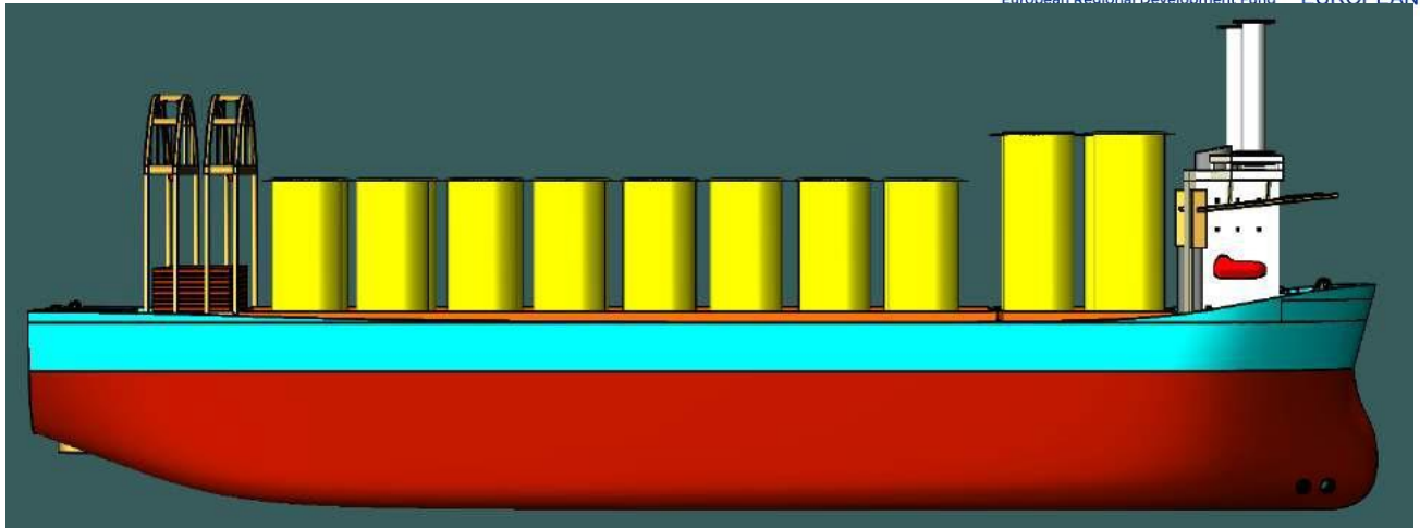
Figure 6-46 Side View of Load of 12MW TP with Decom Tools Vessel
