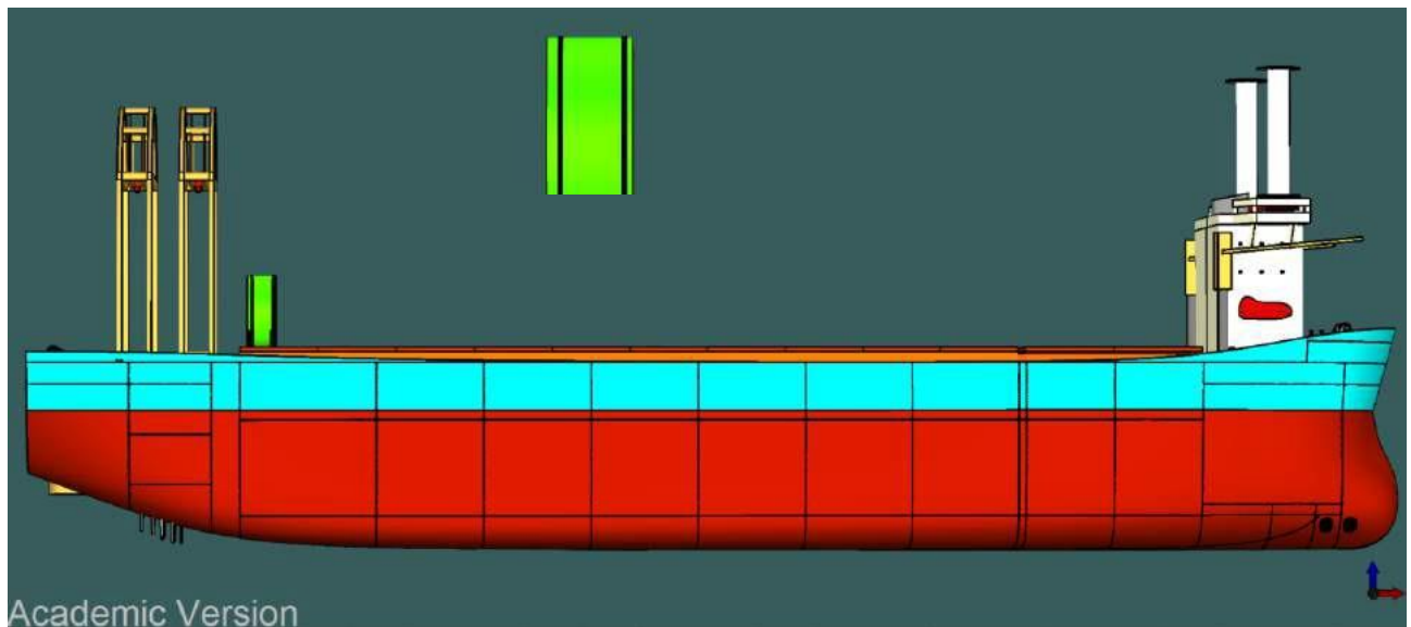
Figure 6-170 Seafastening of MP & TP After Cutting & MGR (Side View)
