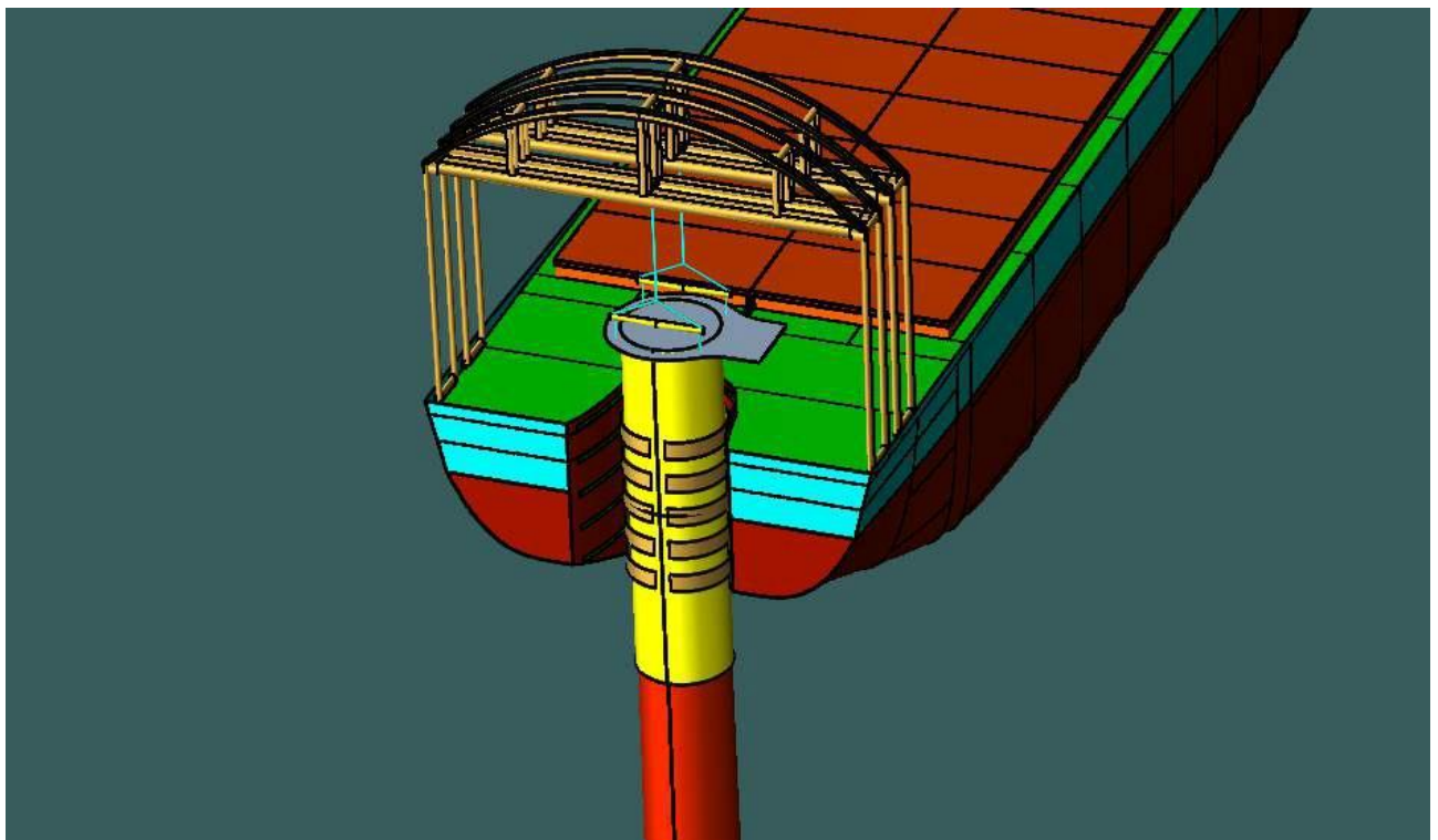
Figure 6-99 The Transition piece is hold by the Grippers & connected with slings to the Gantry Cranes
