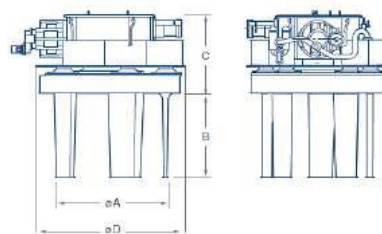
Figure 5-66 Data Sheet of Voith Schneider Propulsion System
