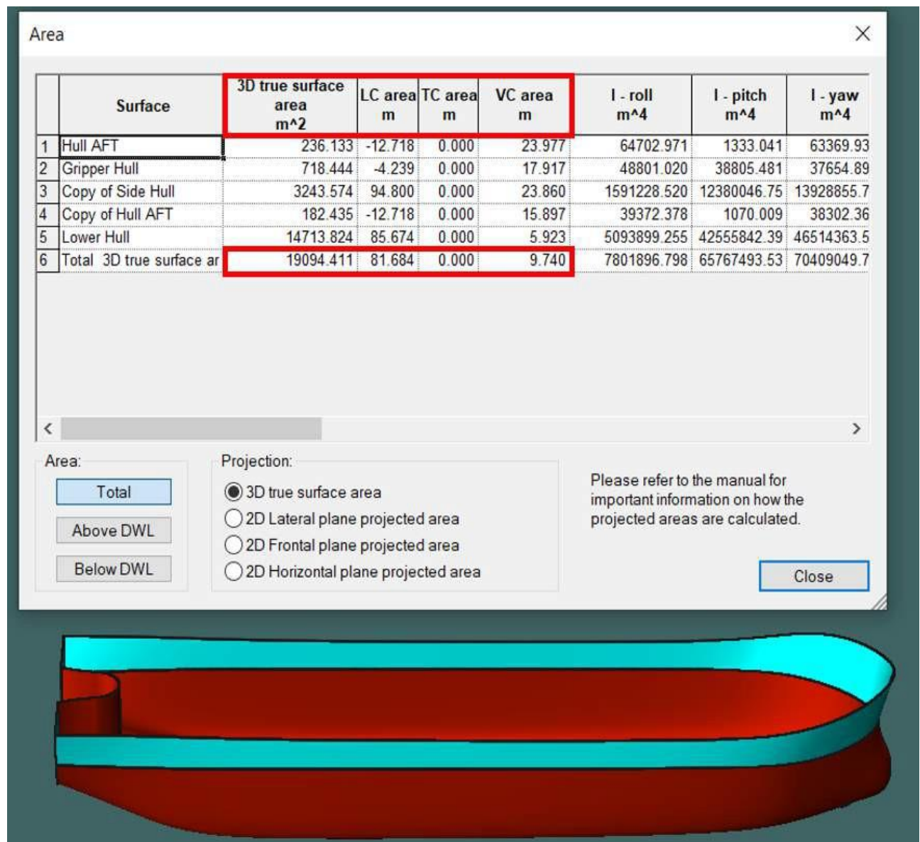
Figure 7-5 Calculating the Surface of Decom Tools Hull
