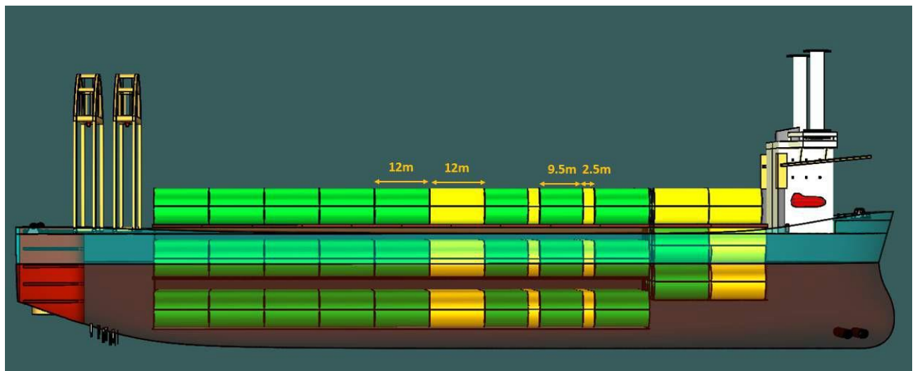
Figure 6-164 Load out of 44 Numbers of MP plus TP (side View)
