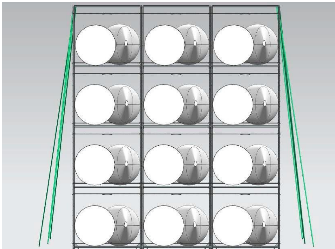
Figure 6-80 Front View of Loading 5MW blades inside the racks
