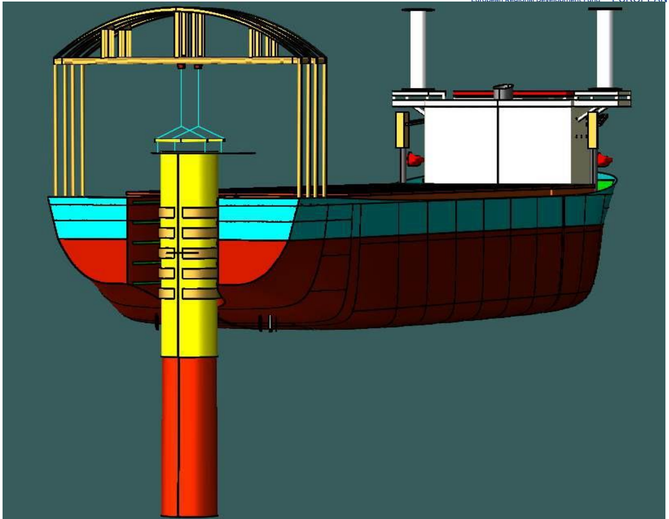
Figure 6-98 Transition Piece are positioned inside the grippers (perspective view)
