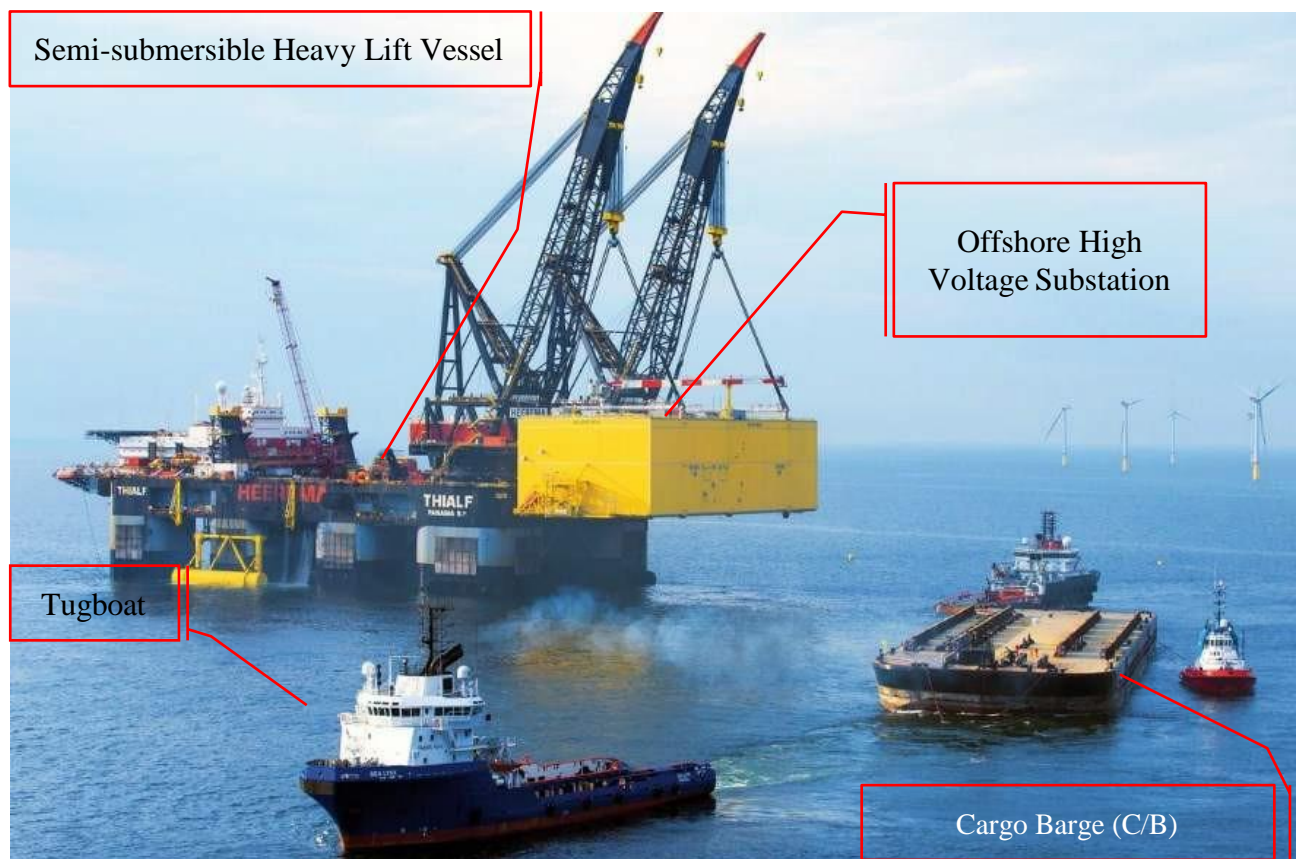
Figure 3-27 Installation of Topside of OHVS
