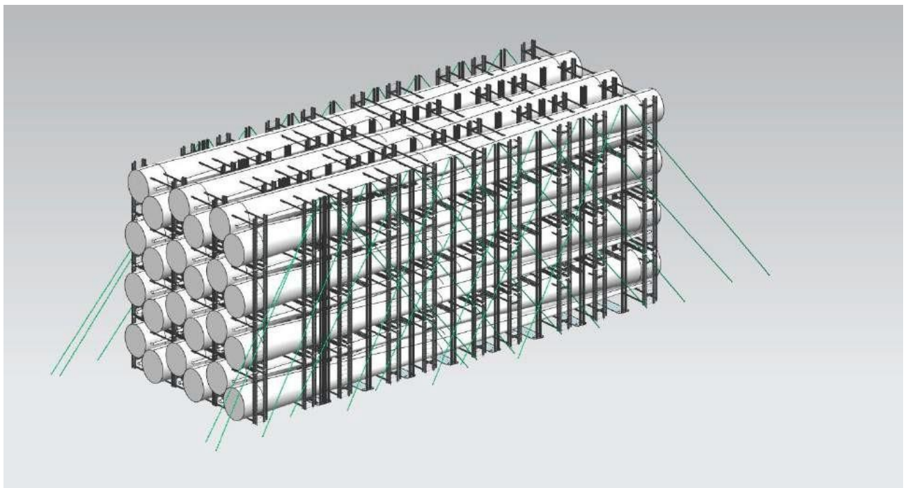
Figure 6-82 Optimum Arrangement of Rack and Cutting Tools for 3.6 MW blades
