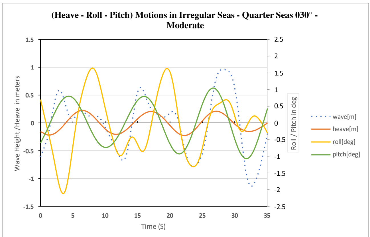
Figure 8-24 Motion in irregular following seas 030^\circ – Moderate
