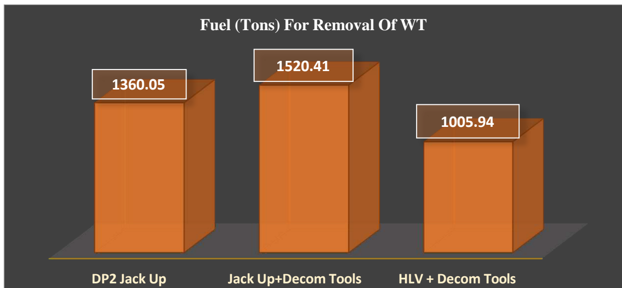
Figure 3-38 Fuel Consumption of Various Logistic Configuration in Decommissioning of Noblewind OWP
