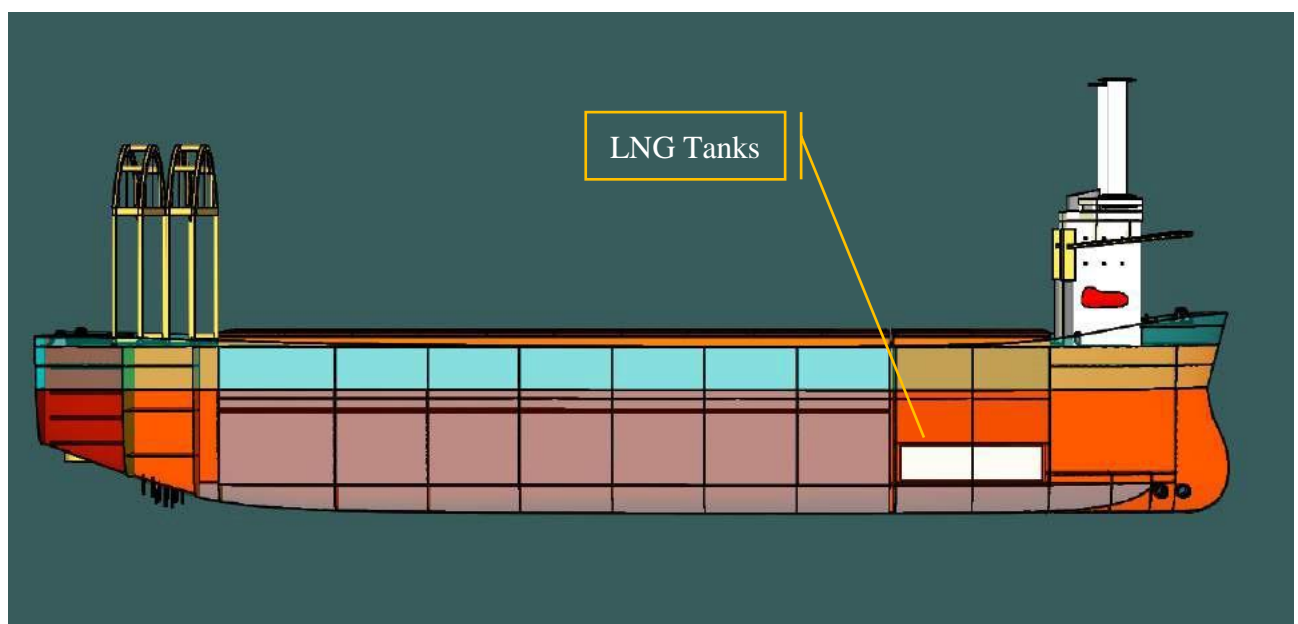
Figure 5-31 Location of LNG tanks of Decom Tools Vessel
