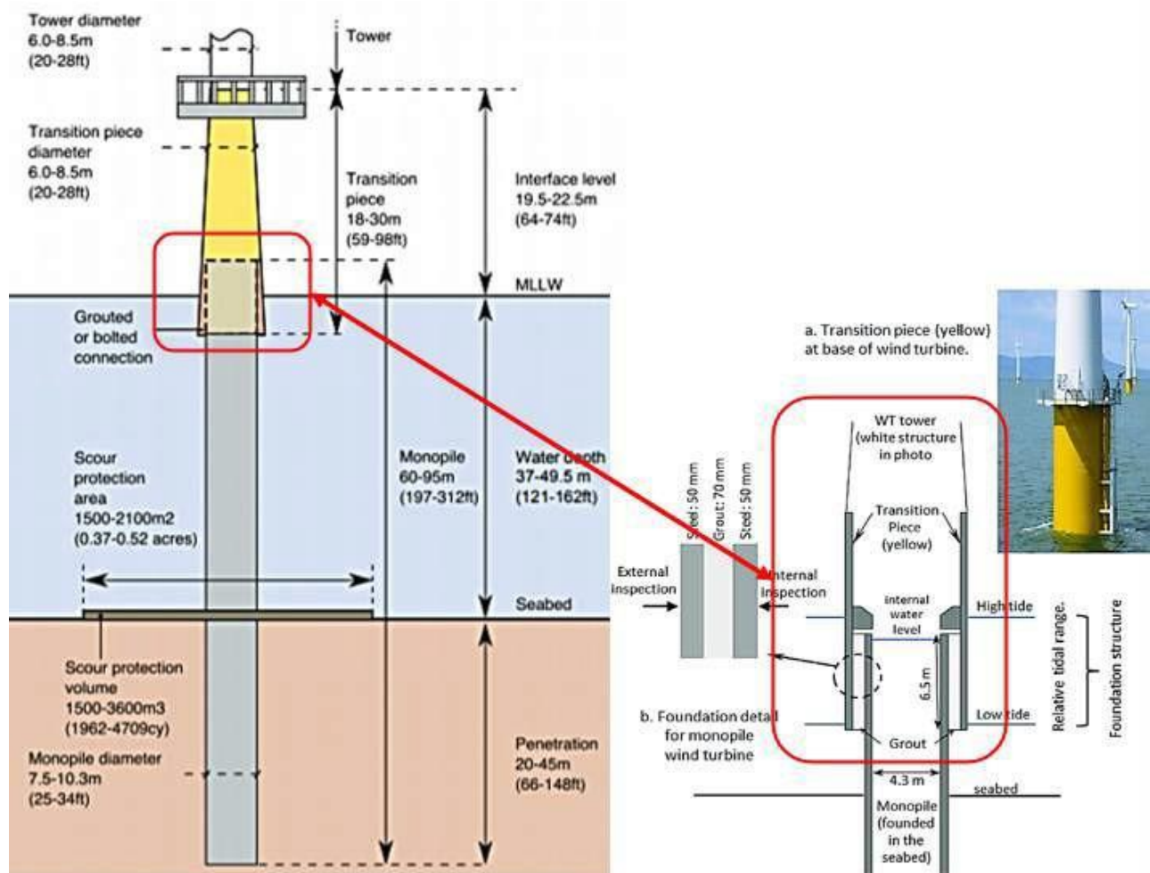
Figure 6-87 Detail of Installation of TP & MP
