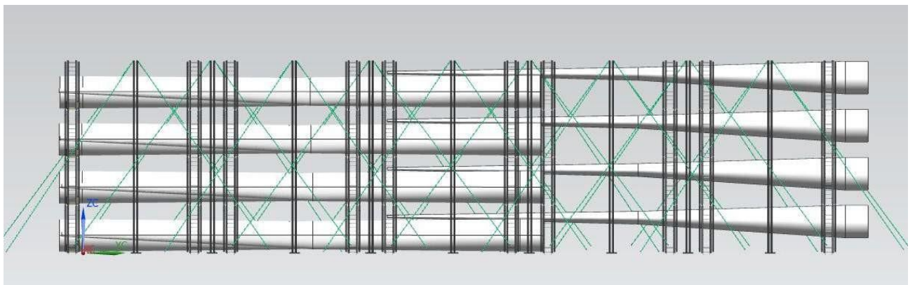
Figure 6-79 Optimum Load out of 5MW Blades
