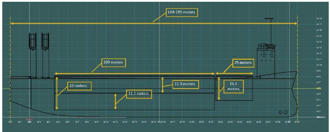
Figure 6-20 Dimension of Decom Tools Vessel
