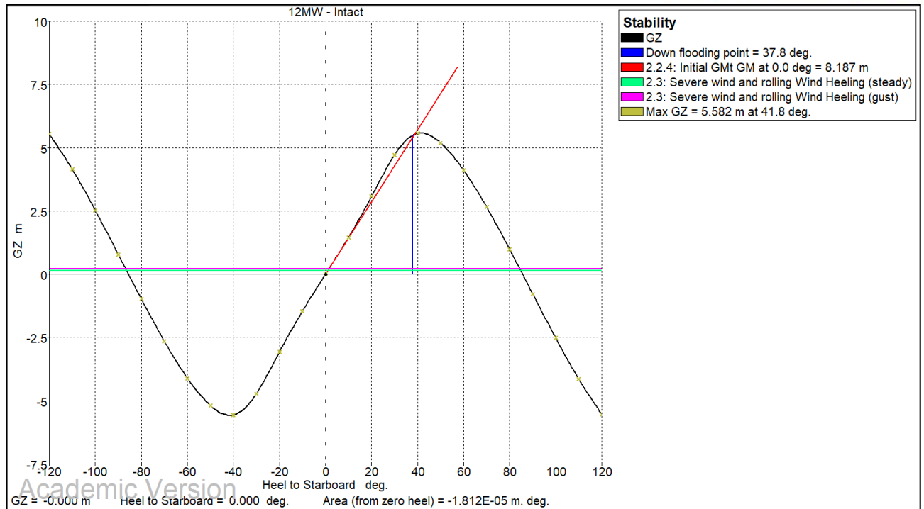
Figure 7-27 Decom Tools Vessel GZ Curve after Loading 8 x 12MW WT
