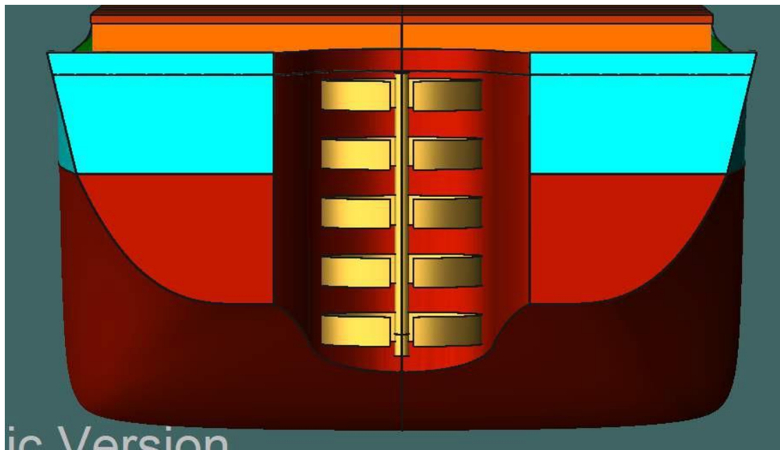
Figure 6-120 Extraction Grippers
