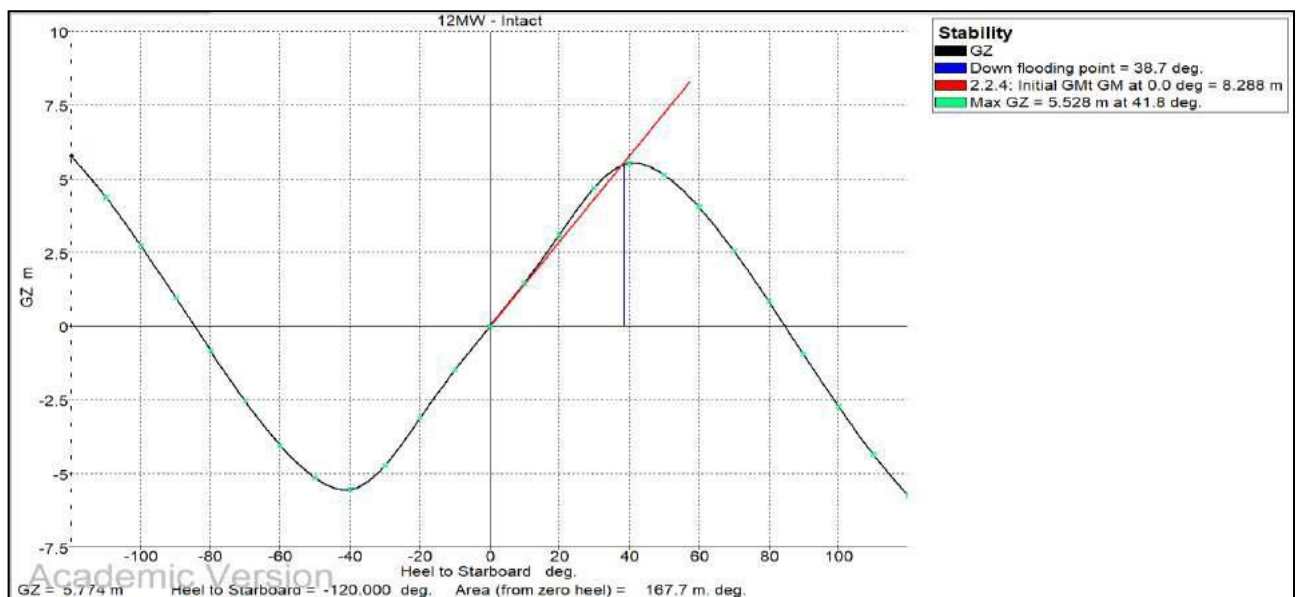
Figure 7-24 GZ Curve Arrival Condition While Loading 8x12MW WT
