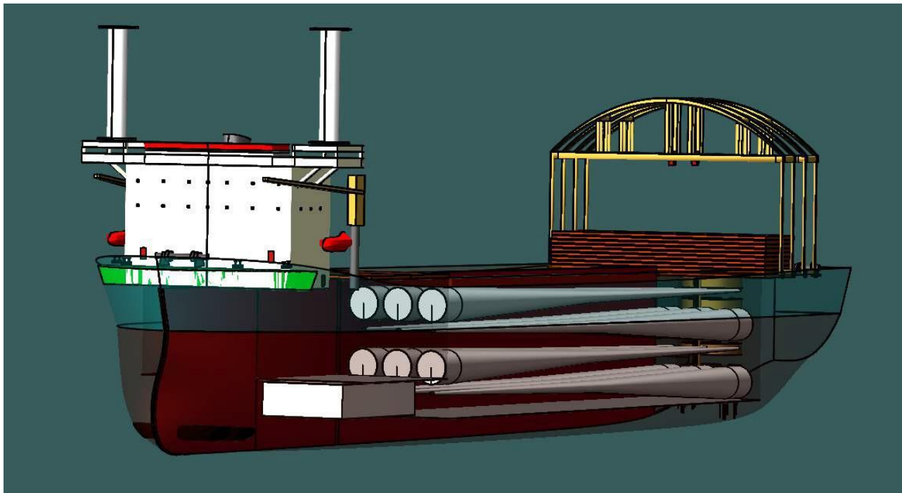
Figure 6-23 Perspective view of Load out of 12 MW Blades inside the holds
